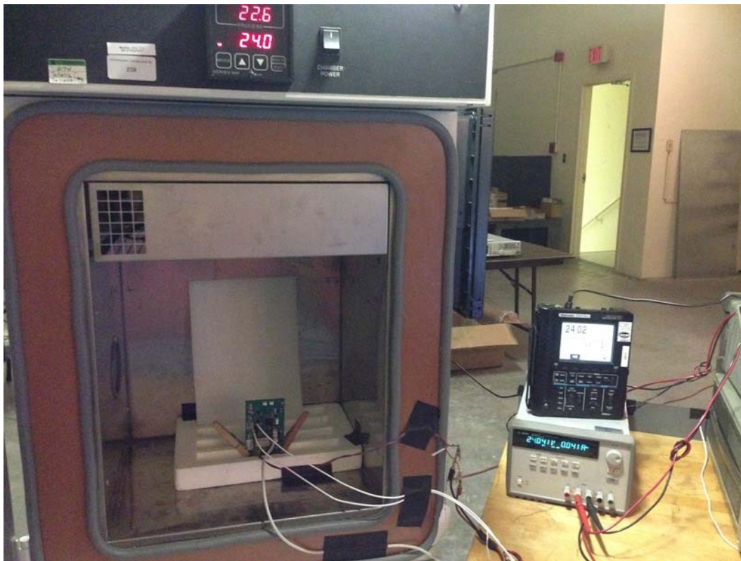
Frequency Stability 1
