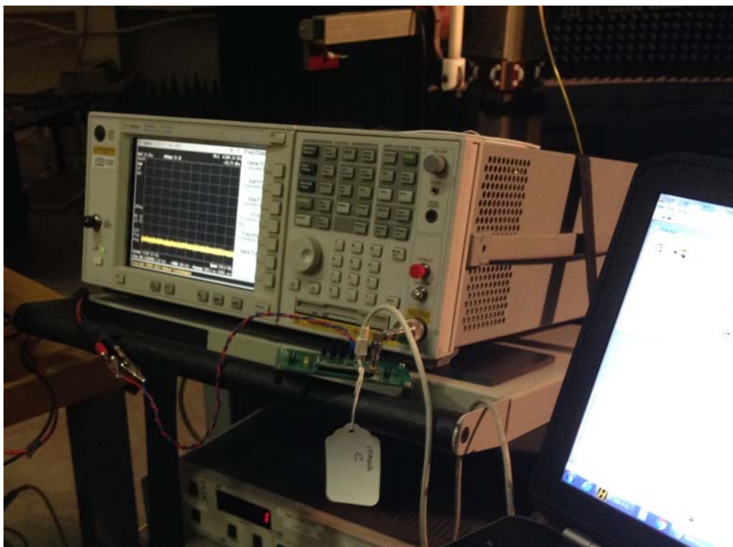
Conducted Antenna Port: Bandwidth, Power, Spurious, Mask
