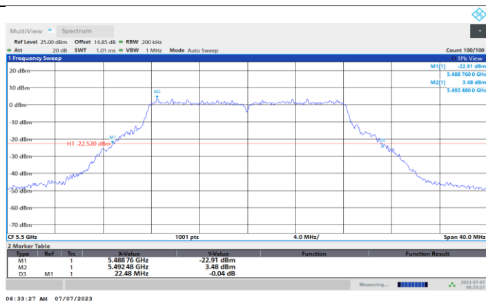
11A-CDD_Ant4_5500
