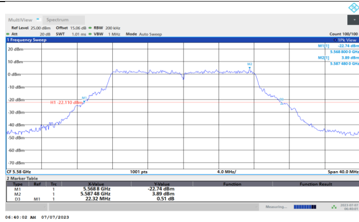
11A-CDD_Ant3_5580
