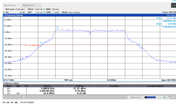
11A-CDD_Ant4_5700
