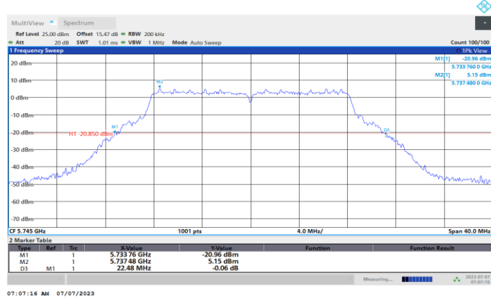
11A-CDD_Ant4_5745
