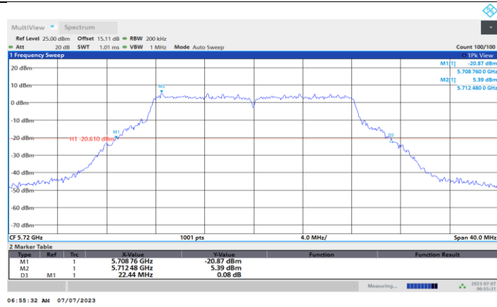
11A-CDD_Ant4_5720
