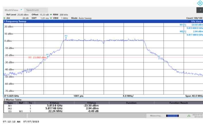
11A-CDD_Ant3_5825
