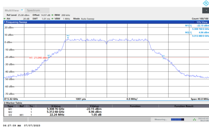
11A-CDD_Ant4_5320
