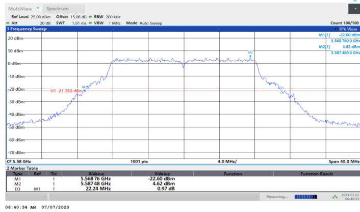
11A-CDD_Ant4_5580
