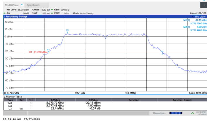
11A-CDD_Ant4_5785
