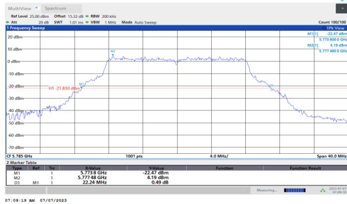
11A-CDD_Ant3_5785
