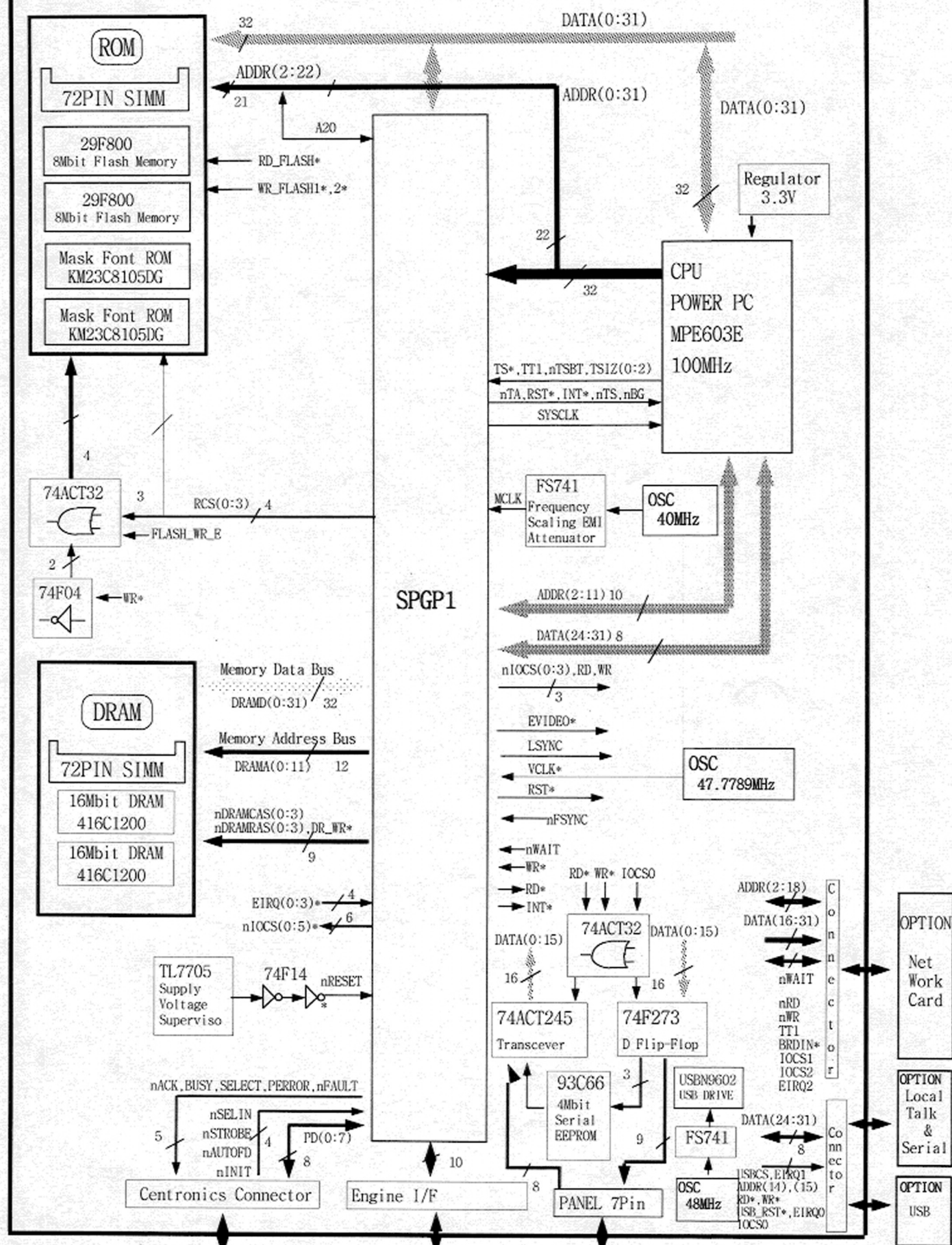
Video Controller Board Block Diagram
