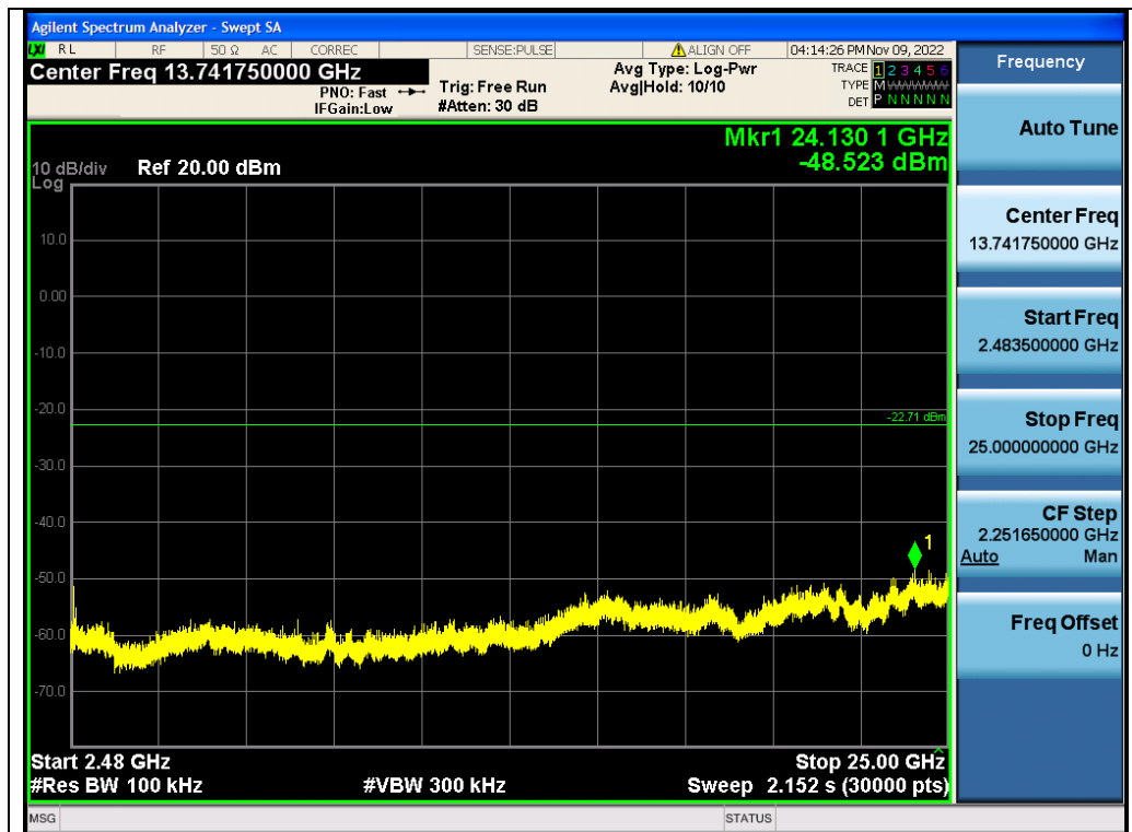
Test_Graph_2.4G_ANT2_2440_1Mbps_Higher Band Emissions
