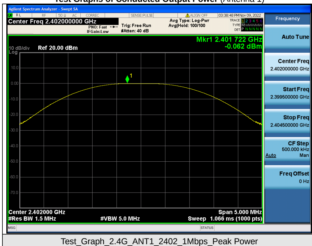
Test Graphs of Conducted Output Power (Antenna 1)
