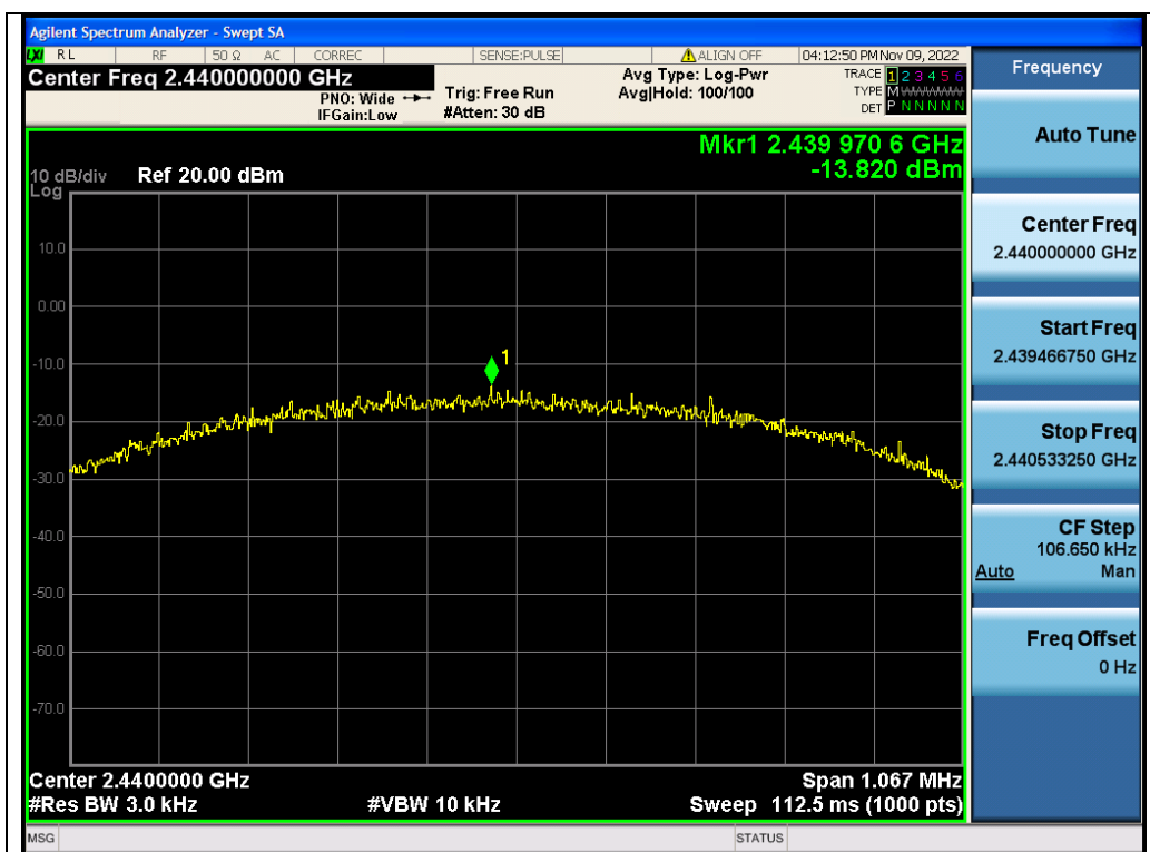
Test_Graph_2.4G_ANT2_2440_1Mbps_PSD
