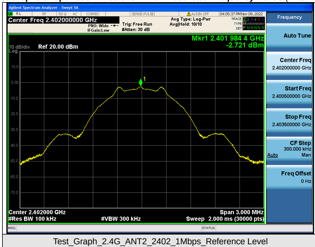
Test Graphs of Spurious Emissions in Non-Restricted Frequency Bands (Antenna 2)
