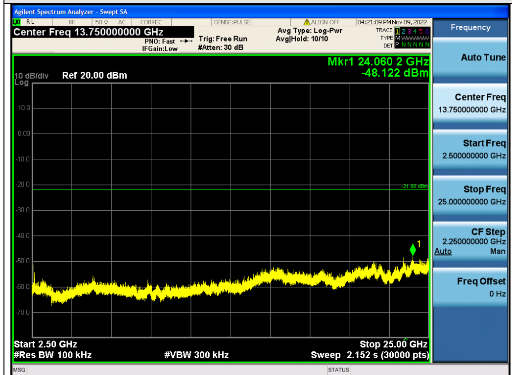
Test_Graph_2.4G_ANT2_2480_1Mbps_Higher Band Emissions
