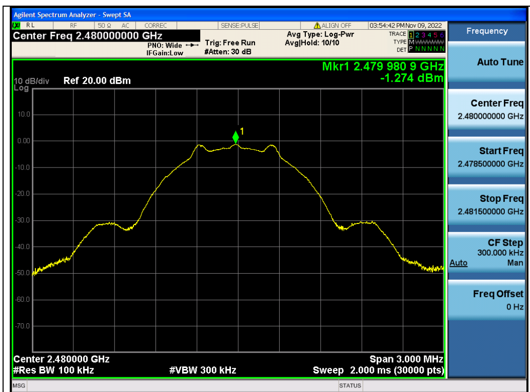
Test_Graph_2.4G_ANT1_2480_1Mbps_Reference Level
