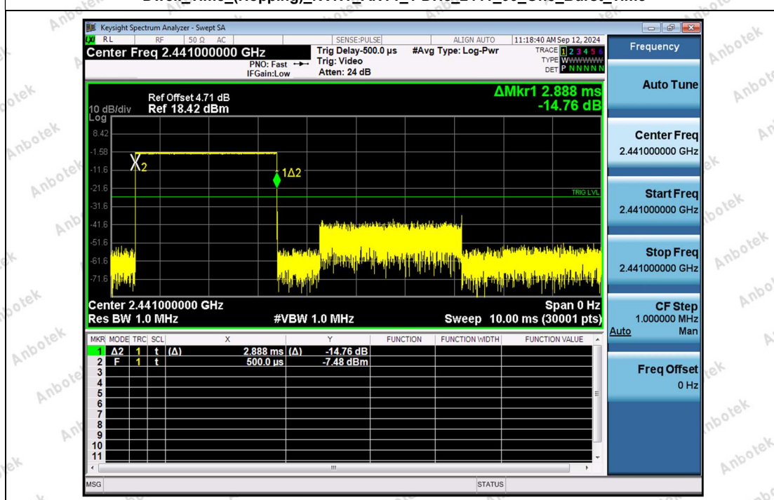
Dwell_Time_(Hopping)_NVNT_ANT1_1-DH5_2441_00_One_Burst_Time
