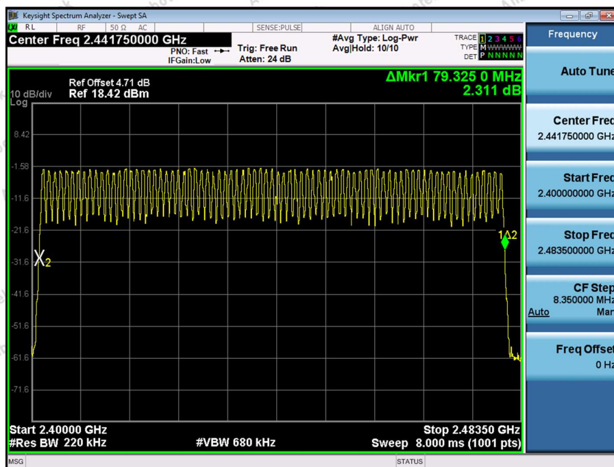
Number_of_Hopping_Channel_(Hopping)_NVNT_ANT1_1-DH5_Hopping
