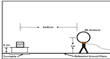
Figure 1. Below 30MHz
