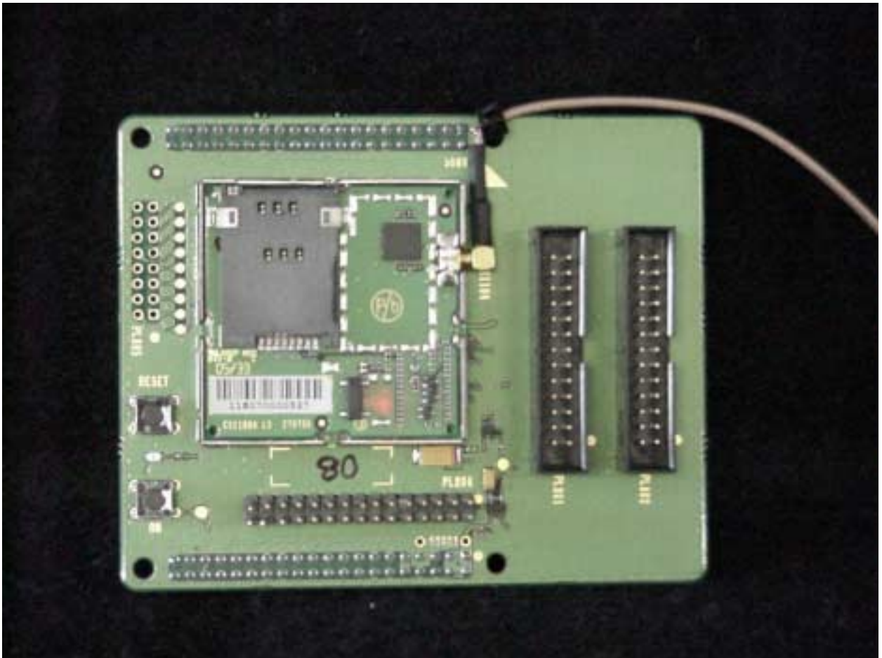
Photo 1. Top of EUT with shield removed
