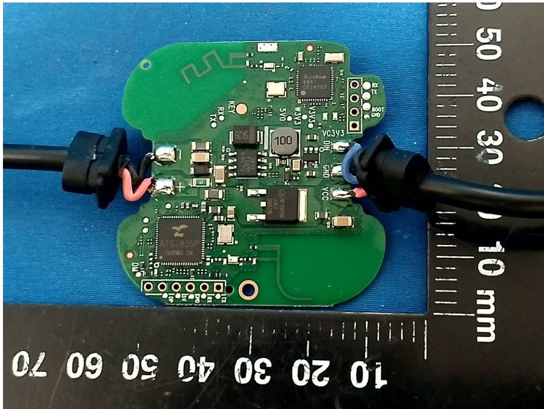
WiFi Chip+Antenna
