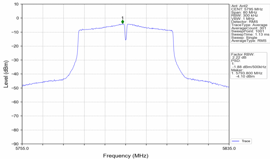
802.11ac(VHT40)_HCH_5795MHz_MIMO_NTNV
