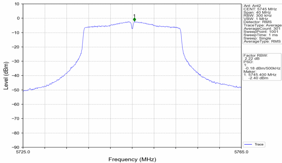
802.11ac(VHT20)_LCH_5745MHz_MIMO_NTNV
