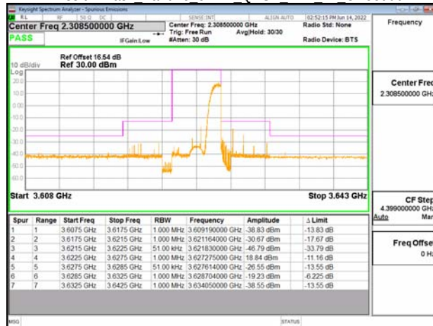
Emission Mask Band48 5MHz QPSK RB1 24 CH56715
