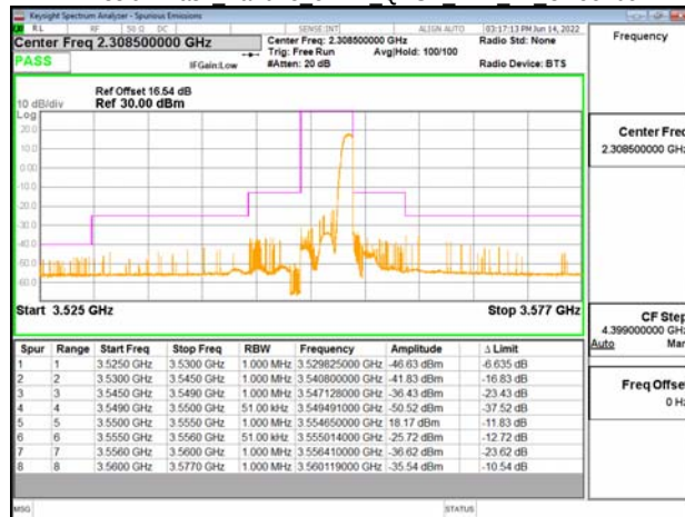
Emission Mask Band48 5MHz QPSK RB1 24 CH55990
