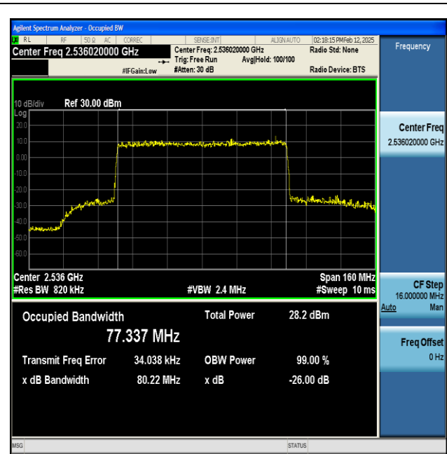
NTNV-n41-PC2-30-80-L-CP-256QAM-Outer_Full-Ant1-1 PASS
