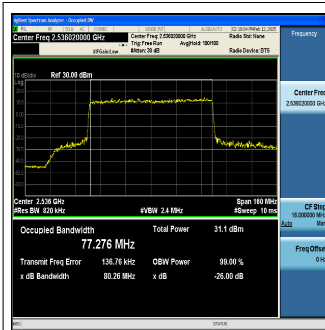
NTNV-n41-PC2-30-80-L-CP-64QAM-Outer_Full-Ant1-1 PASS
