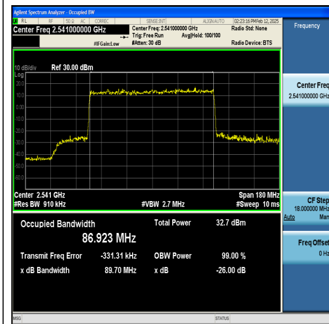
NTNV-n41-PC2-30-90-L-DFT-16QAM-Outer_Full-Ant1- PASS
