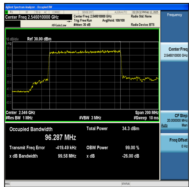
NTNV-n41-PC2-30-100-L-DFT-BPSK-Outer_Full-Ant1- PASS
