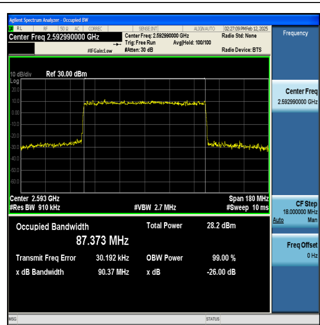
NTNV-n41-PC2-30-90-M-CP-256QAM-Outer_Full-Ant1- PASS
