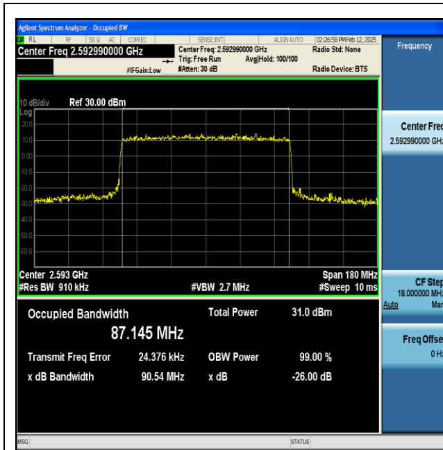
NTNV-n41-PC2-30-90-M-CP-64QAM-Outer_Full-Ant1- PASS
