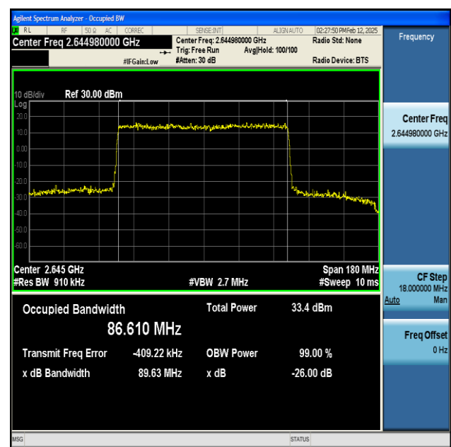
NTNV-n41-PC2-30-90-H-DFT-QPSK-Outer_Full-Ant1- PASS
