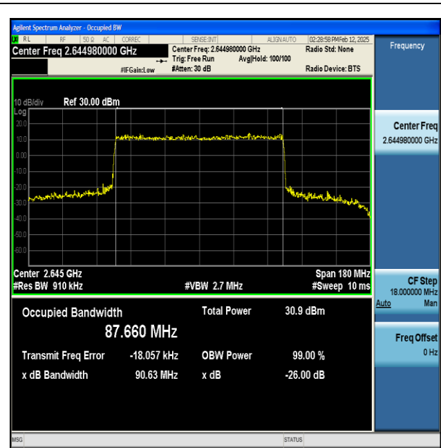
NTNV-n41-PC2-30-90-H-CP-64QAM-Outer_Full-Ant1- PASS
