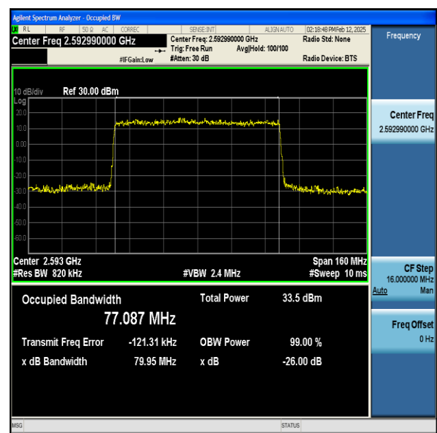
NTNV-n41-PC2-30-80-M-DFT-QPSK-Outer_Full-Ant1-1 PASS
