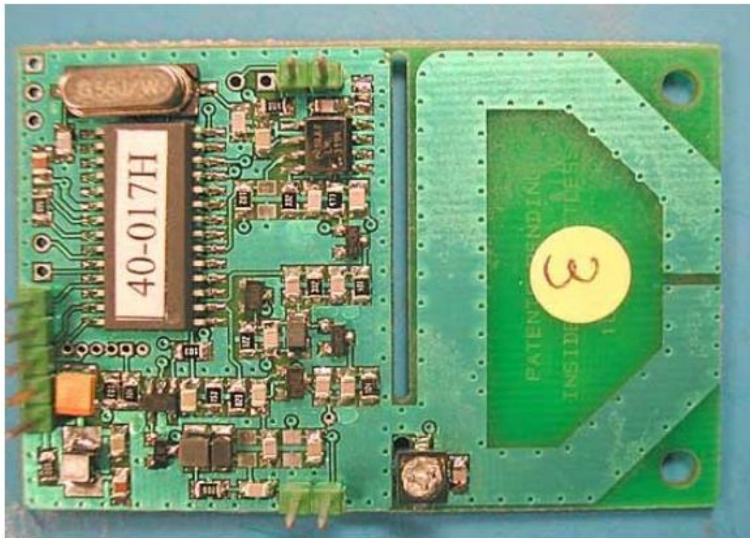
Top with Antenna (on the right)
