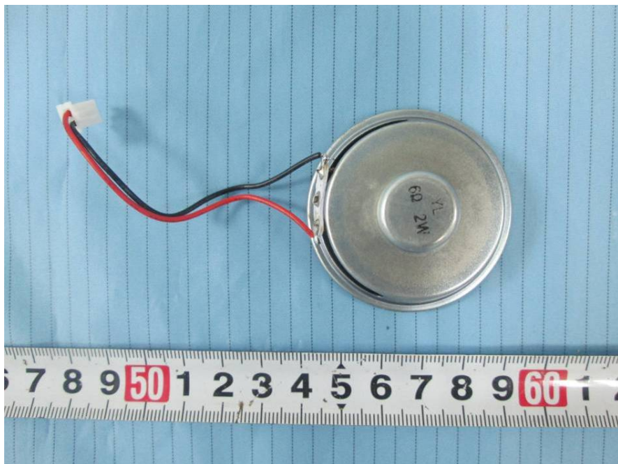
EUT – Loudspeaker Rear View
