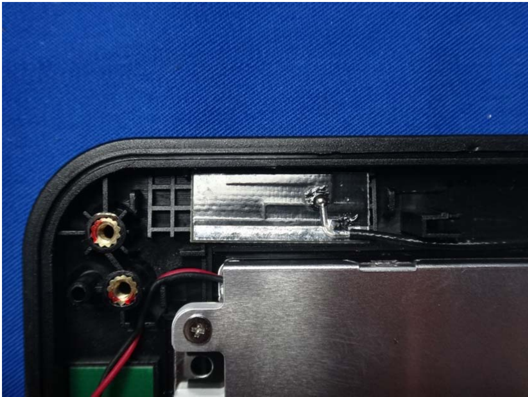
(44) EUT Photo-WLAN+BT Antenna
