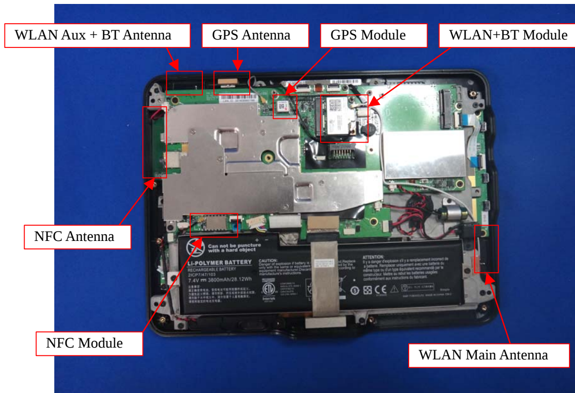
(11) EUT Photo
