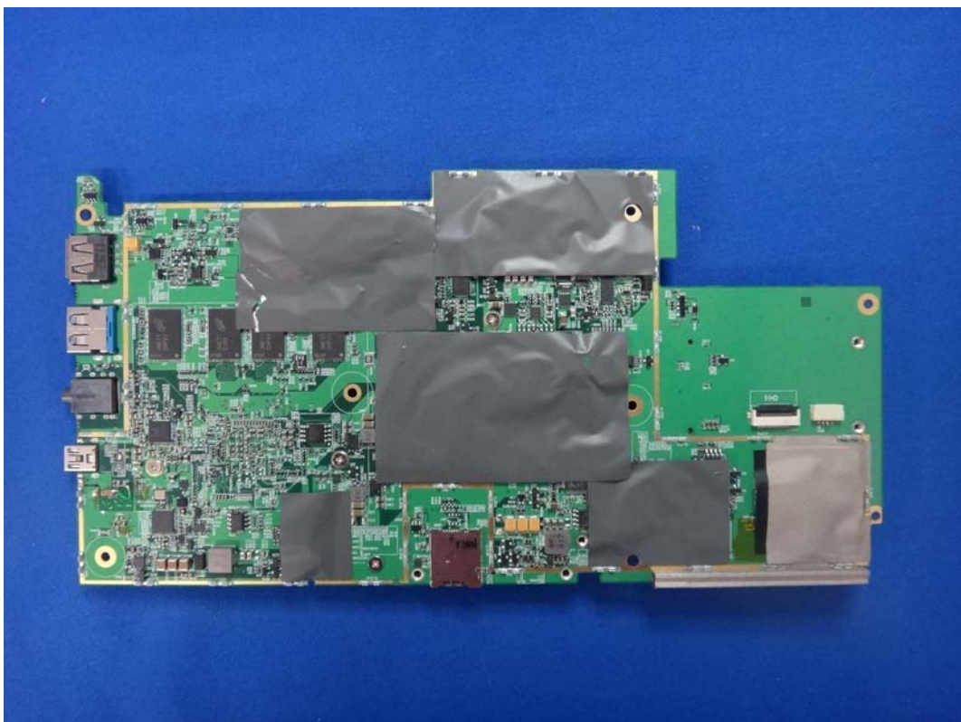
(35) EUT Photo
