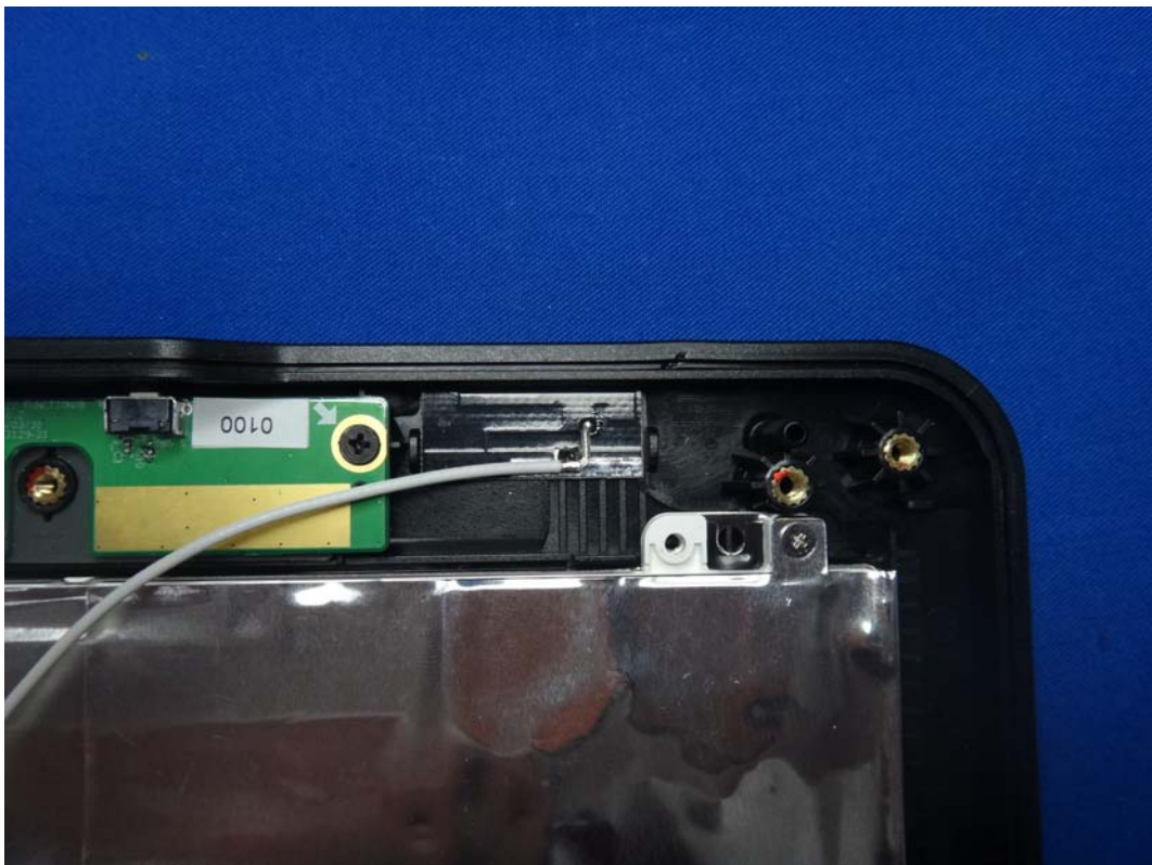
(45) EUT Photo-WLAN+BT Antenna
