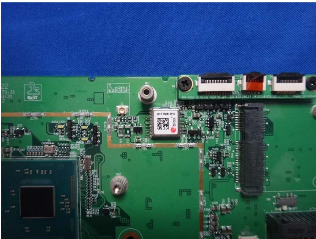
(27) EUT Photo-GPS
