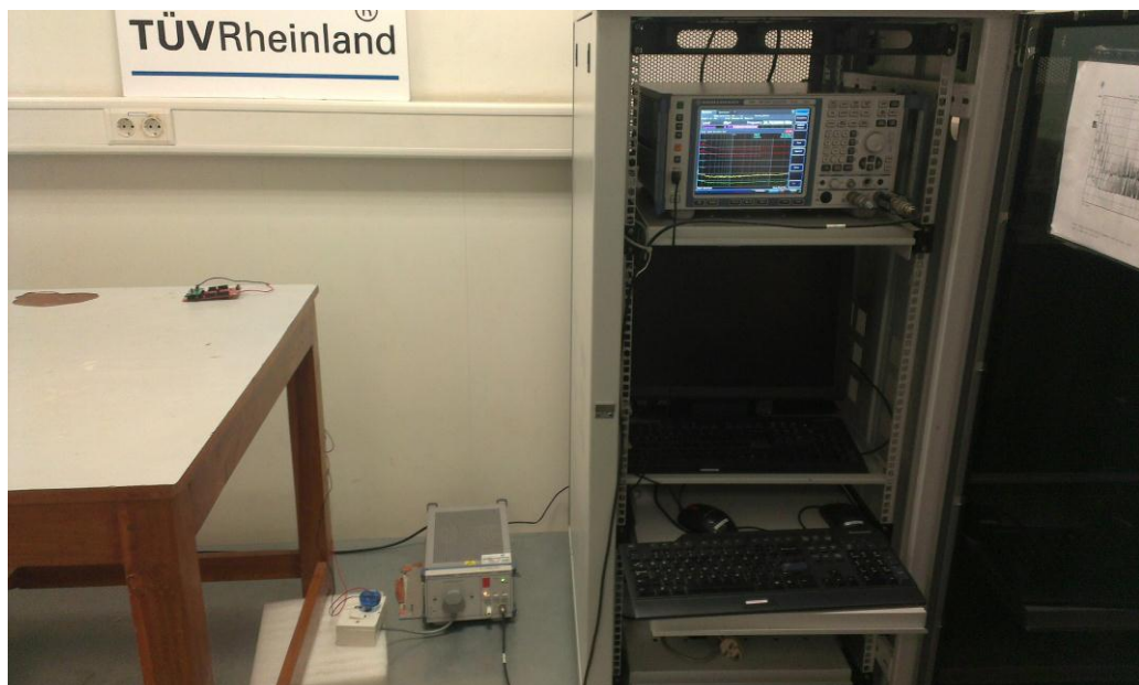
Test setup – Conducted Emission
