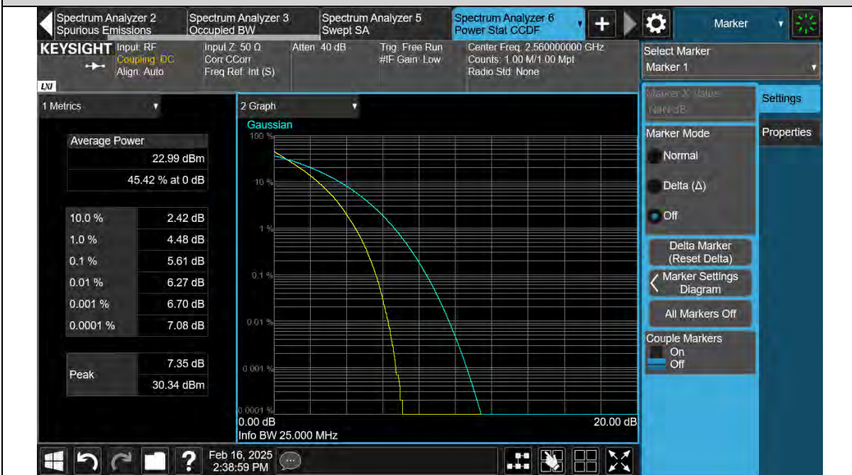
Band7-20MHz-QPSK-21350-100RB#0
