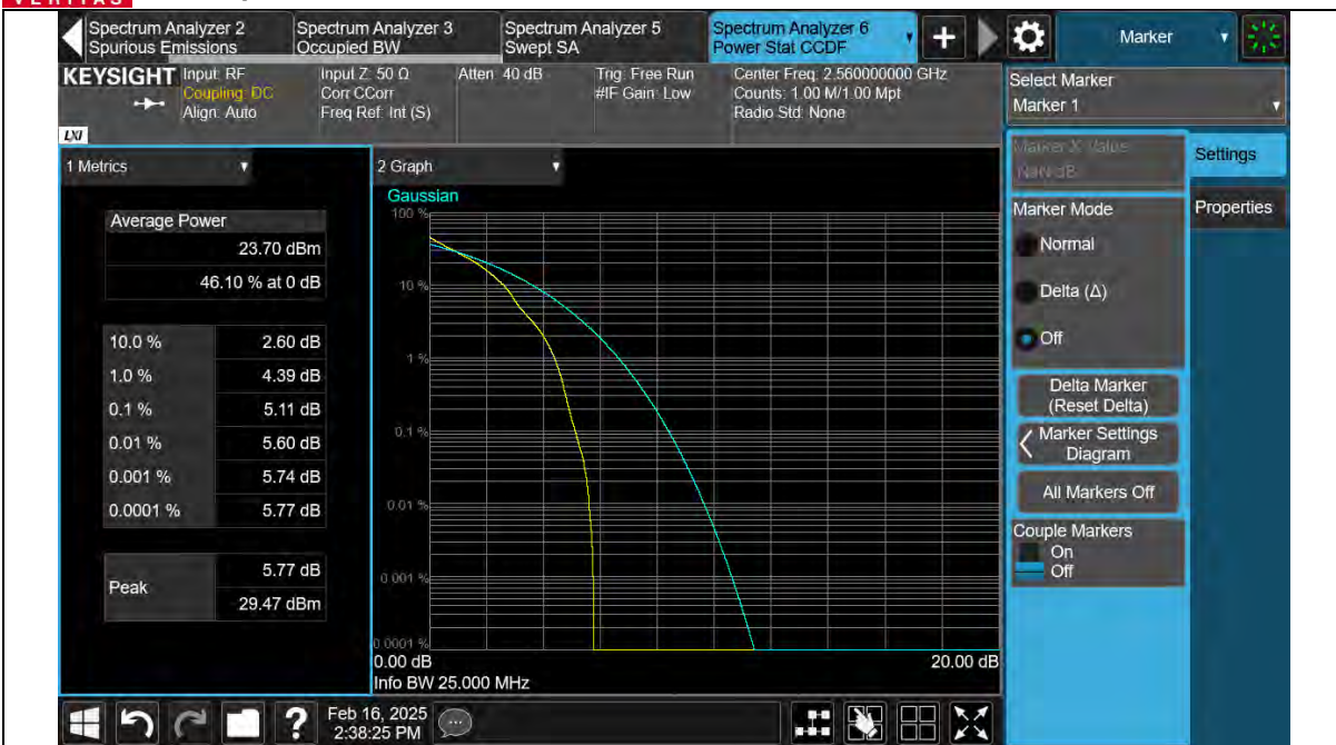
Band7-20MHz-QPSK-21350-1RB#0
