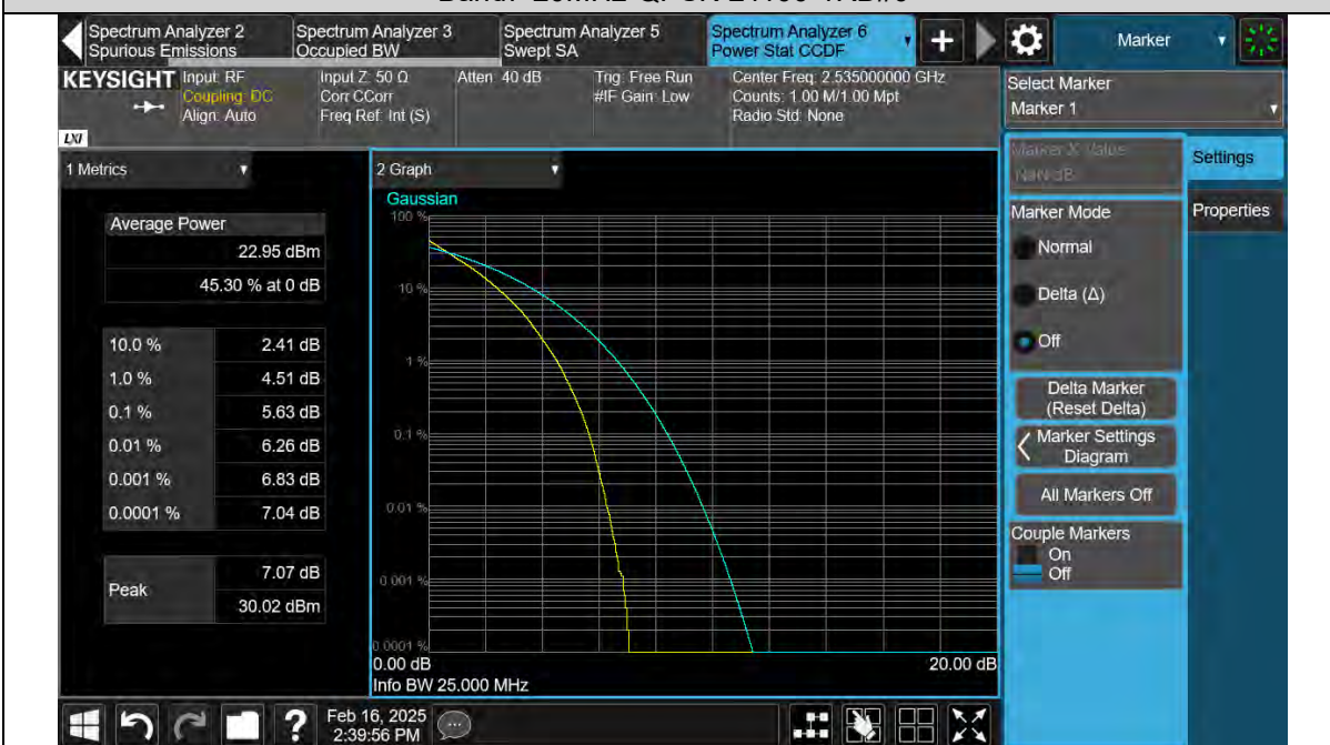
Band7-20MHz-QPSK-21100-100RB#0
