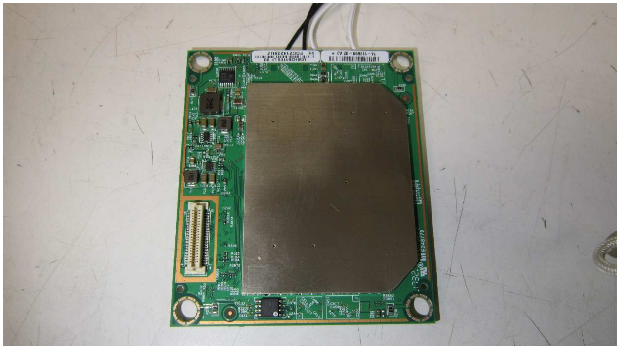
EUT External-Bottom View
