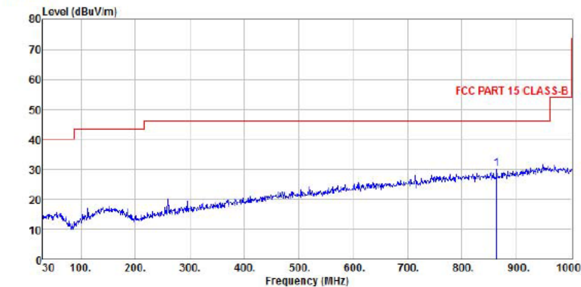
GSM1900 Normal Voltage Condition at Middle Channel
