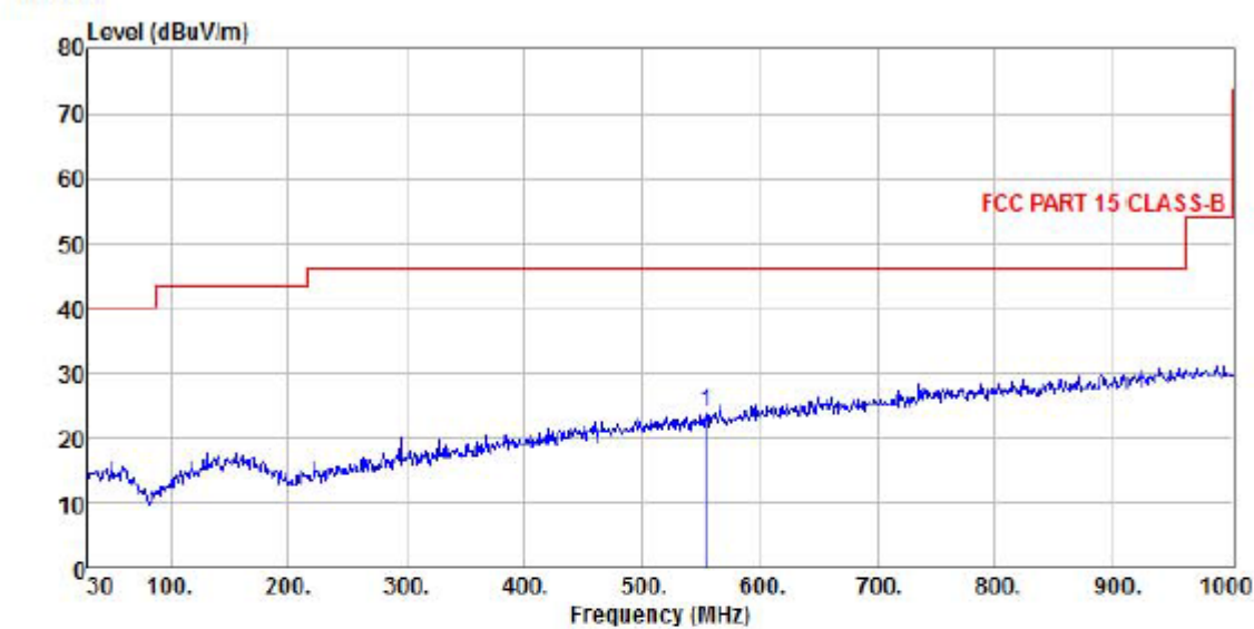
EGPRS850 Normal Voltage Condition at Middle Channel
