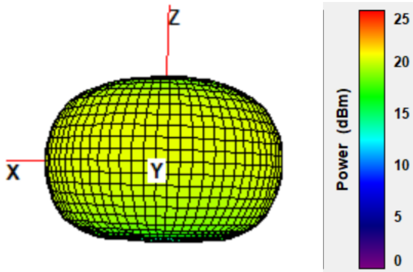
Figure 3 LTE Antenna Radiation Pattern at 707MHz.
