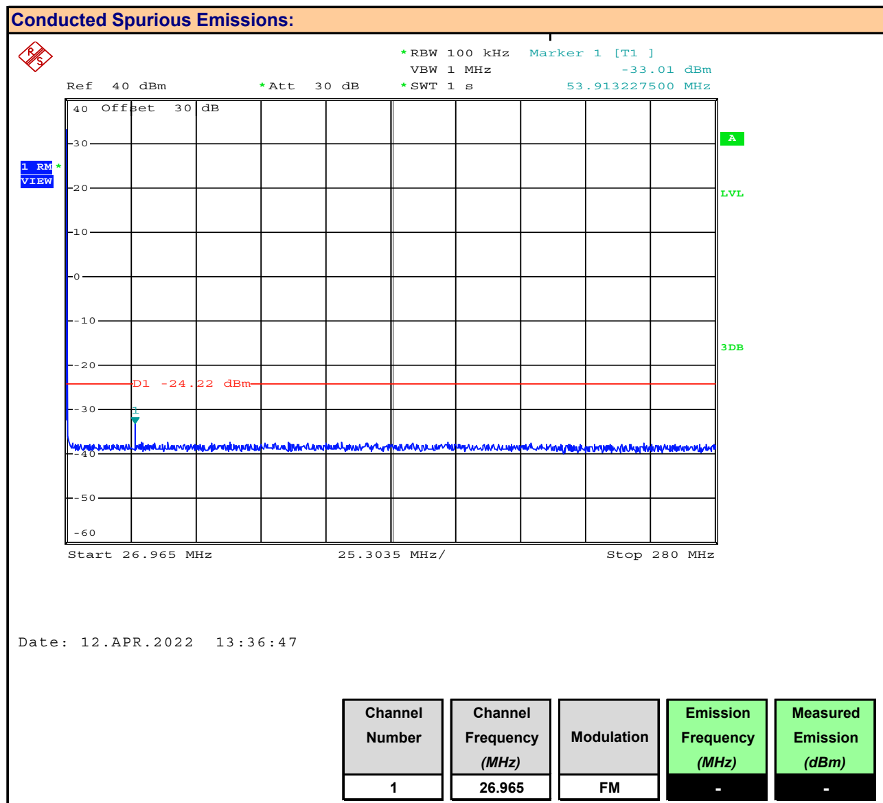
Plot 10.7 – Conducted Out of Band Emissions, 27MHz – 280MHz, Channel 1, FM
