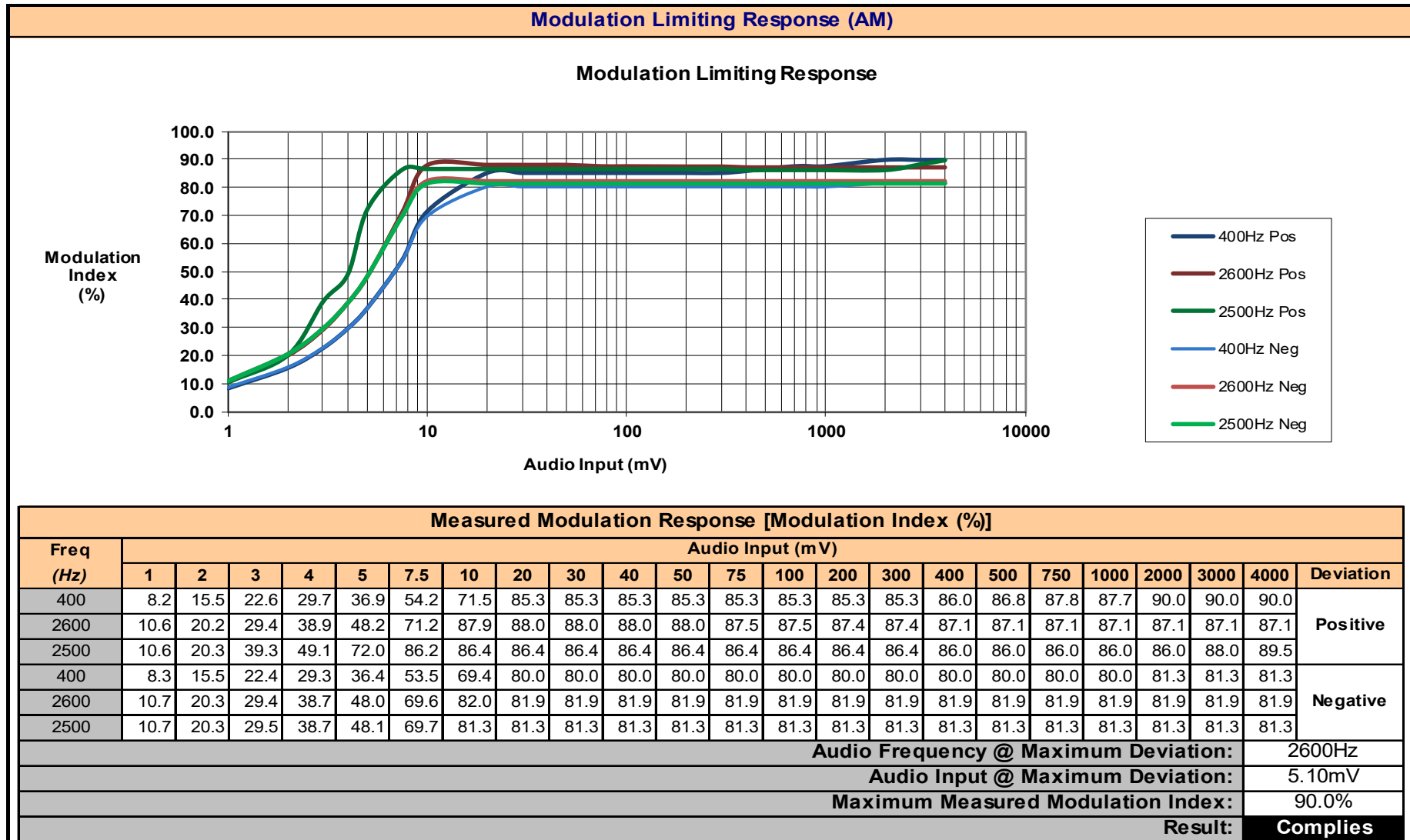
Plot 8.2 – Modulation Limiting Response, AM
