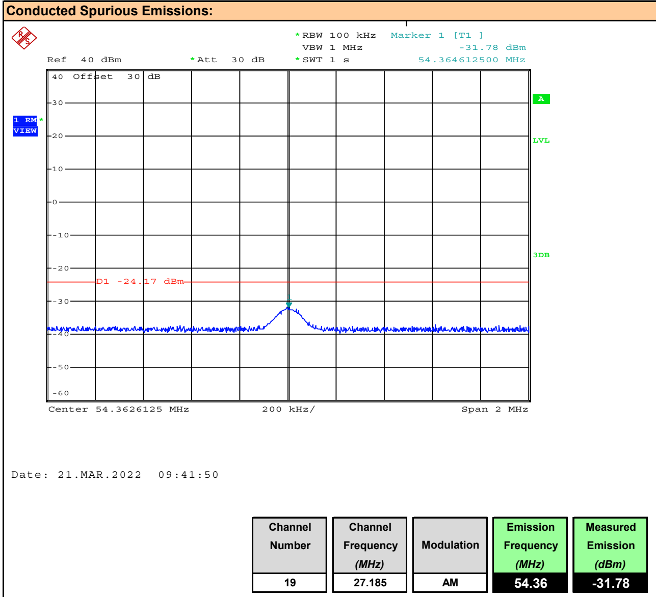
Plot 10.4 – Conducted Out of Band Emissions, 2 nd Harmonic, Channel 19, AM
