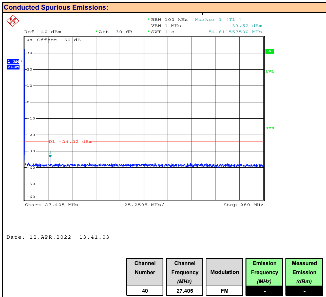
Plot 10.11 – Conducted Out of Band Emissions, 27MHz – 280MHz, Channel 40, FM
