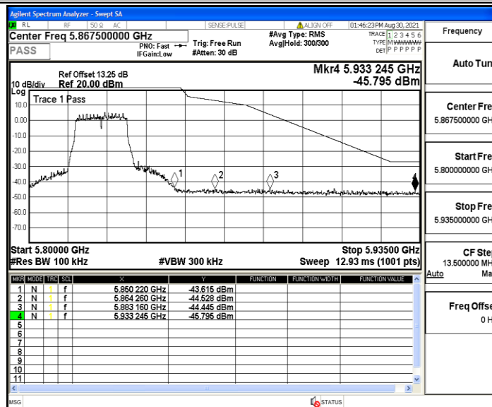
1AC20MIMO_Ant2_High_5825
