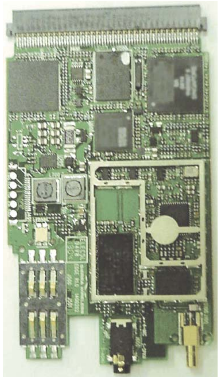
AirCard 775 Dual-Band GSM GPRS/EDGE PCMCIA Modem
