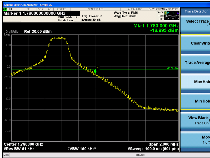
Band66-5MHz-64QAM-132647-1RB#24
