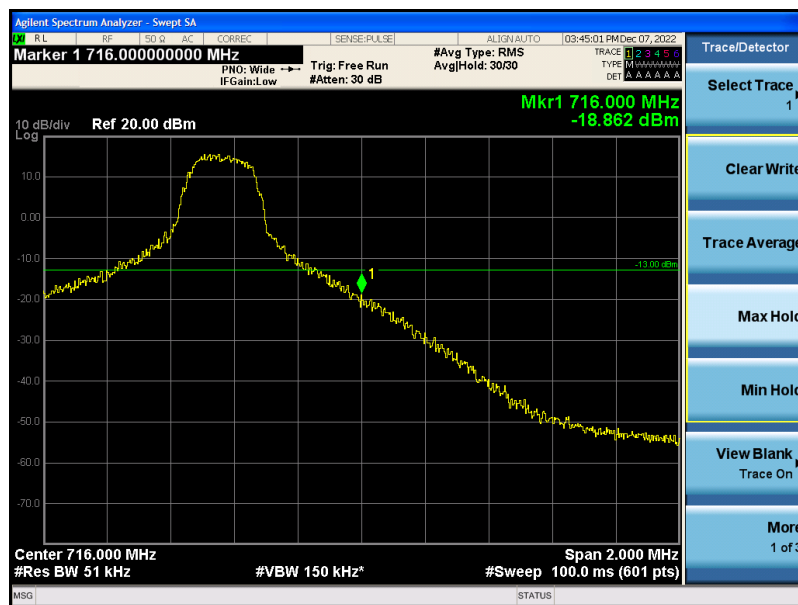
Band12-5MHz-16QAM-23155-1RB#24
