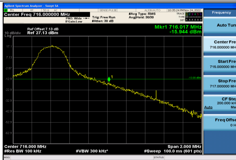
Band12-10MHz-16QAM-23130-1RB#49
