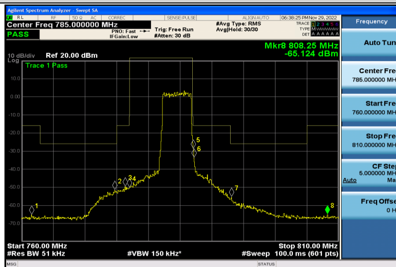
Band13-5MHz-64QAM-23255-25RB#0
