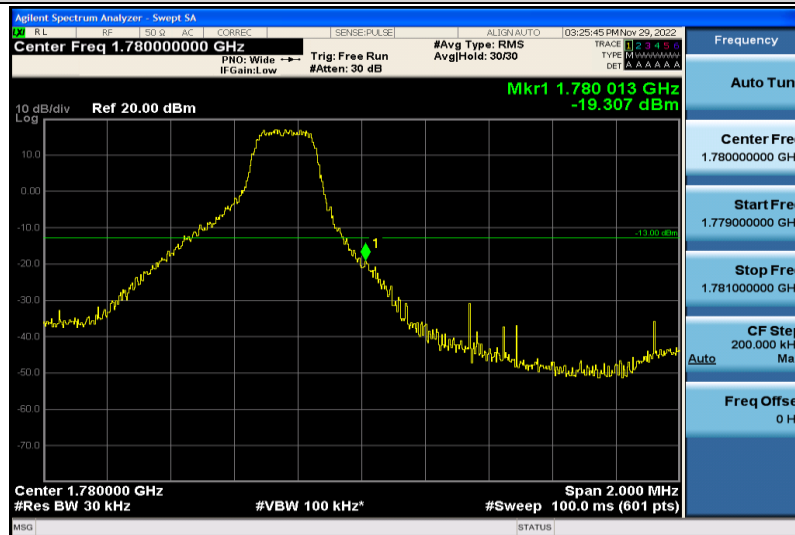
Band66-3MHz-QPSK-132657-1RB#14
