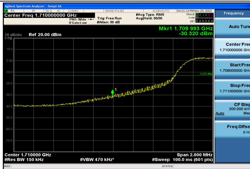
Band66-15MHz-QPSK-132047-75RB#0
