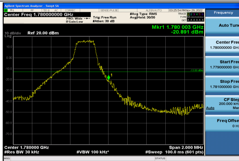
Band66-3MHz-16QAM-132657-1RB#14
