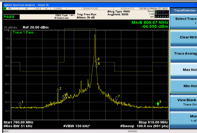
Band13-5MHz-16QAM-23255-1RB#24
