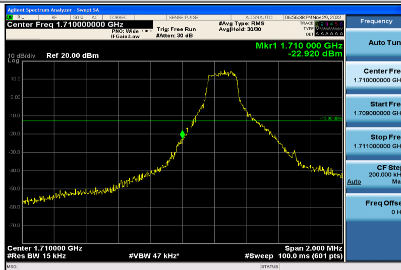
Band66-1.4MHz-64QAM-131979-1RB#0
