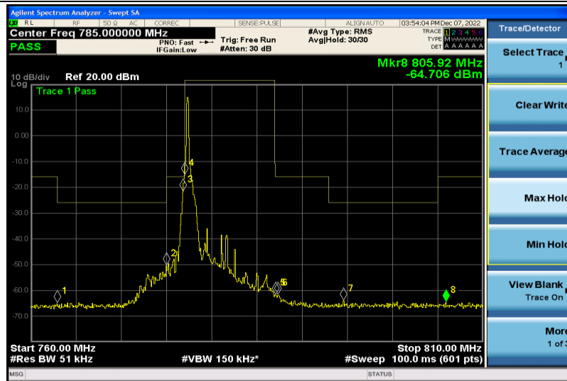
Band13-5MHz-QPSK-23205-1RB#0
