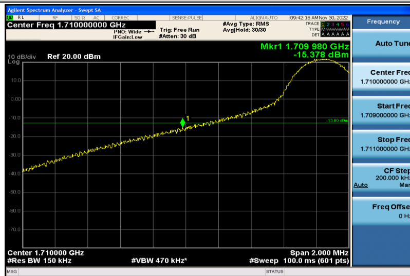
Band66-15MHz-64QAM-132047-1RB#0
