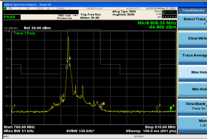
Band13-5MHz-64QAM-23205-1RB#0
