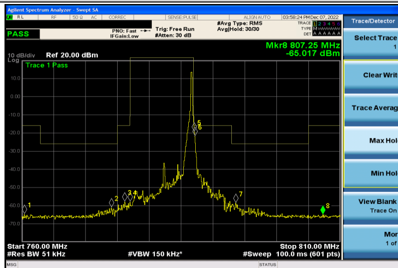
Band13-5MHz-64QAM-23255-1RB#24
