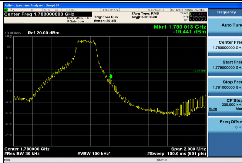
Band66-3MHz-64QAM-132657-1RB#14
