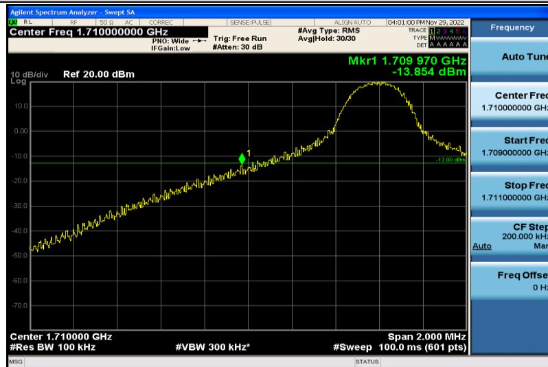
Band66-10MHz-16QAM-132022-1RB#0
