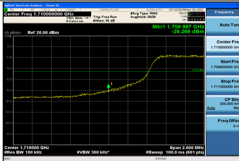
Band66-10MHz-64QAM-132022-50RB#0
