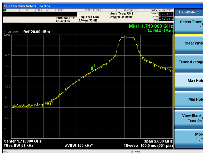
Band66-5MHz-16QAM-131997-1RB#0
