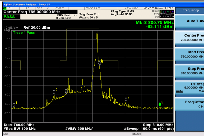
Band13-10MHz-64QAM-23230-1RB#49
