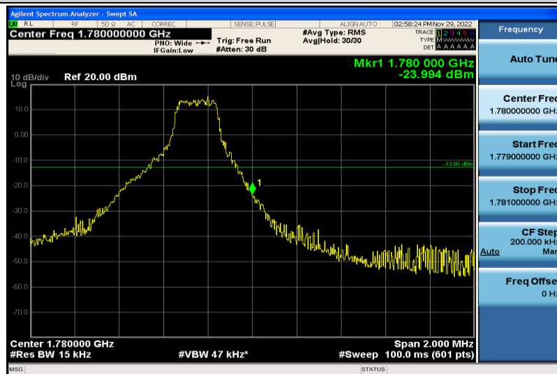
Band66-1.4MHz-16QAM-132665-1RB#5
