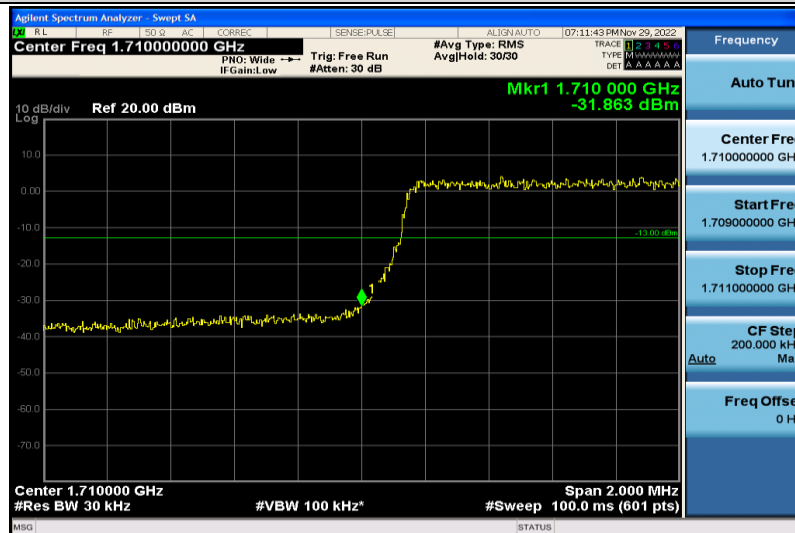
Band66-3MHz-64QAM-131987-15RB#0
