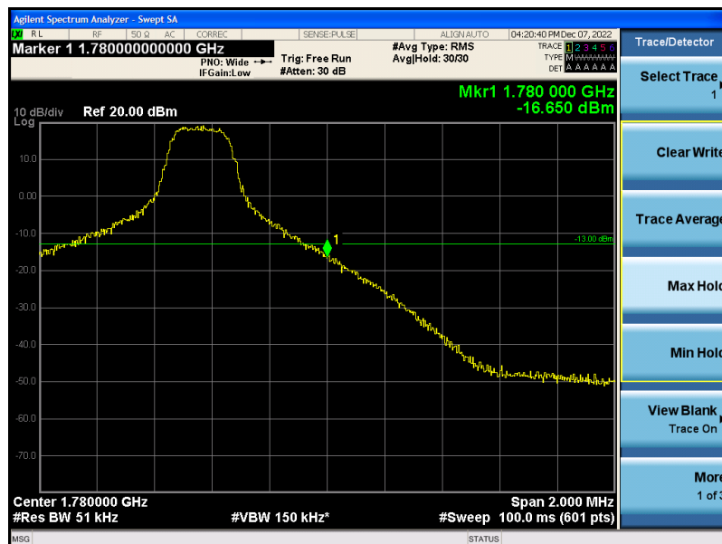
Band66-5MHz-QPSK-132647-1RB#24
