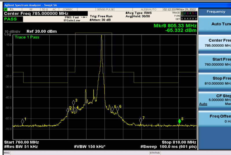
Band13-5MHz-16QAM-23230-1RB#24
