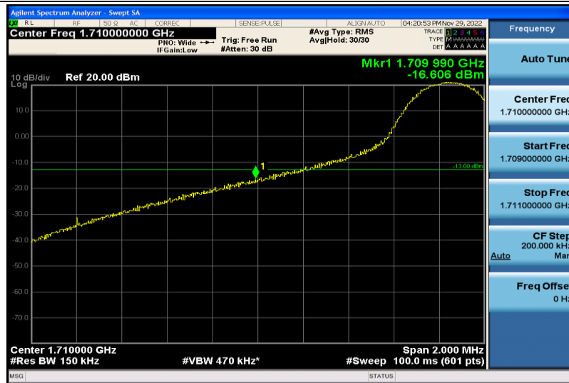
Band66-15MHz-QPSK-132047-1RB#0
