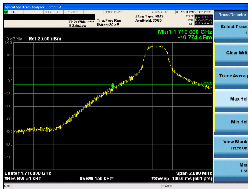
Band66-5MHz-64QAM-131997-1RB#0
