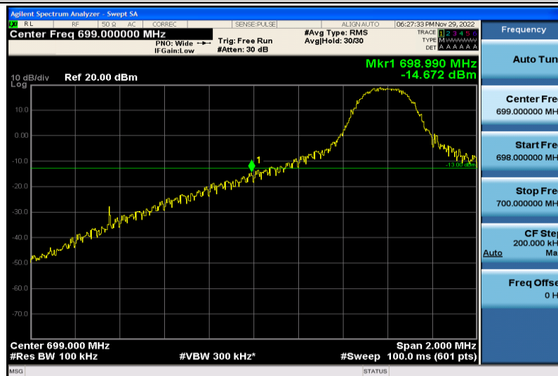
Band12-10MHz-64QAM-23060-1RB#0
