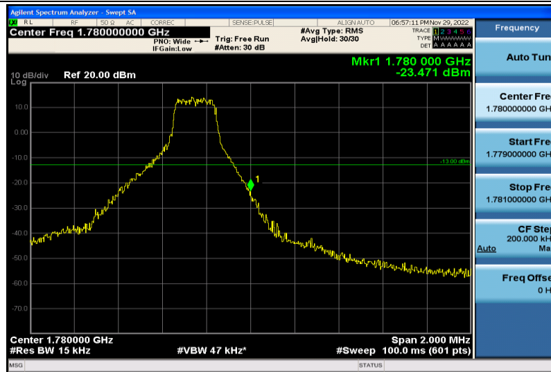
Band66-1.4MHz-64QAM-132665-1RB#5
