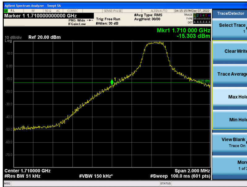
Band66-5MHz-QPSK-131997-1RB#0
