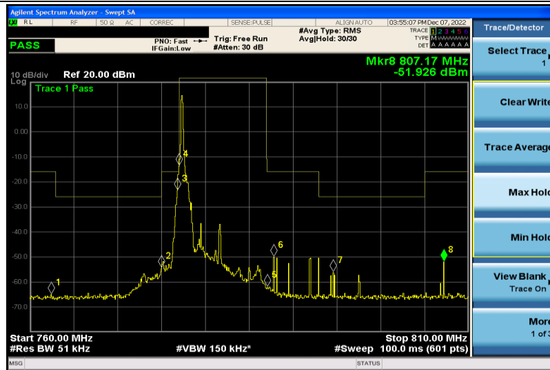
Band13-5MHz-16QAM-23205-1RB#0
