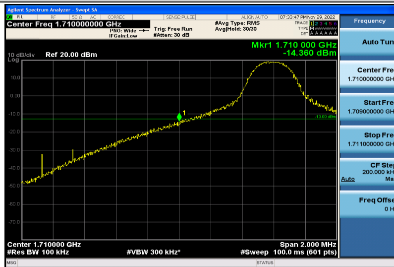
Band66-10MHz-64QAM-132022-1RB#0
