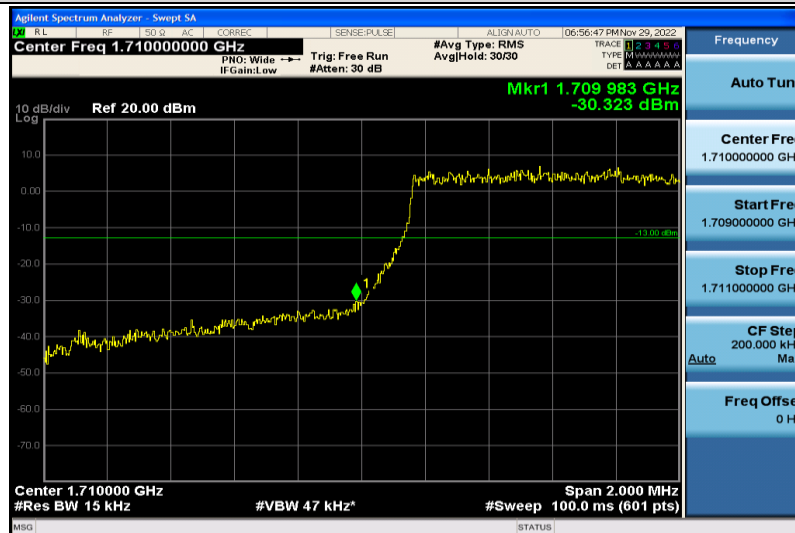
Band66-1.4MHz-64QAM-131979-6RB#0
