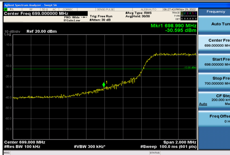
Band12-10MHz-64QAM-23060-50RB#0
