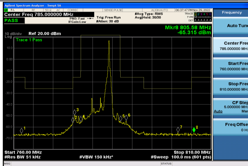
Band13-5MHz-64QAM-23230-1RB#24
