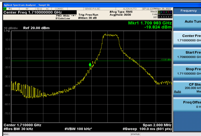
Band66-3MHz-64QAM-131987-1RB#0
