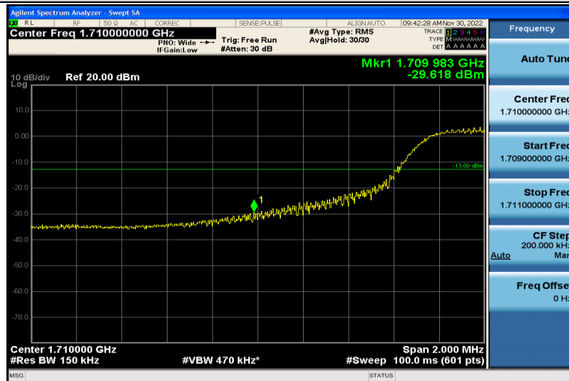
Band66-15MHz-64QAM-132047-75RB#0
