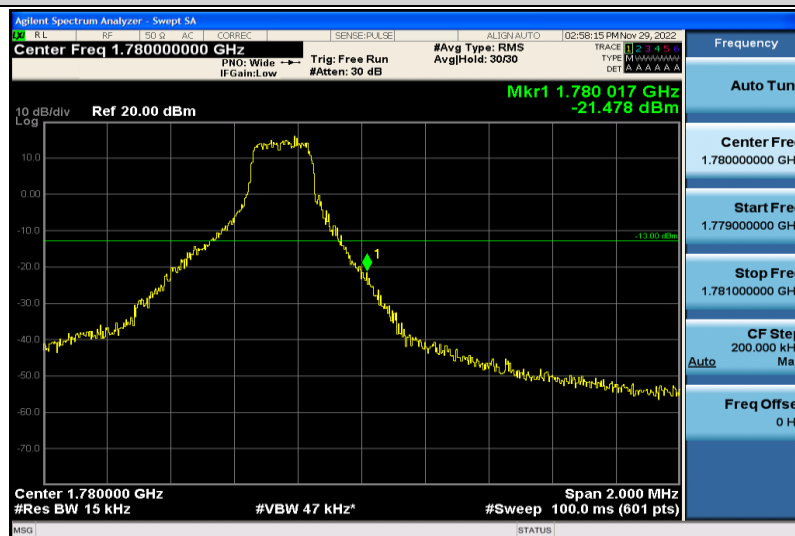
Band66-1.4MHz-QPSK-132665-1RB#5
