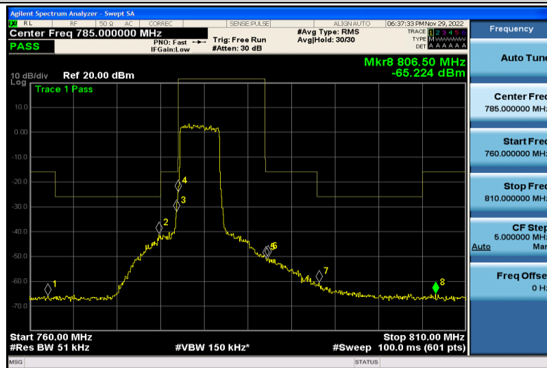
Band13-5MHz-64QAM-23205-25RB#0
