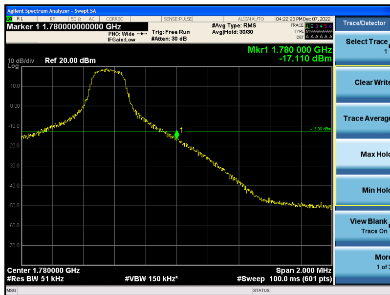
Band66-5MHz-16QAM-132647-1RB#24
