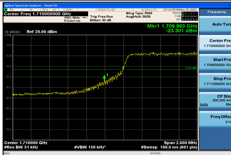
Band66-5MHz-64QAM-131997-25RB#0
