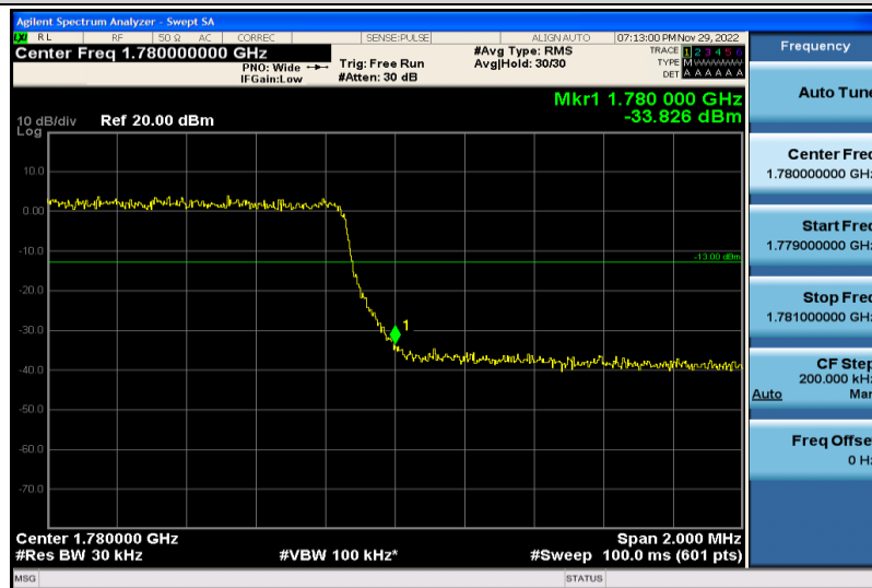
Band66-3MHz-64QAM-132657-15RB#0
