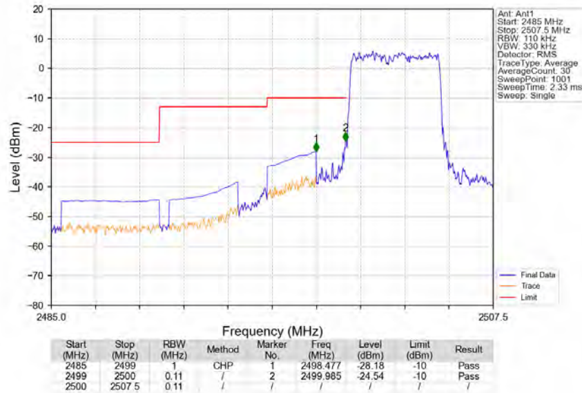
Band7_5MHz_64QAM_LCH_2502.5MHz_RB_25_0_NTNV
