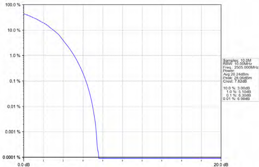
Band7_10MHz_64QAM_LCH_2505MHz_RB_50_0_NTNV
