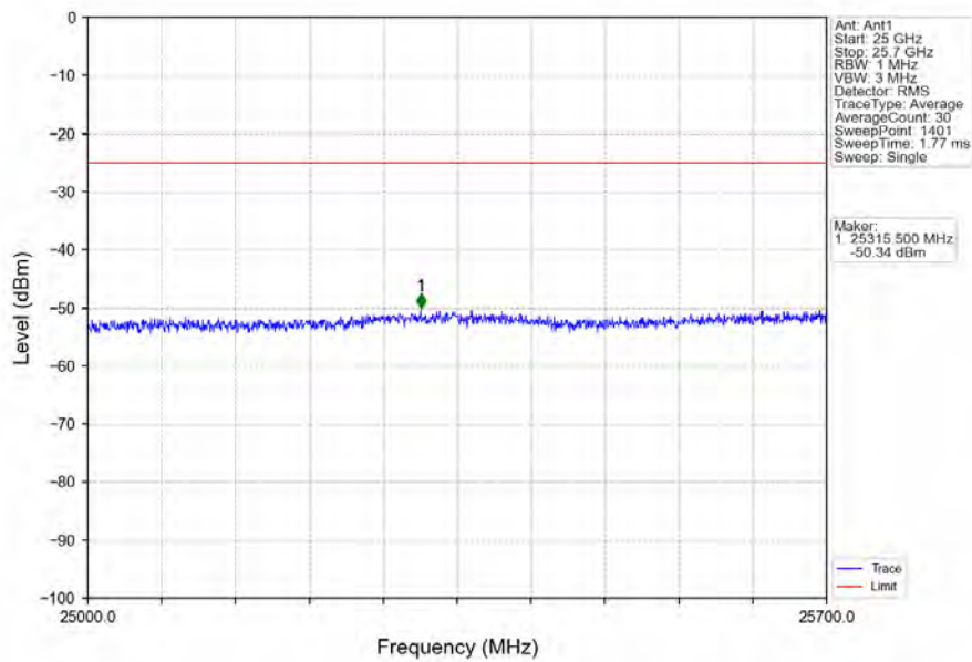
Band7_5MHz_16QAM_HCH_2567.5MHz_RB_1_0_NTNV
