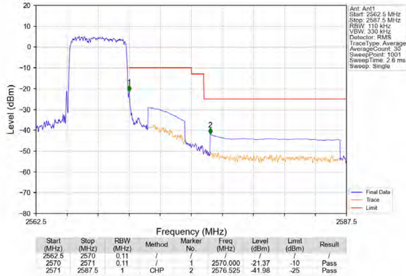
Band7_5MHz_64QAM_HCH_2567.5MHz_RB_25_0_NTNV
