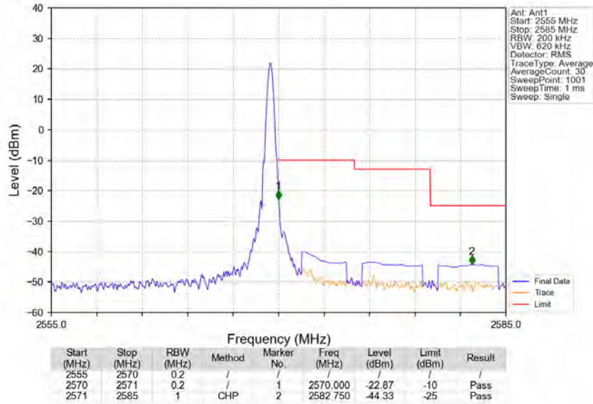
Band7_10MHz_16QAM_HCH_2565MHz_RB_1_49_NTNV
