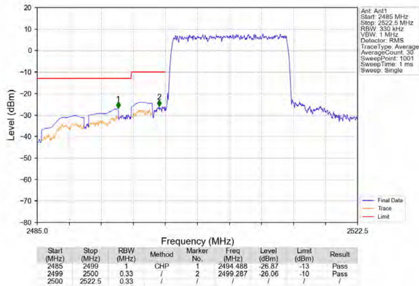
Band7_15MHz_QPSK_LCH_2507.5MHz_RB_75_0_NTNV
