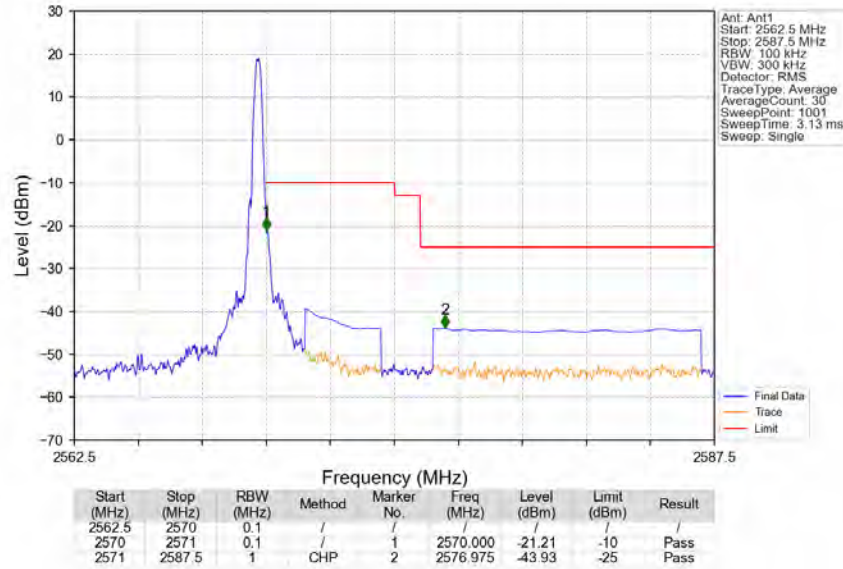
Band7_5MHz_16QAM_HCH_2567.5MHz_RB_1_24_NTNV
