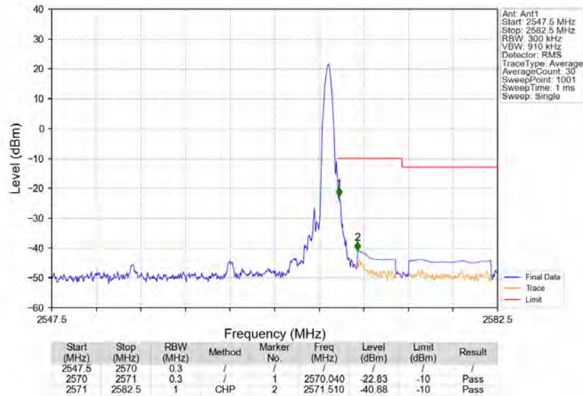
Band7_15MHz_16QAM_HCH_2562.5MHz_RB_1_74_NTNV
