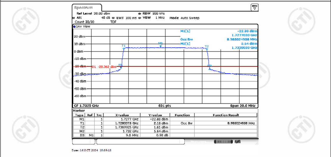
Band4-10MHz-QPSK-20175-50RB#0-8.985
