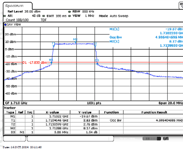
Band4-10MHz-16QAM-20000-25RB#0-4.595
