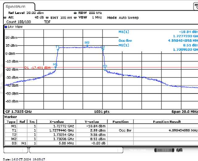
Band4-10MHz-16QAM-20175-25RB#0-4.595
