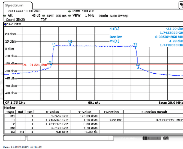
Band4-10MHz-QPSK-20350-50RB#0-8.985
