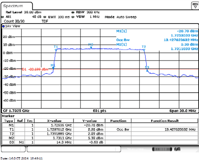
Band4-15MHz-QPSK-20175-75RB#0-13.428
