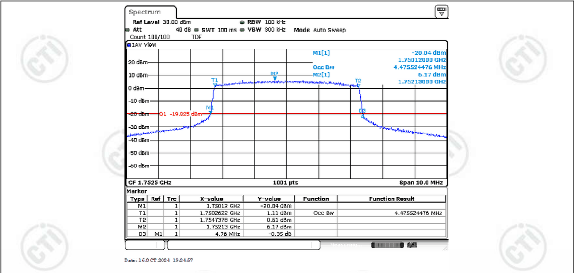
Band4-5MHz-16QAM-20375-25RB#0-4.476
