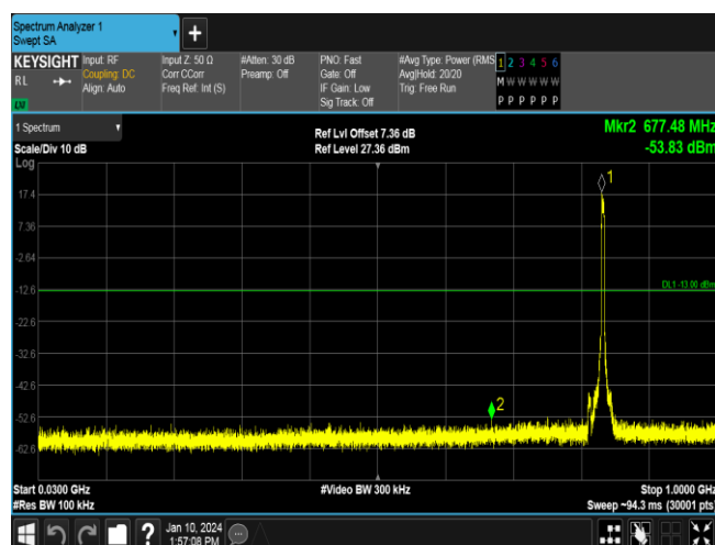
WCDMA 850_RMC 12.2kps_MCH
