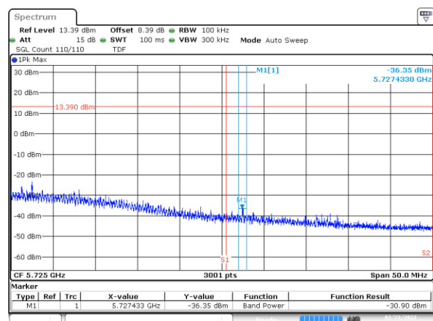
BE-NR-HIGH, MIMO-B, 802.11n40-HT0, Ch134
