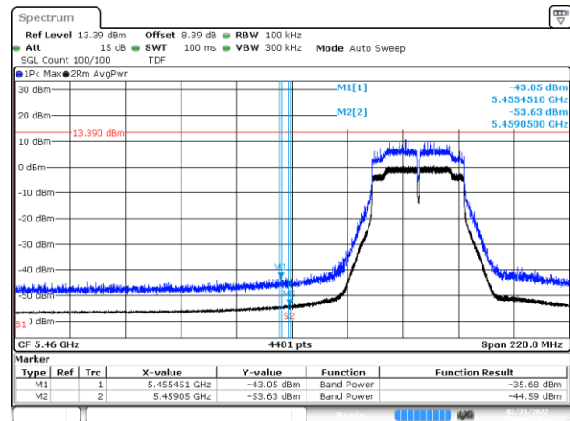
BE-R-LOW, MIMO-B, 802.11n40-HT0, Ch102
