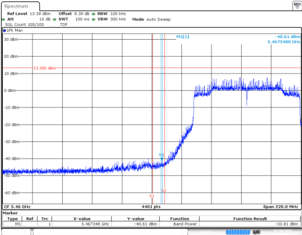
BE-NR-LOW, MIMO-B, 802.11ax80-HE0, Ch106
