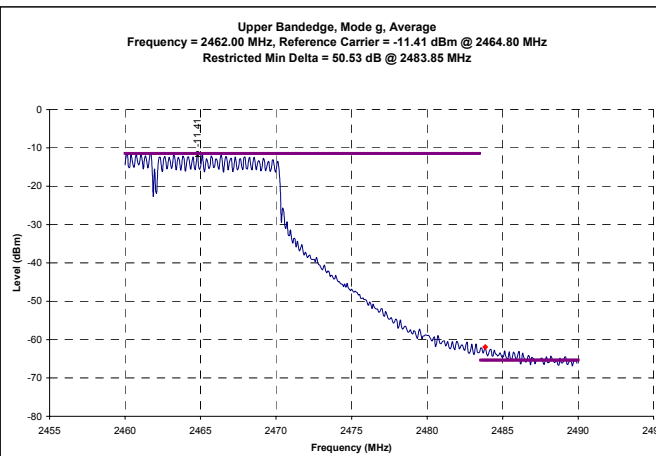
Channel 11 - Average Conducted Band-edge Plots
