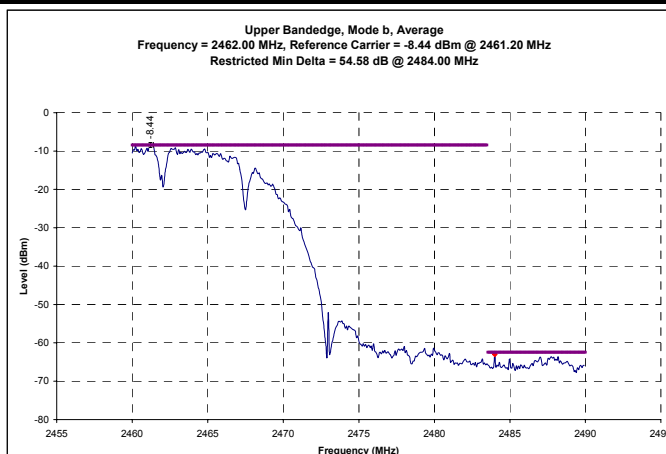
Channel 11 - Average Conducted Band-edge Plots
