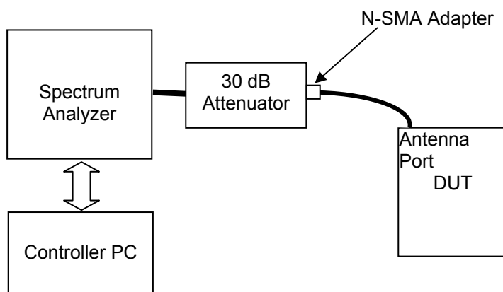
Figure G.6-1 - Setup Drawing
