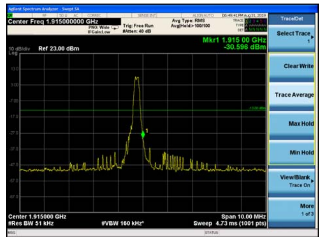
LTE Band 25 1.4MHz QPSK 100%RB CH-High
