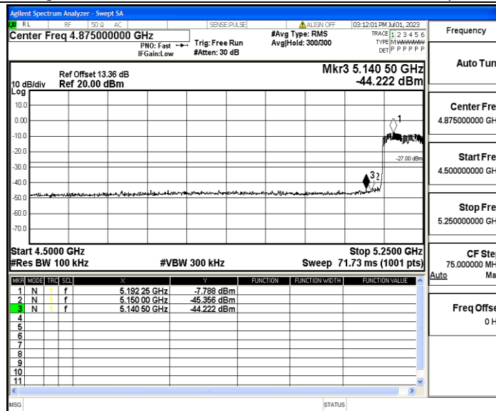
11AC80MIMO_Ant1_High_5210
