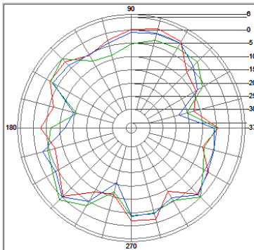
Ant 3, Theta, XY-Plan
