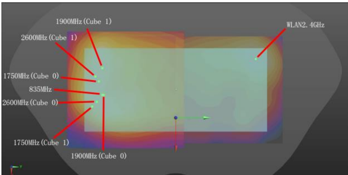
Back for WWAN+WLAN2.4GHz_5mm
