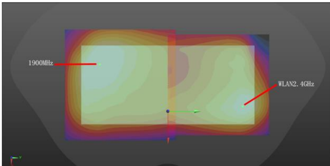
Front for WWAN+WLAN2.4GHz_5mm
