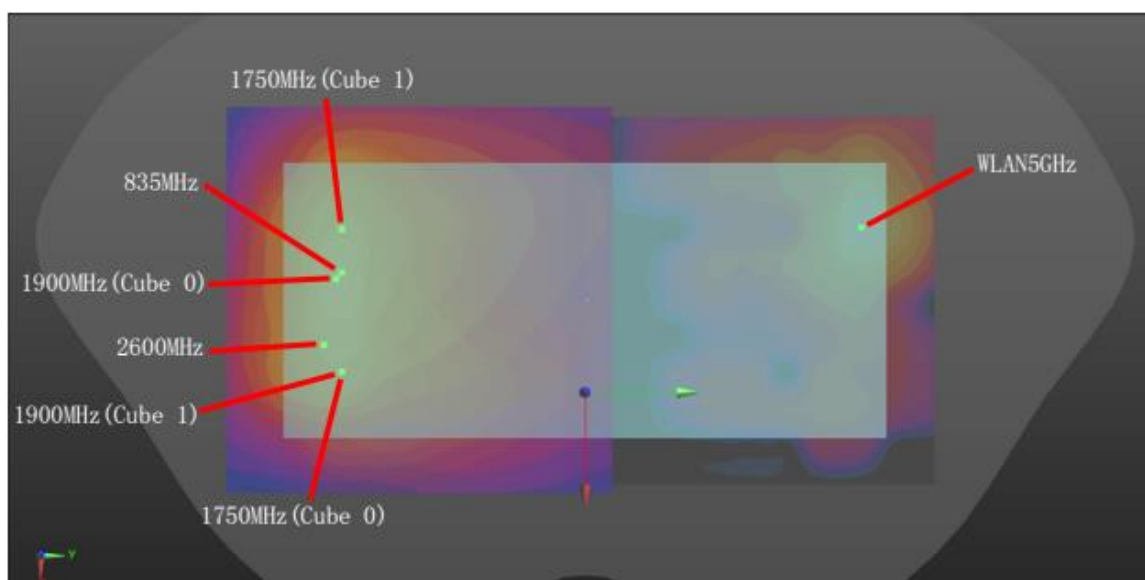
Back for WWAN+WLAN5GHz_0mm
