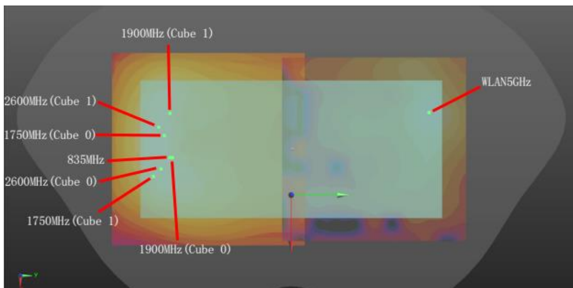
Back for WWAN+WLAN5GHz_5mm
