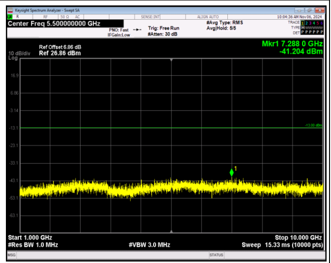
Band5-1.4MHz-64QAM-20643-1RB#0-Range2:1000~10000MHz
