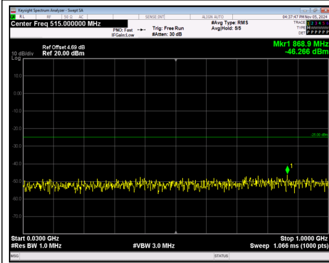
Band7-20MHz-64QAM-20850-1RB#0-Range1:30~100 OMHz
