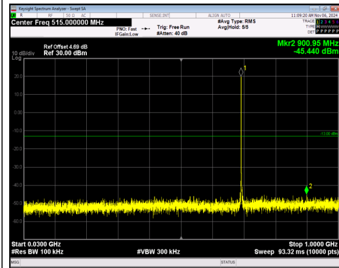
Band12-1.4MHz-64QAM-23095-1RB#0-Range1:30~1000MHz
