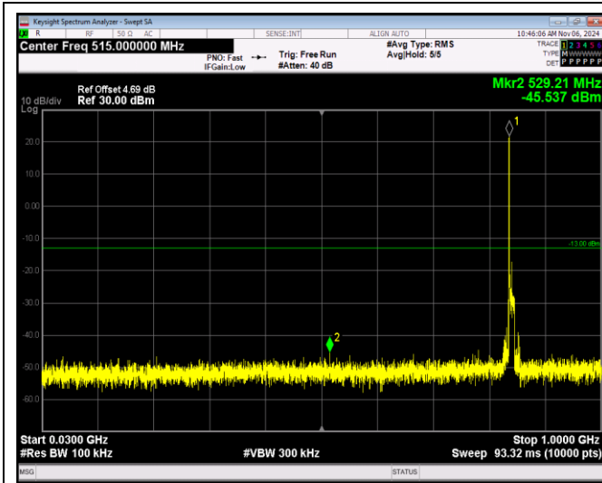
Band5-10MHz-16QAM-20450-1RB#0-Range1:30~100 OMHz
