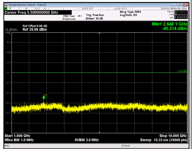
Band5-1.4MHz-64QAM-20643-1RB#0-Range2:1000~10000MHz
