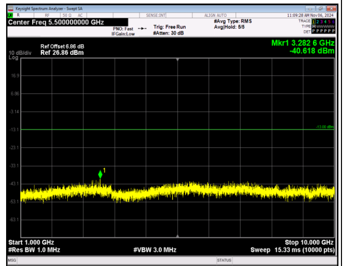
Band12-1.4MHz-64QAM-23095-1RB#0-Range2:1000~10000MHz
