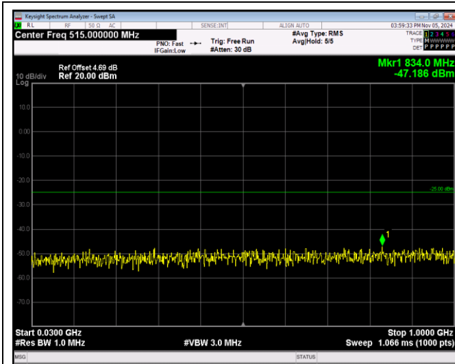
Band7-20MHz-QPSK-20850-1RB#0-Range1:30~1000 MHz
