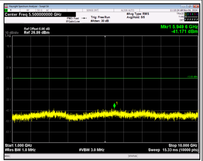
Band12-1.4MHz-64QAM-23095-1RB#0-Range2:1000~10000MHz
