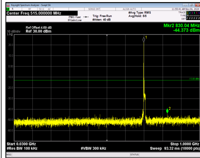
Band12-10MHz-16QAM-23060-1RB#0-Range1:30~10 00MHz
