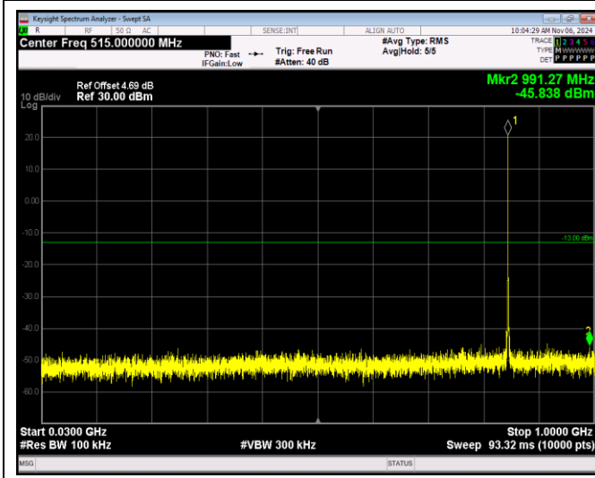
Band5-1.4MHz-64QAM-20643-1RB#0-Range1:30~1000MHz
