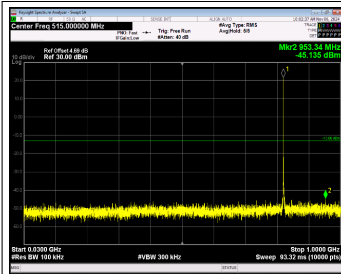
Band5-1.4MHz-64QAM-20525-1RB#0-Range1:30~1000MHz
