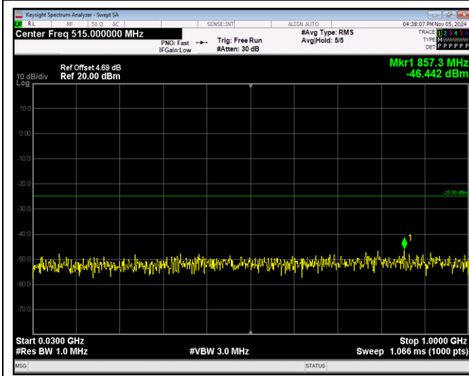
Band7-20MHz-QPSK-21100-1RB#0-Range1:30~1000 MHz
