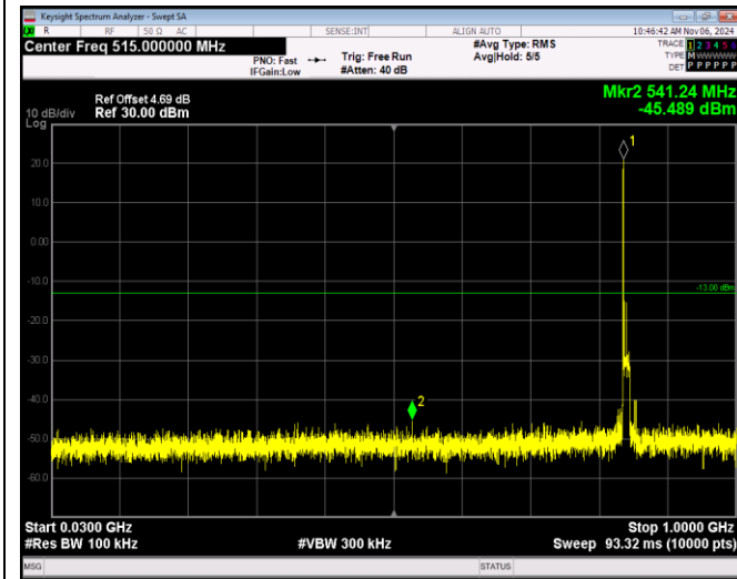
Band7-5MHz-QPSK-20775-1RB#0-Range1:30~1000 MHz
