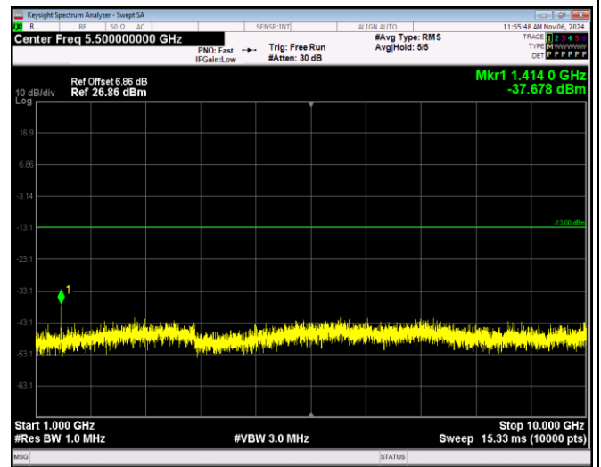
Band12-10MHz-16QAM-23060-1RB#0-Range2:1000~ 10000MHz
