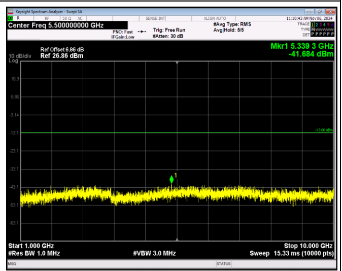
Band12-1.4MHz-QPSK-23173-1RB#0-Range2:1000~10000MHz
