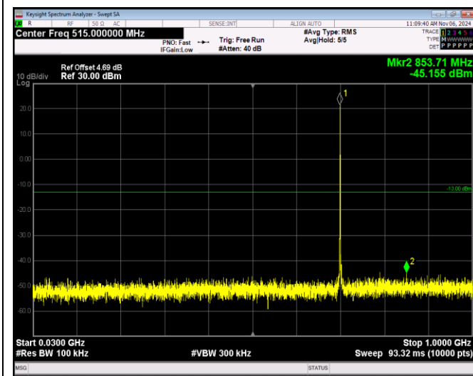
Band12-1.4MHz-QPSK-23173-1RB#0-Range1:30~1000MHz
