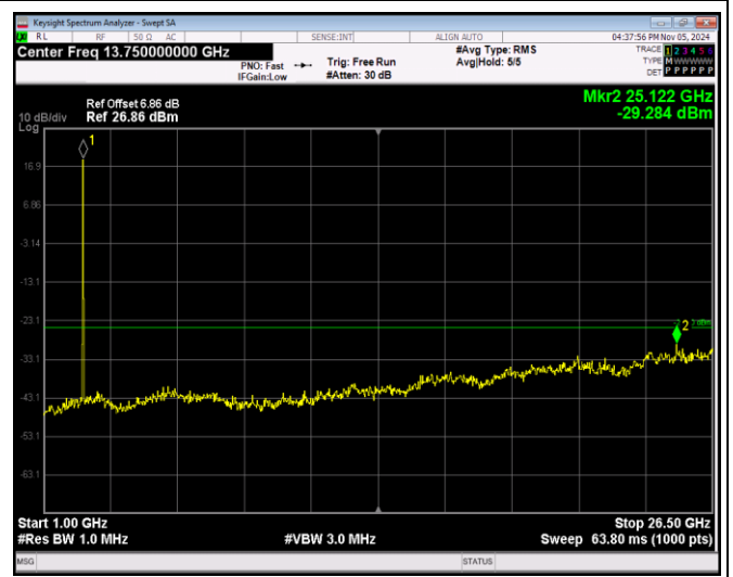
Band7-20MHz-64QAM-20850-1RB#0-Range2:1000~2 6500MHz
