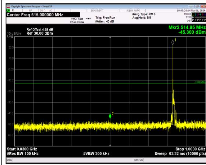
Band5-10MHz-16QAM-20525-1RB#0-Range1:30~100 OMHz
