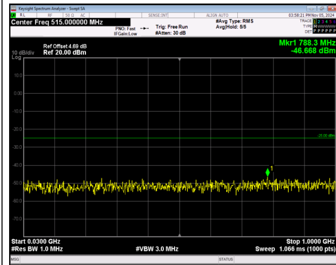
Band7-5MHz-16QAM-21425-1RB#0-Range1:30~1000 MHz
