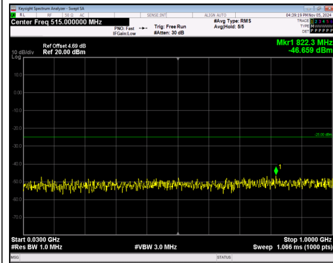
Band7-20MHz-64QAM-20850-1RB#0-Range1:30~100 OMHz
