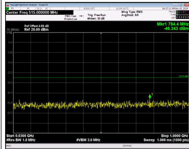
Band7-20MHz-QPSK-21100-1RB#0-Range1:30~1000 MHz
