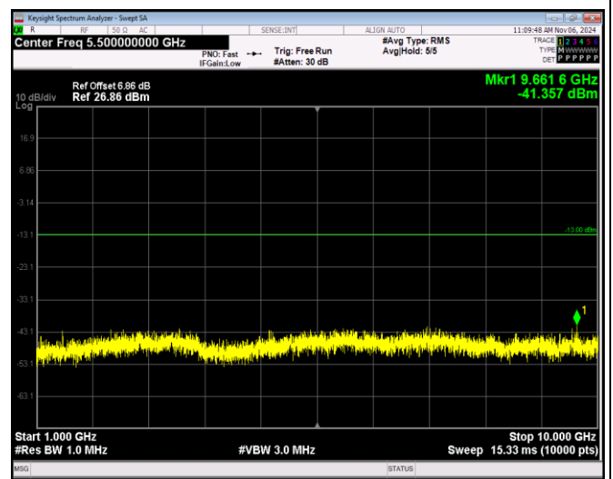
Band12-1.4MHz-QPSK-23173-1RB#0-Range2:1000~10000MHz
