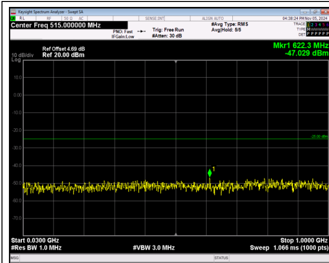
Band7-20MHz-16QAM-21350-1RB#0-Range1:30~100 OMHz
