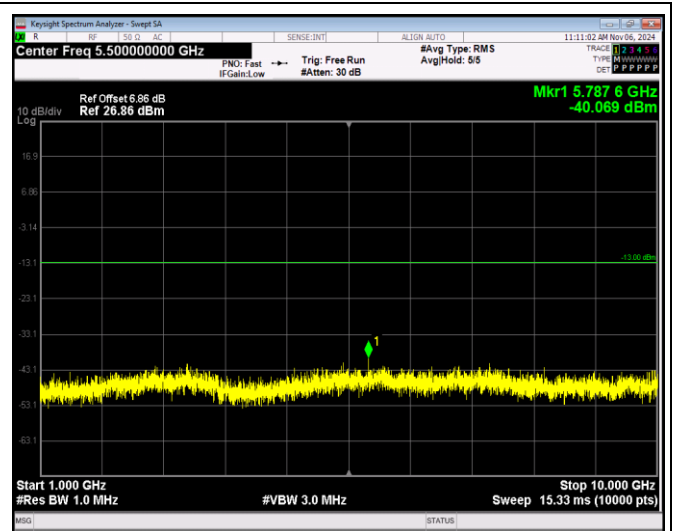
Band12-1.4MHz-64QAM-23017-1RB#0-Range2:1000~10000MHz
