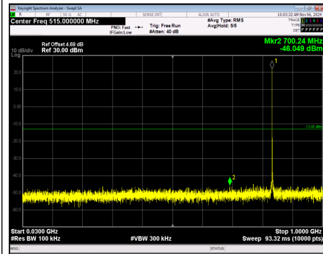
Band5-1.4MHz-64QAM-20643-1RB#0-Range1:30~1000MHz
