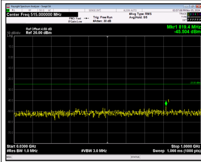
Band7-5MHz-QPSK-20775-1RB#0-Range1:30~1000 MHz
