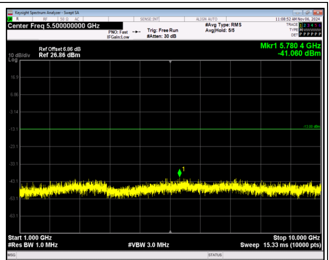
Band12-1.4MHz-QPSK-23095-1RB#0-Range2:1000~10000MHz
