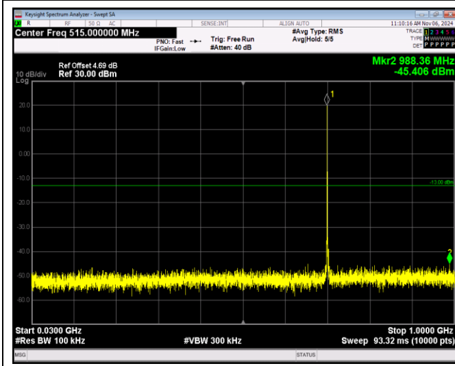
Band12-1.4MHz-64QAM-23095-1RB#0-Range1:30~1000MHz
