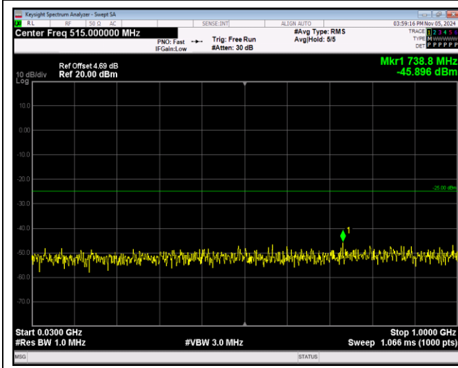
Band7-5MHz-16QAM-21425-1RB#0-Range1:30~1000 MHz
