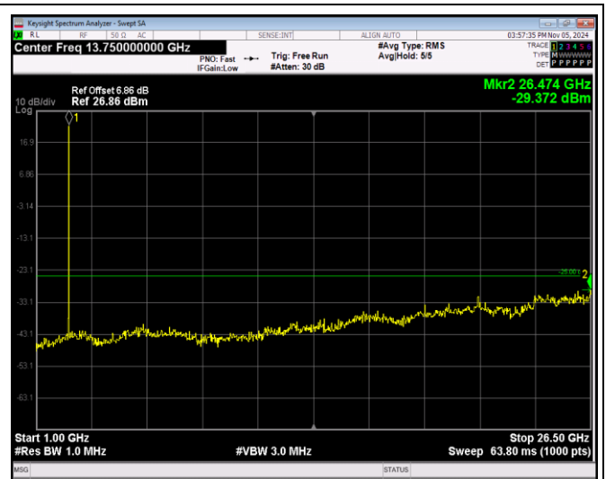
Band7-5MHz-16QAM-21100-1RB#0-Range2:1000~26 500MHz
