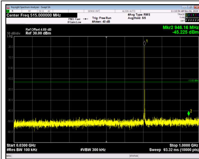
Band12-1.4MHz-64QAM-23017-1RB#0-Range1:30~1000MHz
