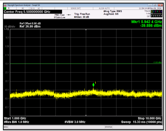
Band12-10MHz-16QAM-23060-1RB#0-Range2:1000~ 10000MHz
