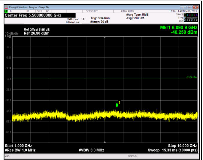
Band5-10MHz-16QAM-20450-1RB#0-Range2:1000~1 0000MHz
