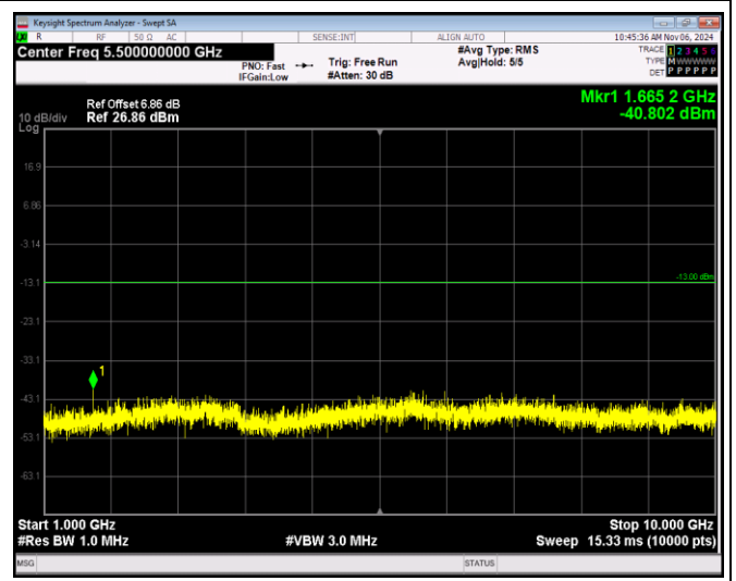
Band5-10MHz-16QAM-20525-1RB#0-Range2:1000~1 0000MHz
