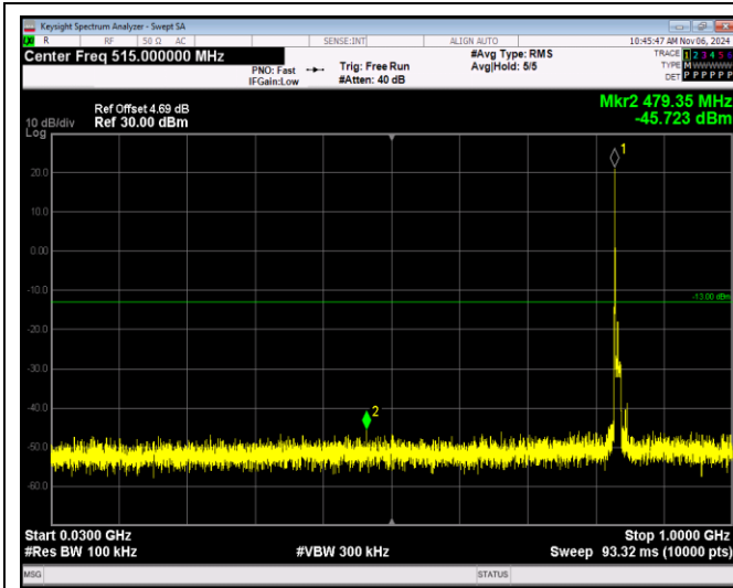
Band5-10MHz-64QAM-20600-1RB#0-Range1:30~100 OMHz
