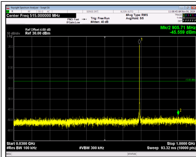
Band12-1.4MHz-QPSK-23095-1RB#0-Range1:30~1000MHz
