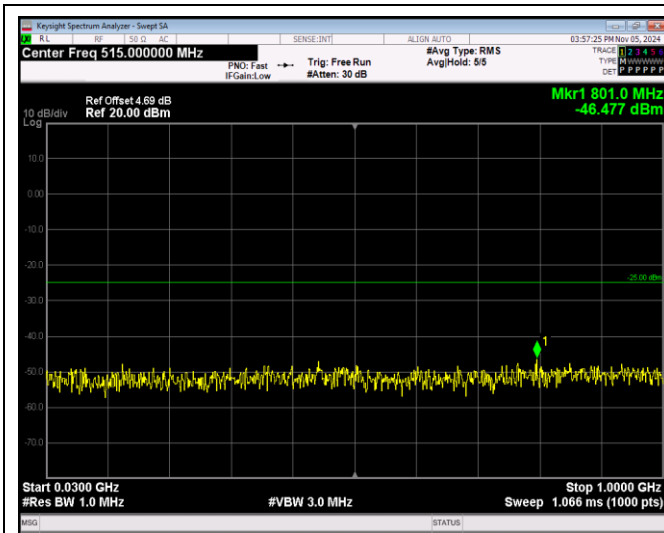
Band7-5MHz-16QAM-21100-1RB#0-Range1:30~1000 MHz
