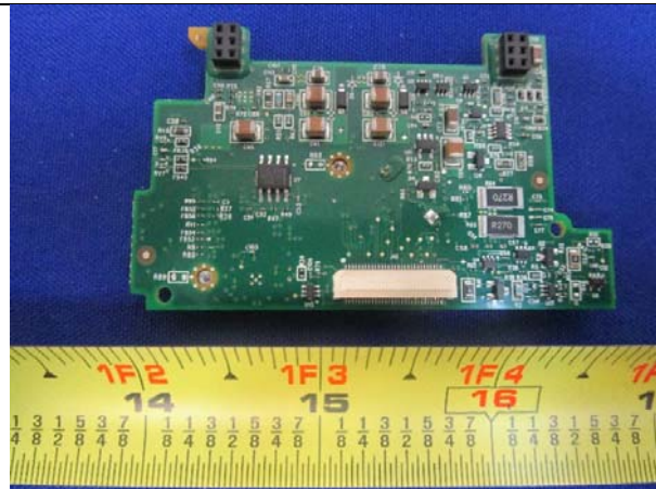
PCB1 Bottom View
