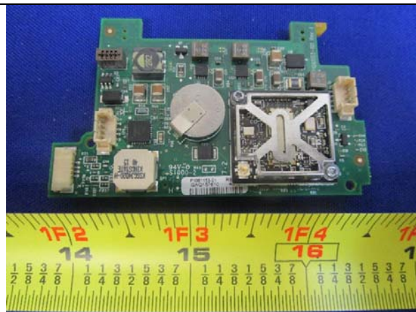
PCB1 Top View 2
