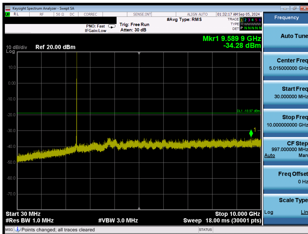
Plot 7-60. Conducted Spurious Plot MIMO ANT1 (802.11ax/be OFDMA – 26 Tones – Ch. 11)
