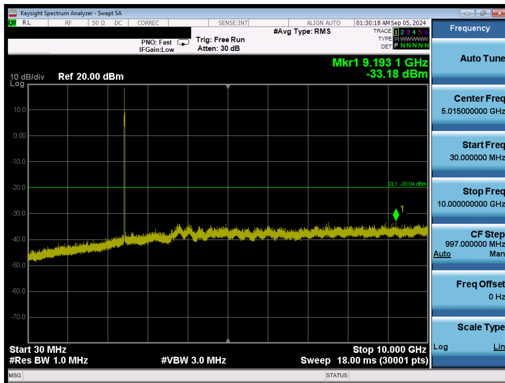
Plot 7-58. Conducted Spurious Plot MIMO ANT1 (802.11ax/be OFDMA – 26 Tones – Ch. 6)
