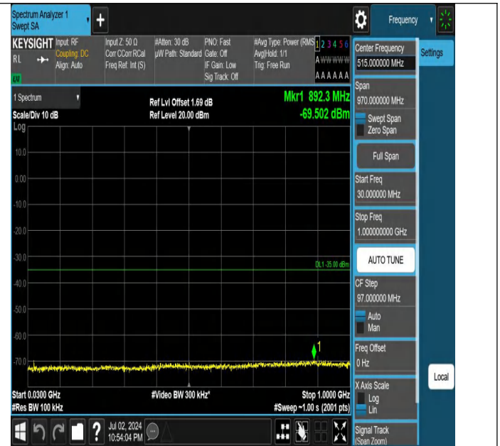
Band7-5MHz-QPSK-21100-1RB#24-30~1000-PASS
