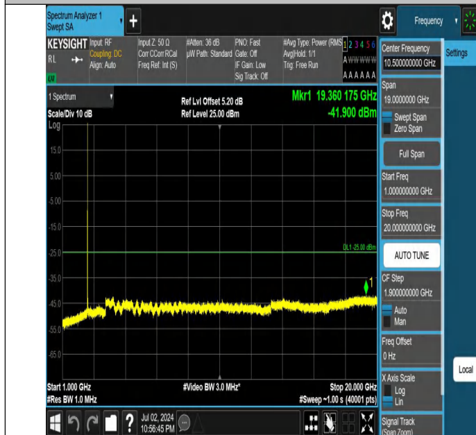
Band7-10MHz-21100-20800-1RB#49-1000~20000-PASS
