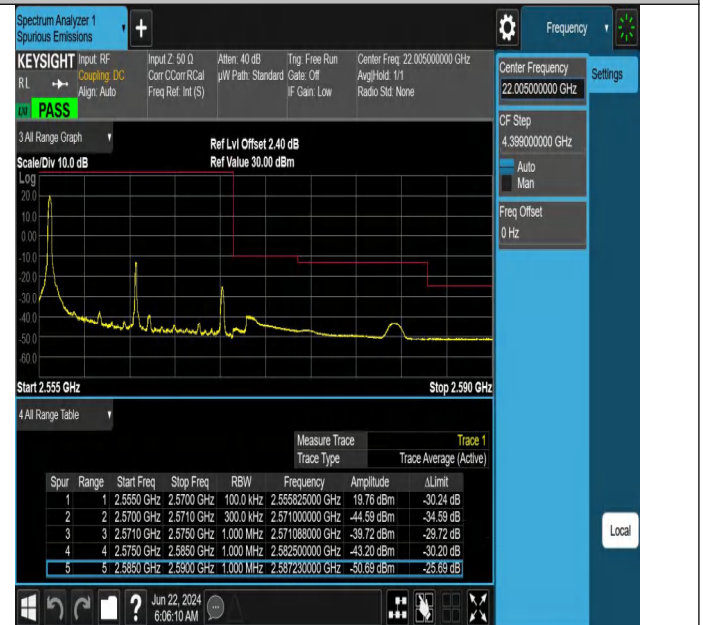
Band7-15MHz-QPSK-21375-1RB#0-PASS
