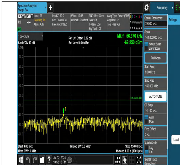
Band7-5MHz-QPSK-20775-1RB#0-0.009~0.15-PASS
