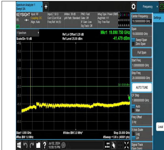
Band7-5MHz-QPSK-21425-1RB#24-1000~20000-PASS
