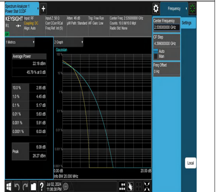
Band7-20MHz-16QAM-21100-27RB#0-PASS
