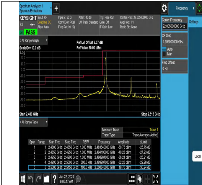
Band7-15MHz-QPSK-20825-1RB#0-PASS
