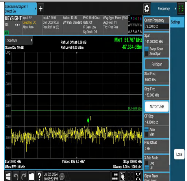
Band7-5MHz-QPSK-21100-1RB#24-0.009~0.15-PASS
