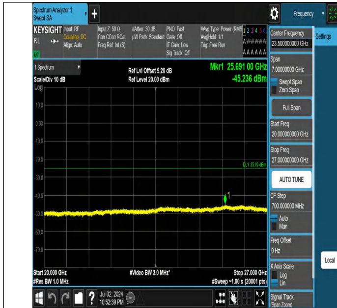
Band7-5MHz-QPSK-20775-1RB#0-20000~27000-PASS
