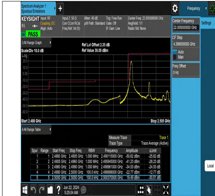
Band7-5MHz-QPSK-20775-1RB#0-PASS
