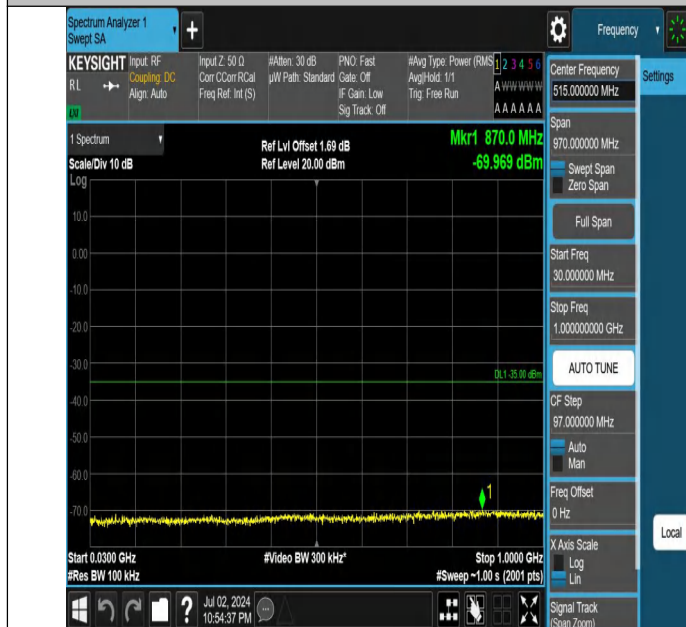
Band7-5MHz-QPSK-21425-1RB#0-30~1000-PASS
