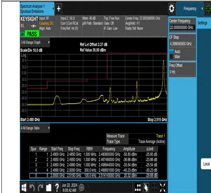
Band7-15MHz-QPSK-20825-1RB#74-PASS
