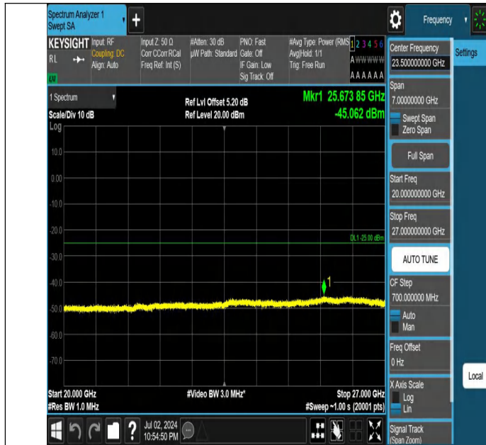
Band7-5MHz-QPSK-21425-1RB#0-20000~27000-PASS
