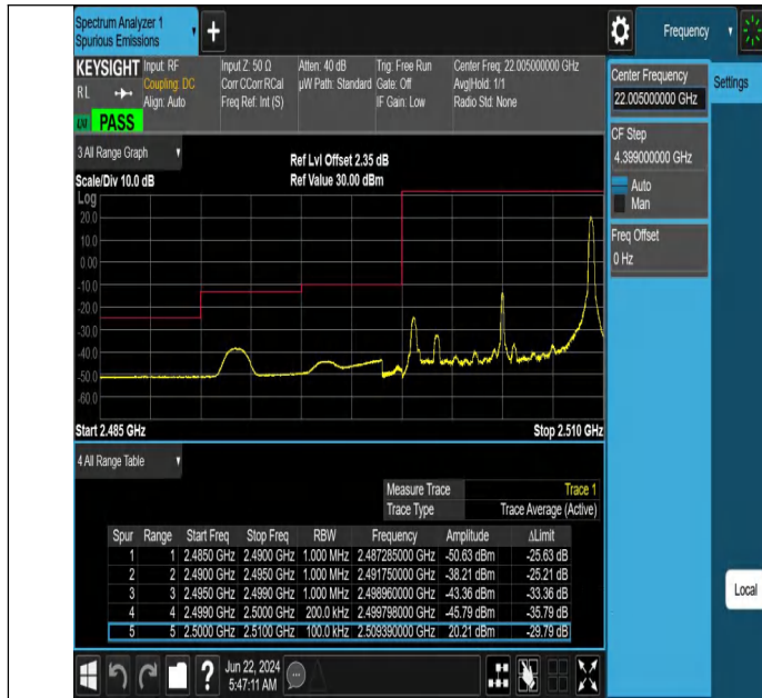
Band7-10MHz-QPSK-20800-1RB#49-PASS
