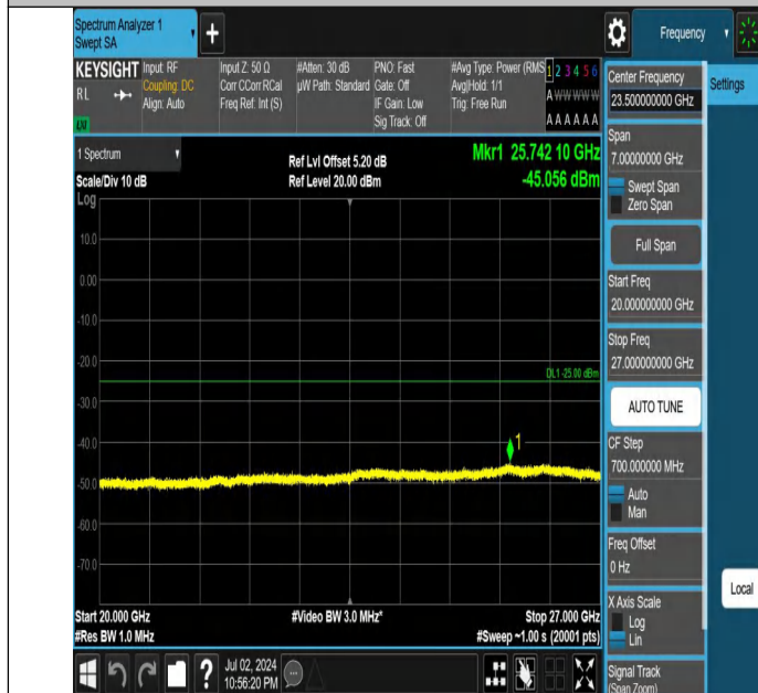
Band7-10MHz-21100-20800-1RB#0-20000~27000-PASS
