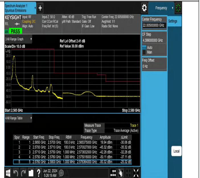
Band7-5MHz-QPSK-21425-1RB#0-PASS
