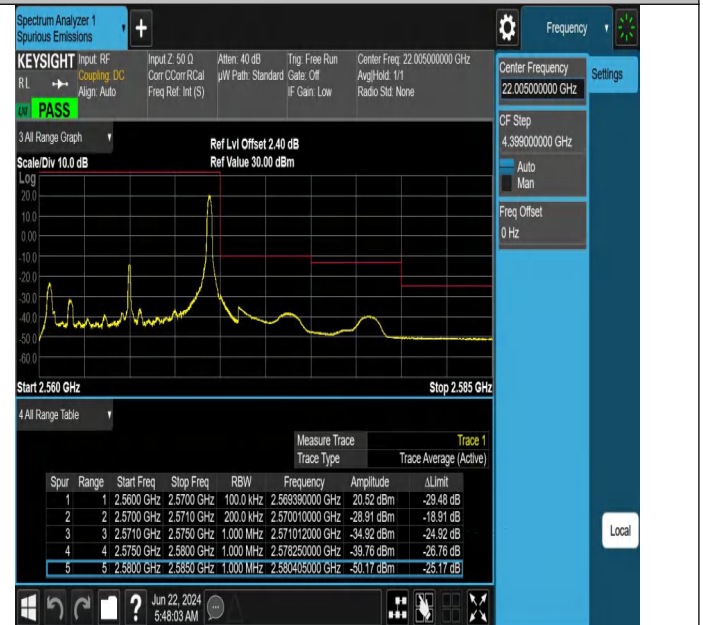
Band7-10MHz-QPSK-21400-1RB#49-PASS
