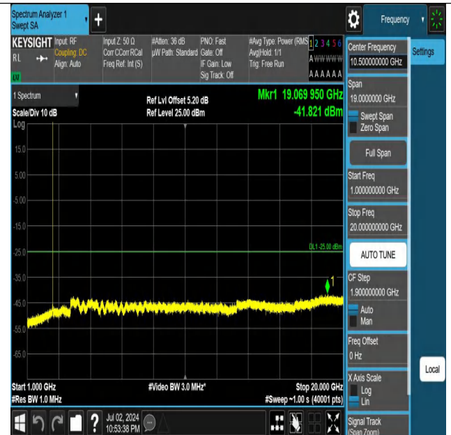
Band7-5MHz-QPSK-21100-1RB#0-1000~20000-PASS
