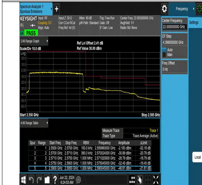
Band7-20MHz-QPSK-21350-100RB#0-PASS
