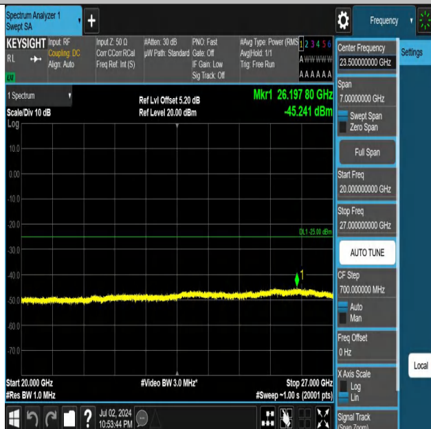
Band7-5MHz-QPSK-21100-1RB#0-20000~27000-PASS
