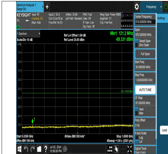
Band7-10MHz-21100-20800-1RB#0-30~1000-PASS
