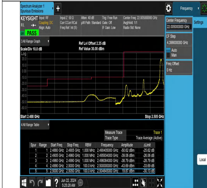
Band7-5MHz-QPSK-20775-1RB#24-PASS
