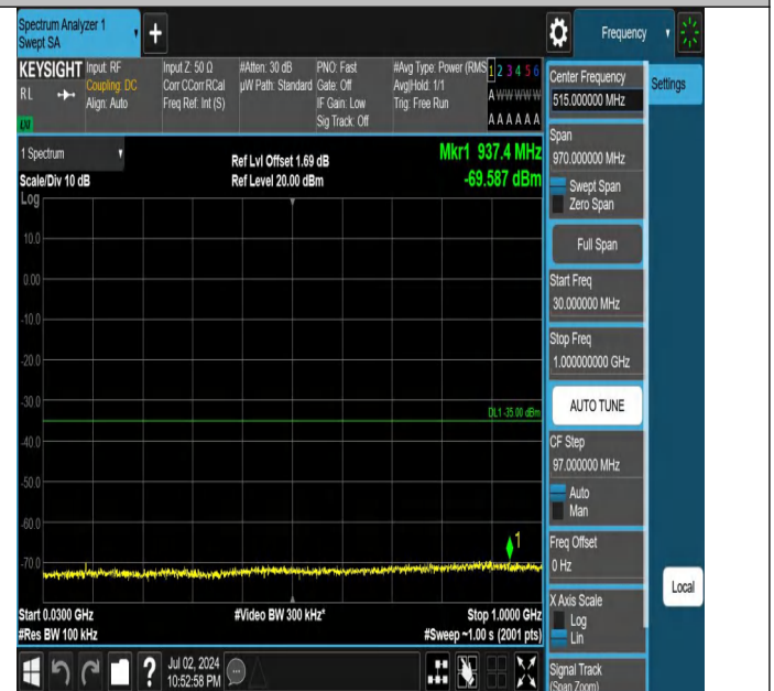
Band7-5MHz-QPSK-20775-1RB#24-30~1000-PASS
