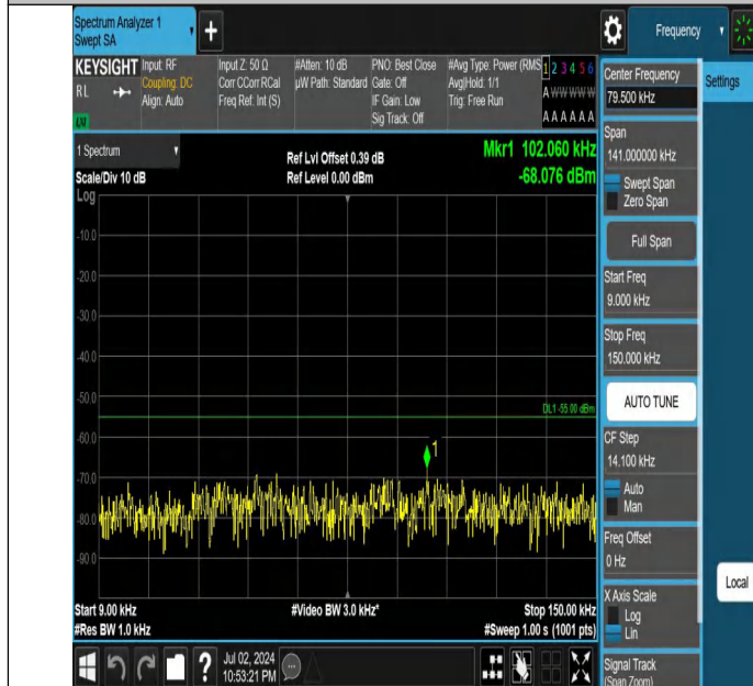
Band7-5MHz-QPSK-21100-1RB#0-0.009~0.15-PASS
