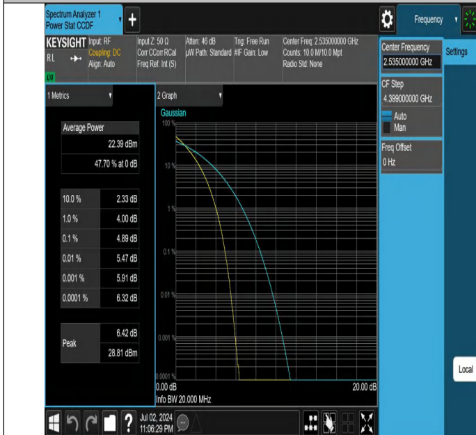
Band7-20MHz-QPSK-21100-100RB#0-PASS
