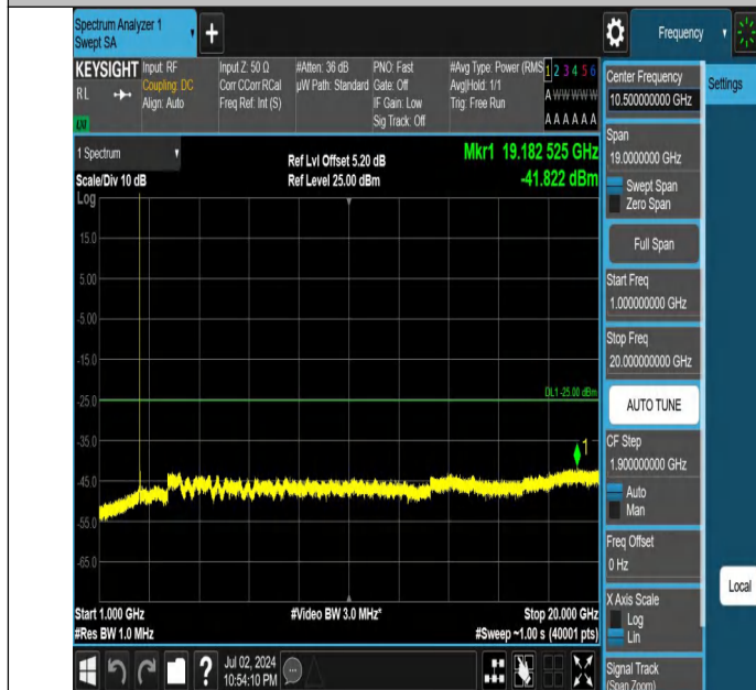
Band7-5MHz-QPSK-21100-1RB#24-1000~20000-PASS
