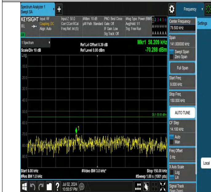
Band7-10MHz-21100-20800-1RB#0-0.009~0.15-PASS
