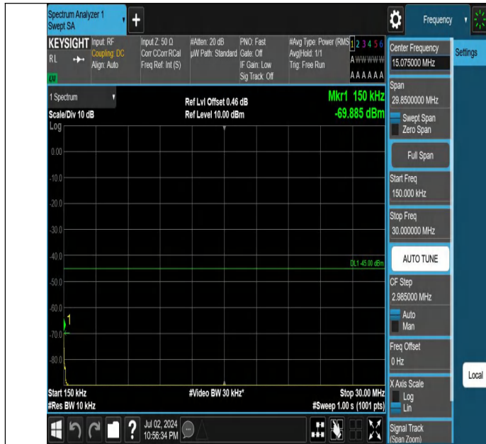
Band7-10MHz-21100-20800-1RB#49-0.15~30-PASS
