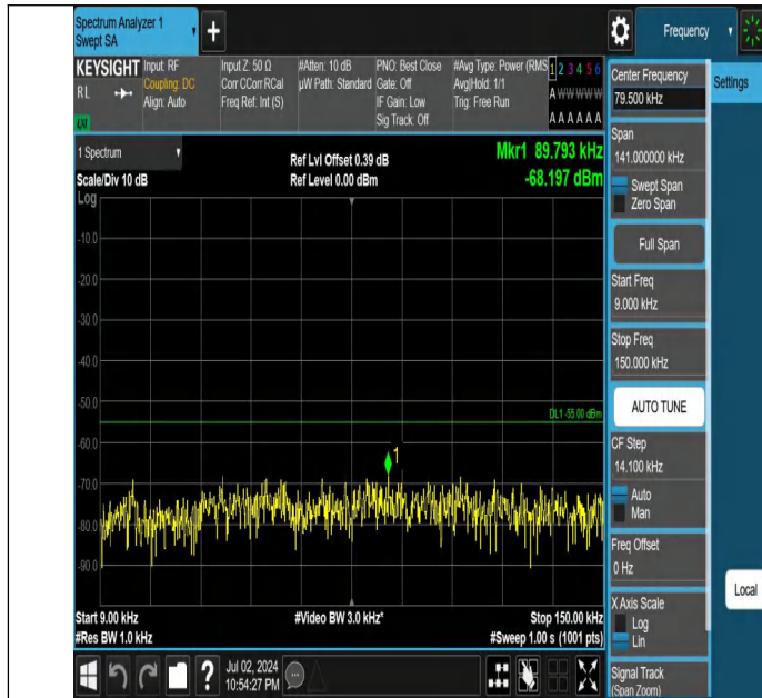
Band7-5MHz-QPSK-21425-1RB#0-0.009~0.15-PASS
