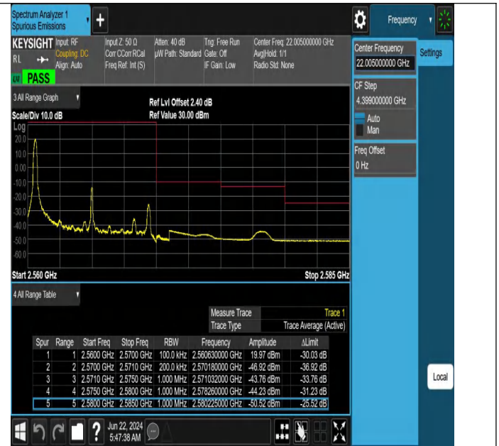
Band7-10MHz-QPSK-21400-1RB#0-PASS
