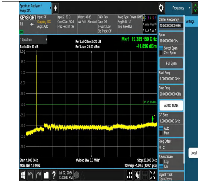
Band7-5MHz-QPSK-20775-1RB#24-1000~20000-PASS
