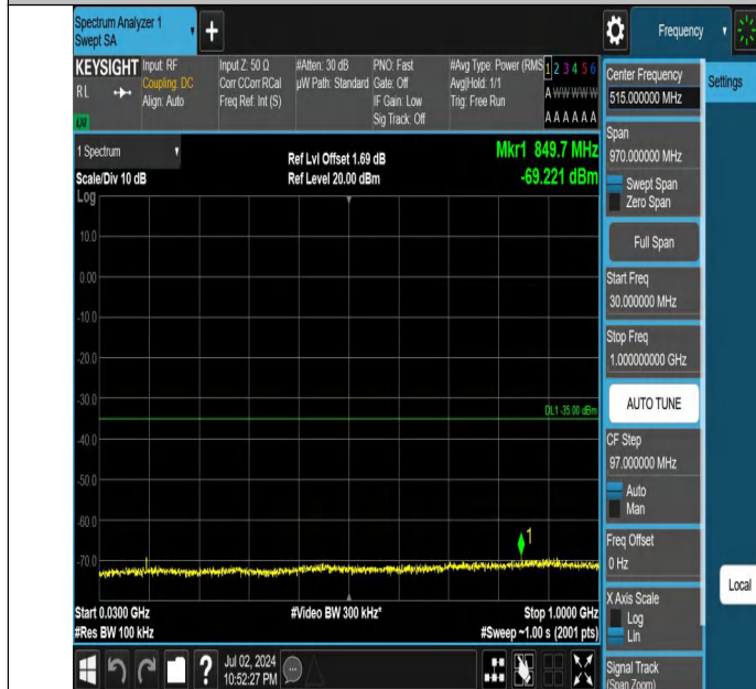
Band7-5MHz-QPSK-20775-1RB#0-30~1000-PASS
