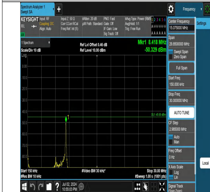
Band7-5MHz-QPSK-21425-1RB#24-0.15~30-PASS
