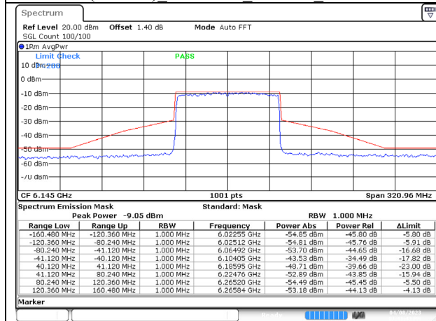
802.11ax (80MHz) 6145MHz Chain A NSS-1
