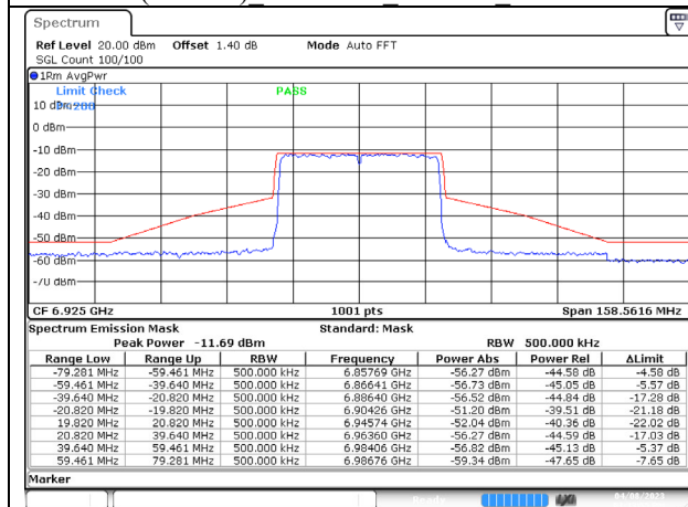
802.11ax (40MHz) 6925MHz Chain A NSS-1
