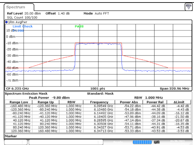
802.11ax (80MHz) 6225MHz Chain B NSS-1
