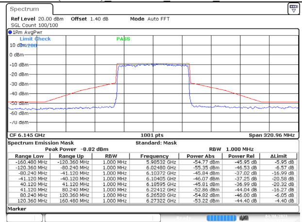
802.11ax (80MHz) 6145MHz Chain B NSS-1
