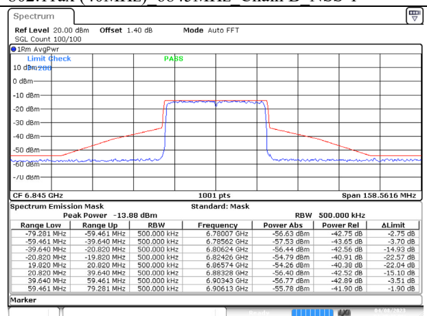
802.11ax (40MHz) 6845MHz Chain B NSS-1
