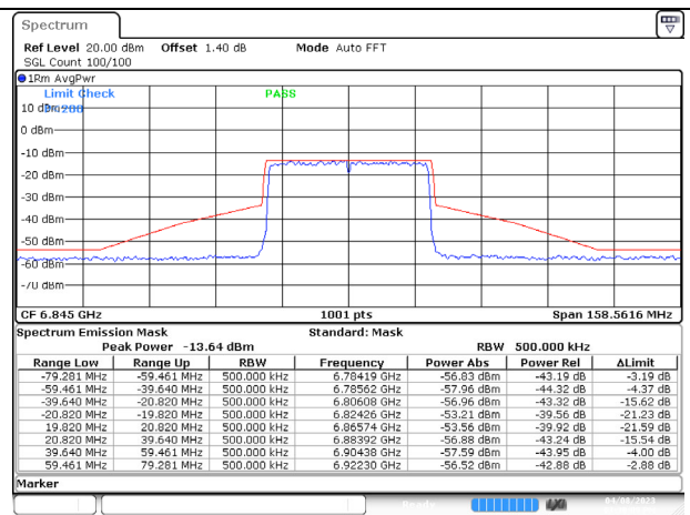
802.11ax (40MHz) 6845MHz Chain B NSS-1
