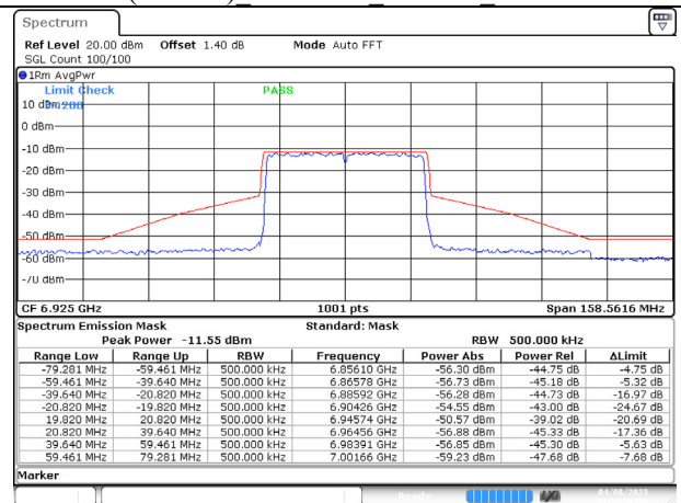
802.11ax (40MHz) 6925MHz Chain B NSS-1
