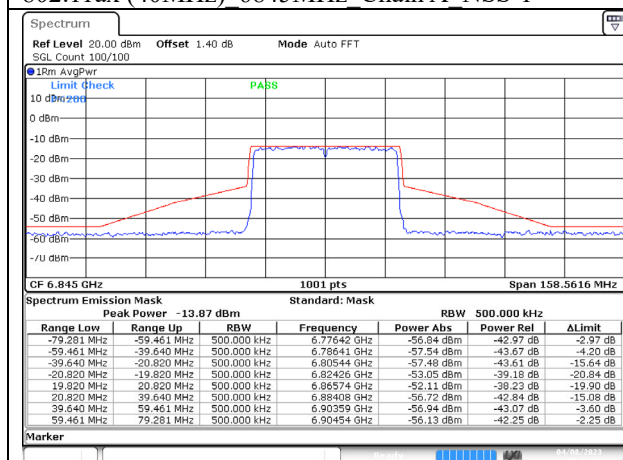
802.11ax (40MHz) 6845MHz Chain A NSS-1
