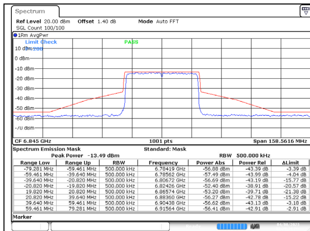
802.11ax (40MHz) 6845MHz Chain A NSS-1
