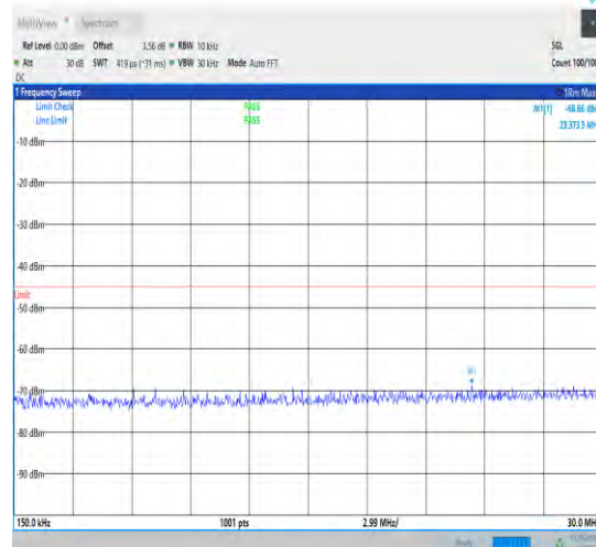
1-N41-30-100-L-1-DFT-PI2BPSK-Inner_1RB_Left-1 @1-0.15-30-Ant1-23.37--68.66--45-PASS
