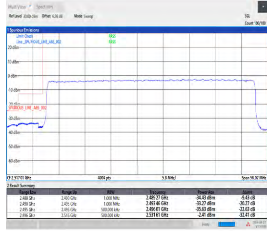
1-N41-30-50-L-3-DFT-PI2BPSK-Outer_Full-128@0- Ant1-1--PASS-see graph
