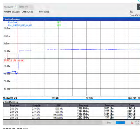
1-N41-30-70-L-6-CP-QPSK-Outer_Full-189@0-Ant 1-1--PASS-see graph
