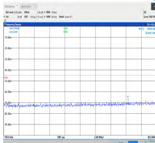
1-N41-30-100-M-1-DFT-PI2BPSK-Inner_1RB_Left-1 @1-0.15-30-Ant1-24.42--68.00--45-PASS
