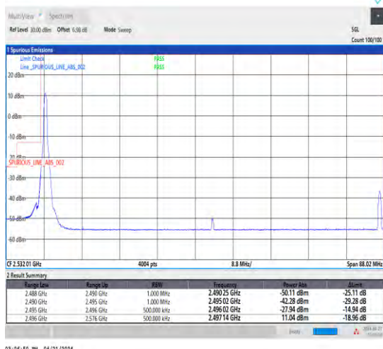
1-N41-30-80-L-1-DFT-PI2BPSK-Edge_1RB_Left-1@0 -Ant1-1--PASS-see graph
