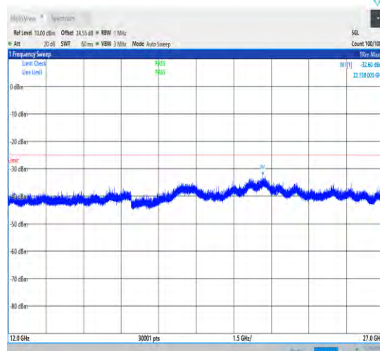
1-N41-30-100-M-1-DFT-PI2BPSK-Inner_1RB_Left-1 @1-12000-27000-Ant1-22158.00--32.60--25-PASS
