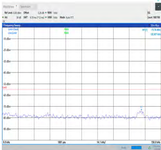
1-N41-30-100-H-1-DFT-PI2BPSK-Inner_1RB_Left-1 @1-0.009-0.15-Ant1-0.13--73.78--55-PASS
