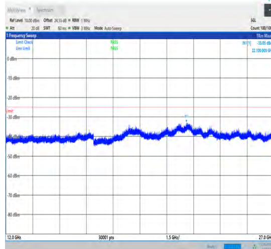
1-N41-30-100-H-1-DFT-PI2BPSK-Inner_1RB_Left-1 @1-12000-27000-Ant1-22100.00--33.05--25-PASS
