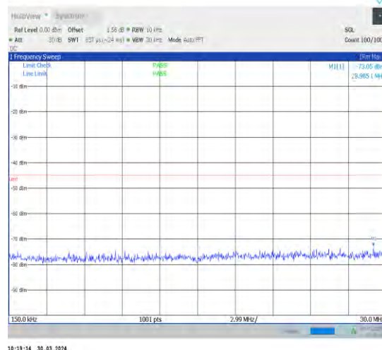
1-N41-30-100-L-1-DFT-PI2BPSK-Inner_1RB_Left-1 @1-0.15-30-Ant1-29.61--73.05--45-PASS
