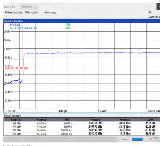
1-N41-30-60-L-3-DFT-PI2BPSK-Outer_Full-162@0- Ant1-1--PASS-see graph
