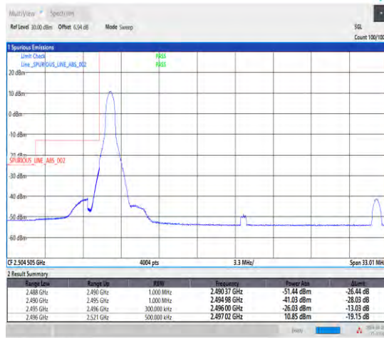
1-N41-30-25-L-4-CP-QPSK-Edge_1RB_Left-1@0-Ant1-1--PASS-see graph
