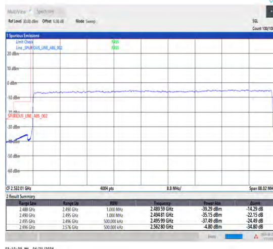
1-N41-30-80-L-3-DFT-PI2BPSK-Outer_Full-216@0- Ant1-1--PASS-see graph
