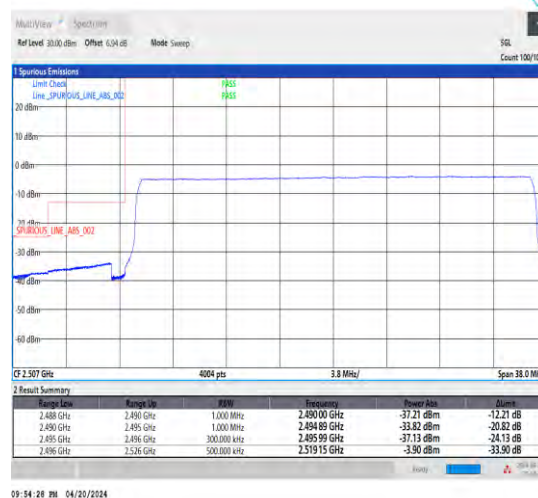
1-N41-30-30-L-6-CP-QPSK-Outer_Full-78@0-Ant1-1--PASS-see graph
