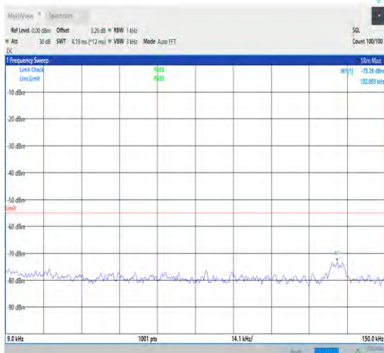
1-N41-30-100-M-1-DFT-PI2BPSK-Inner_1RB_Left-1 @1-0.009-0.15-Ant1-0.13--73.29--55-PASS
