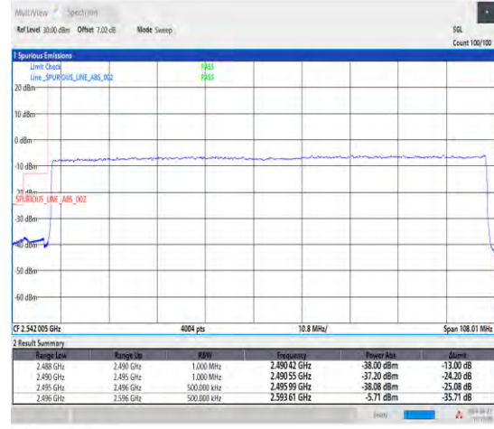
1-N41-30-100-L-3-DFT-PI2BPSK-Outer_Full-270@ 0-Ant1-1--PASS-see graph
