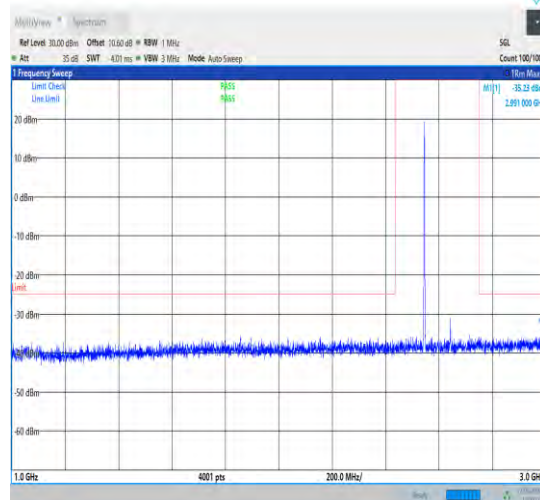
1-N41-30-100-M-1-DFT-PI2BPSK-Inner_1RB_Left-1 @1-1000-3000-Ant1-2991.00--35.23--25-PASS
