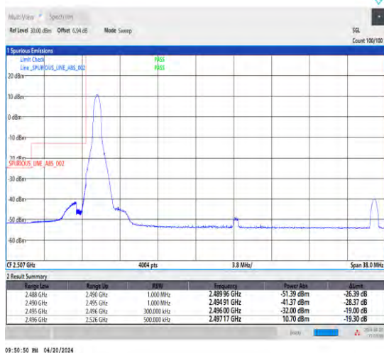
1-N41-30-30-L-4-CP-QPSK-Edge_1RB_Left-1@0-Ant1-1--PASS-see graph
