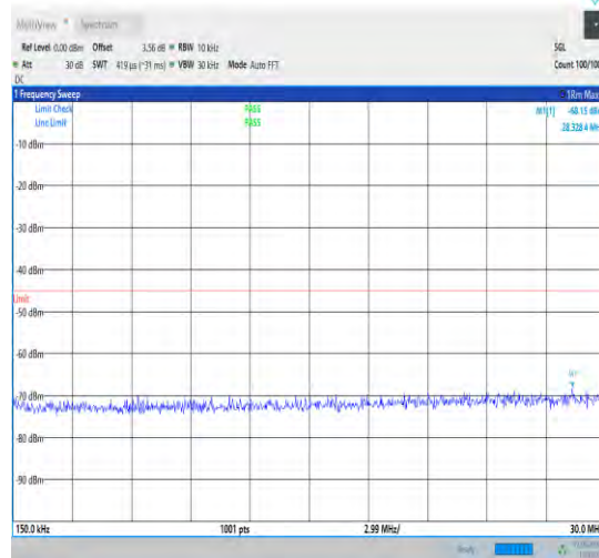
1-N41-30-100-H-1-DFT-PI2BPSK-Inner_1RB_Left-1 @1-0.15-30-Ant1-28.33--68.15--45-PASS
