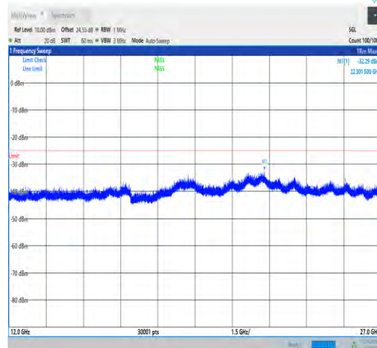
1-N41-30-100-L-1-DFT-PI2BPSK-Inner_1RB_Left-1 @1-12000-27000-Ant1-22301.50--32.29--25-PASS
