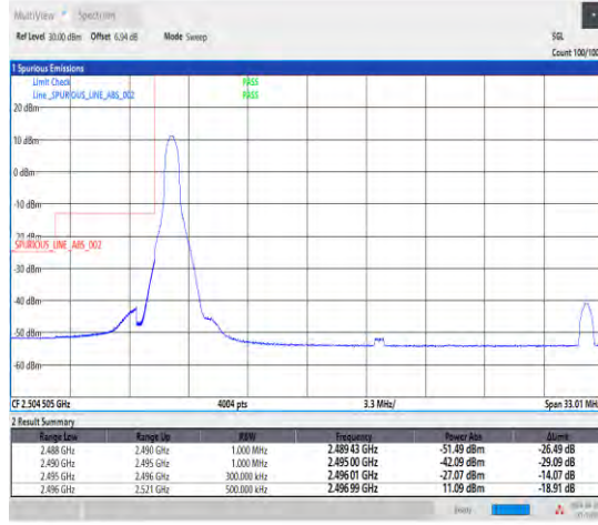
1-N41-30-25-L-1-DFT-PI2BPSK-Edge_1RB_Left-1@0-Ant1-1--PASS-see graph
