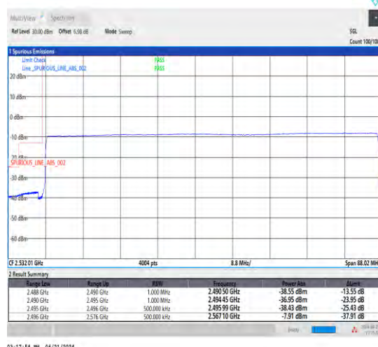
1-N41-30-80-L-6-CP-QPSK-Outer_Full-217@0-Ant 1-1--PASS-see graph
