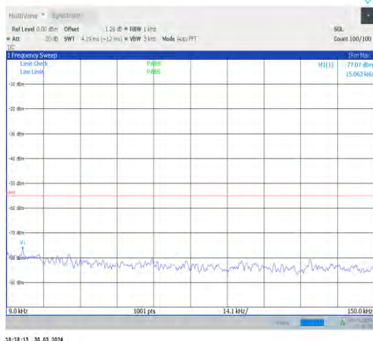
1-N41-30-100-L-1-DFT-PI2BPSK-Inner_1RB_Left-1 @1-0.009-0.15-Ant1-0.01--77.07--55-PASS
