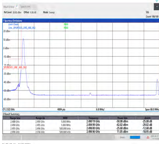
1-N41-30-60-L-1-DFT-PI2BPSK-Edge_1RB_Left-1@0 -Ant1-1--PASS-see graph
