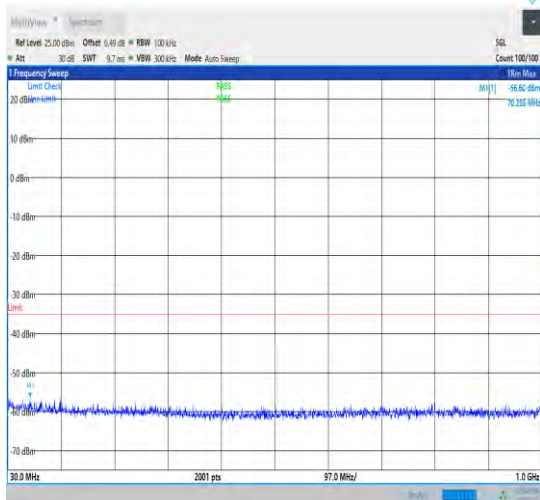
1-N41-30-100-M-1-DFT-PI2BPSK-Inner_1RB_Left-1 @1-30-1000-Ant1-70.26--56.60--35-PASS
