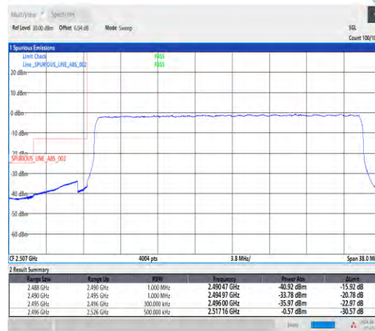
1-N41-30-30-L-3-DFT-PI2BPSK-Outer_Full-75@0-Ant1-1--PASS-see graph
