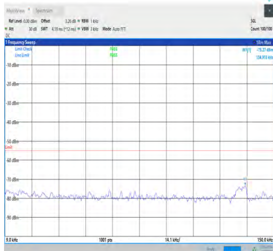
1-N41-30-100-L-1-DFT-PI2BPSK-Inner_1RB_Left-1 @1-0.009-0.15-Ant1-0.13--73.27--55-PASS
