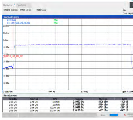
1-N41-30-90-L-3-DFT-PI2BPSK-Outer_Full-240@0-Ant1-1--PASS-see graph
