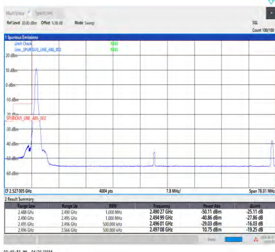
1-N41-30-70-L-4-CP-QPSK-Edge_1RB_Left-1@0-Ant 1-1--PASS-see graph
