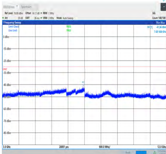
1-N41-30-100-L-1-DFT-PI2BPSK-Inner_1RB_Left-1 @1-3000-12000-Ant1-7431.60--41.34--25-PASS
