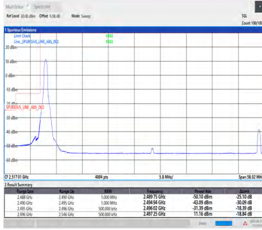
1-N41-30-50-L-1-DFT-PI2BPSK-Edge_1RB_Left-1@0 -Ant1-1--PASS-see graph
