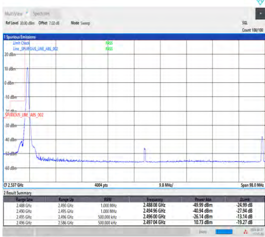
1-N41-30-90-L-4-CP-QPSK-Edge_1RB_Left-1@0-Ant1-1--PASS-see graph
