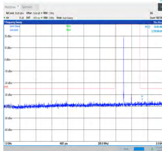
1-N41-30-100-L-1-DFT-PI2BPSK-Inner_1RB_Left-1 @1-1000-3000-Ant1-2729.50--34.89--25-PASS
