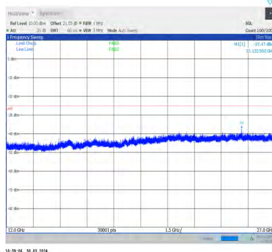
1-N41-30-100-M-1-DFT-PI2BPSK-Inner_1RB_Left-1 @1-12000-27000-Ant1-19449.50--37.47--25-PASS
