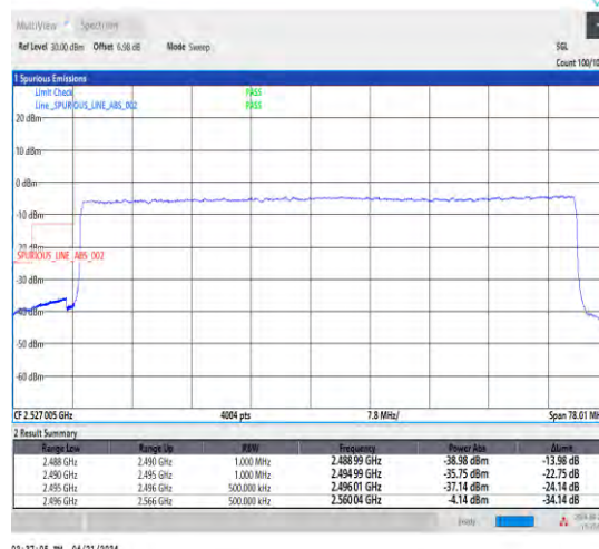
1-N41-30-70-L-3-DFT-PI2BPSK-Outer_Full-180@0- Ant1-1--PASS-see graph
