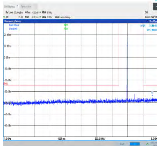
1-N41-30-100-H-1-DFT-PI2BPSK-Inner_1RB_Left-1 @1-1000-3000-Ant1-2917.00--34.66--25-PASS
