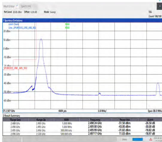
1-N41-30-30-L-1-DFT-PI2BPSK-Edge_1RB_Left-1@0-Ant1-1--PASS-see graph
