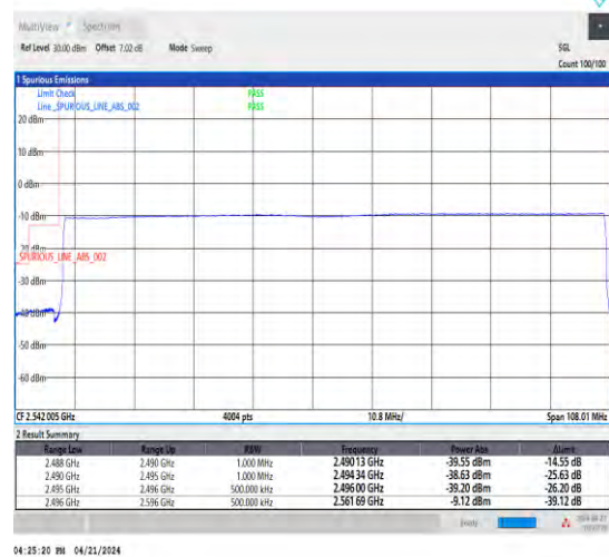
1-N41-30-100-L-6-CP-QPSK-Outer_Full-273@0-Ant1-1--PASS-see graph
