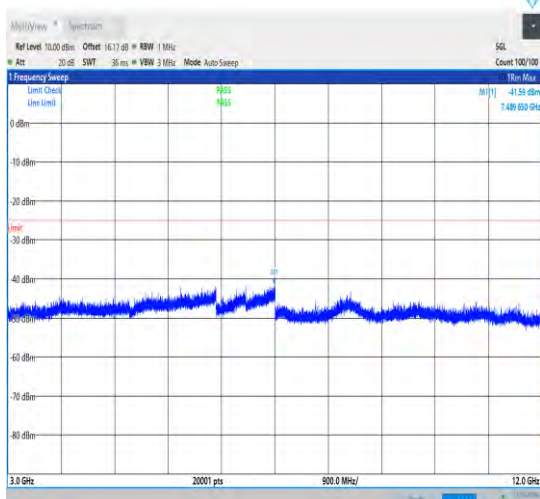
1-N41-30-100-M-1-DFT-PI2BPSK-Inner_1RB_Left-1 @1-3000-12000-Ant1-7489.65--41.59--25-PASS
