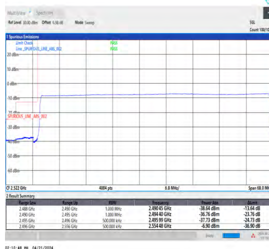
1-N41-30-60-L-6-CP-QPSK-Outer_Full-162@0-Ant 1-1--PASS-see graph
