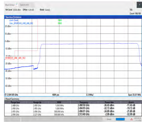
1-N41-30-25-L-6-CP-QPSK-Outer_Full-65@0-Ant1-1--PASS-see graph
