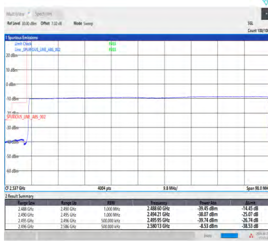
1-N41-30-90-L-6-CP-QPSK-Outer_Full-245@0-Ant1-1--PASS-see graph
