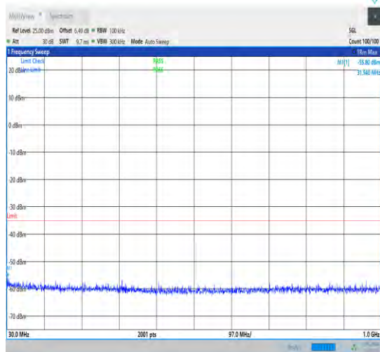
1-N41-30-100-L-1-DFT-PI2BPSK-Inner_1RB_Left-1 @1-30-1000-Ant1-31.94--55.80--35-PASS
