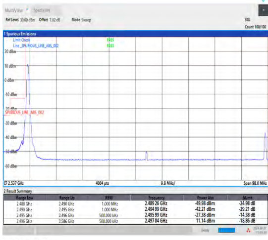
1-N41-30-90-L-1-DFT-PI2BPSK-Edge_1RB_Left-1@0-Ant1-1--PASS-see graph
