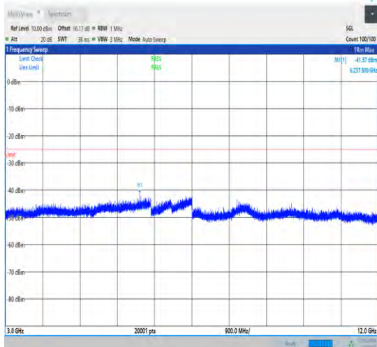
1-N41-30-100-H-1-DFT-PI2BPSK-Inner_1RB_Left-1 @1-3000-12000-Ant1-6237.30--41.37--25-PASS
