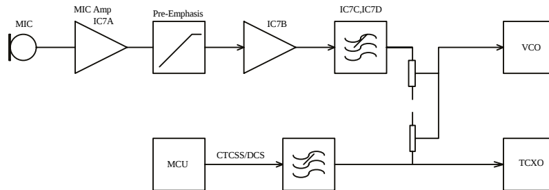
Figure 7 Transmitter Audio Circuit
