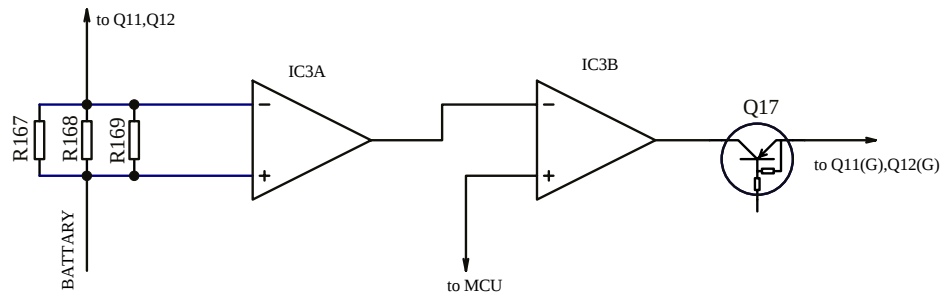
Figure 6 APC Circuit
