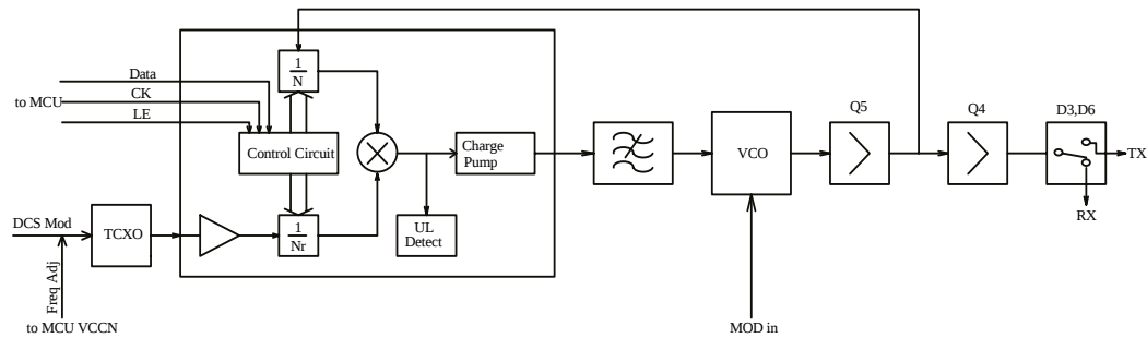
Figure 8 Frequency Synthesizer
