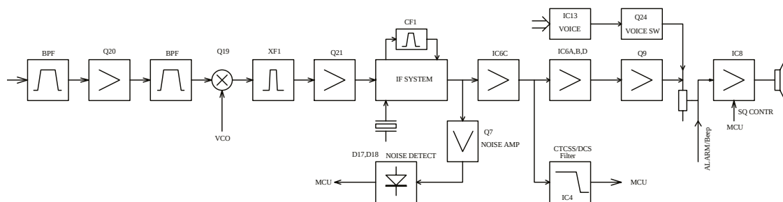
Figure 2 Receiver Illustration
