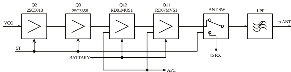
Figure 5 Amplifier and Antenna Switch Diagram
