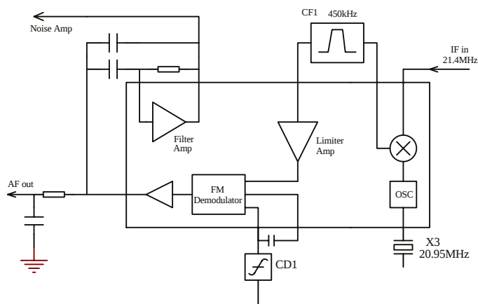
Figure 3 IF System
