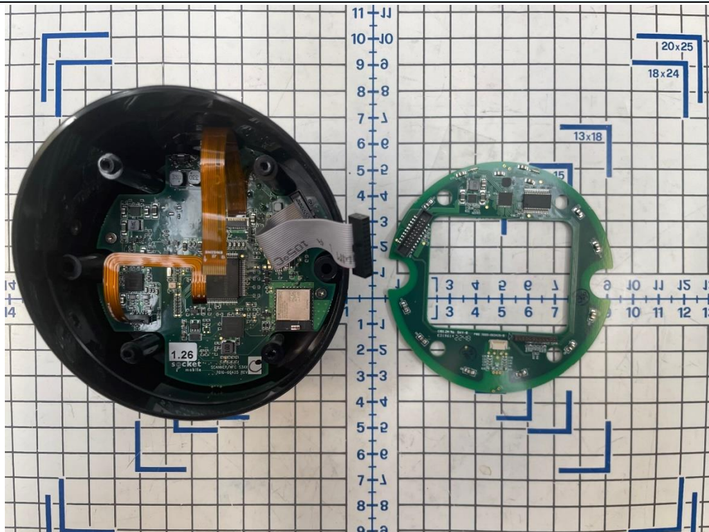
Internal View 4
