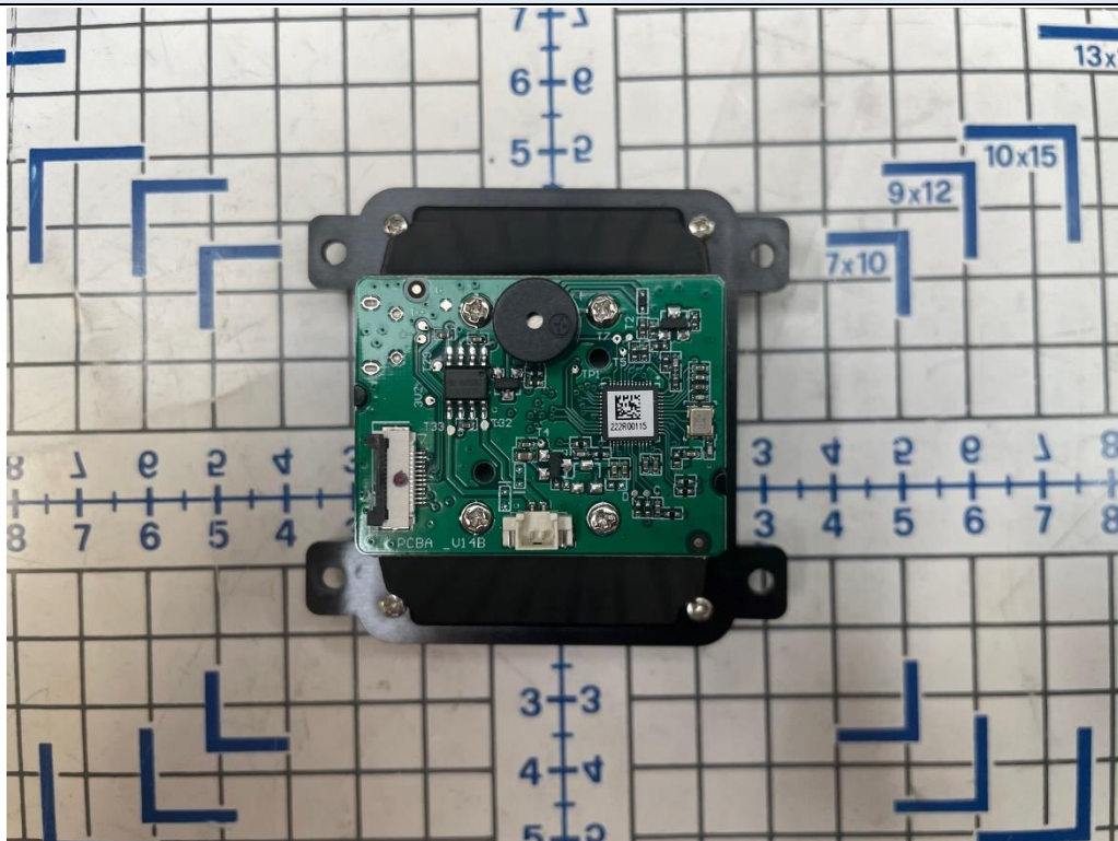
QR Code Reader Board Bottom View
