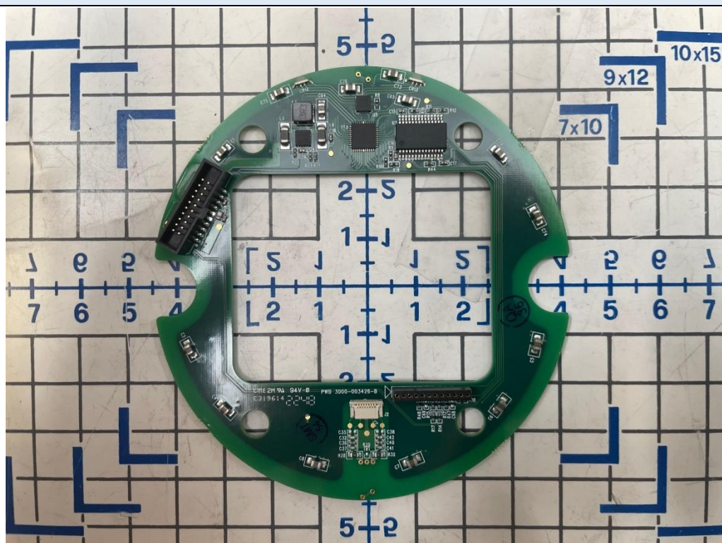
LED / ANT Board Bottom View
