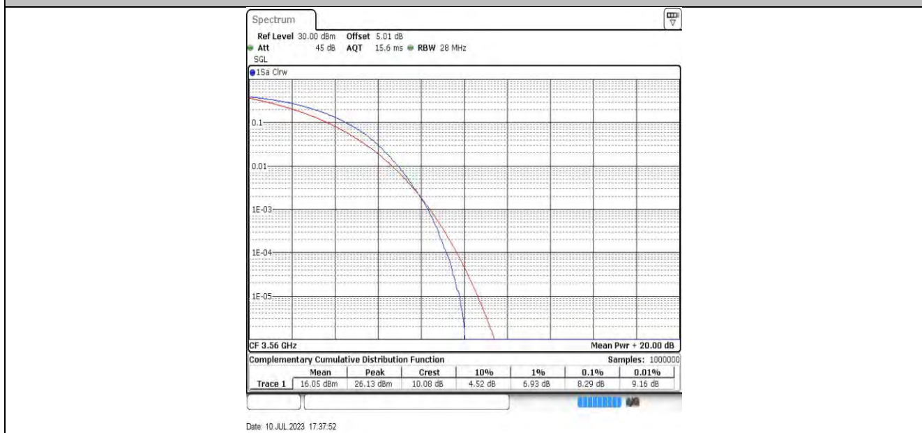
20MHz-55340 256QAM
