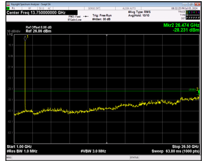
Band41-5MHz-16QAM-40640-1RB#0-Range2:1000~26500MHz
