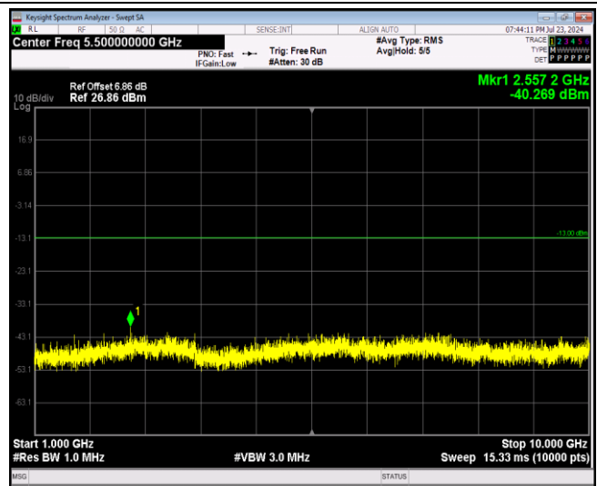
Band5-1.4MHz-64QAM-20525-1RB#0-Range2:1000~10000MHz
