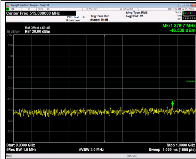
Band7-20MHz-64QAM-20850-1RB#0-Range1:30~1000MHz
