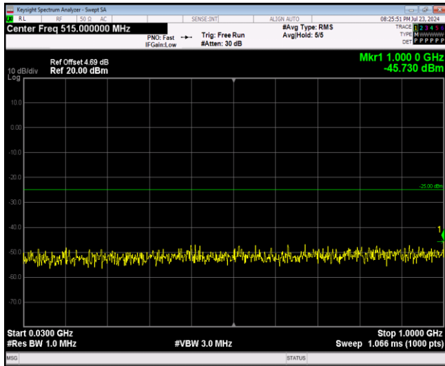
Band7-20MHz-64QAM-21350-1RB#0-Range1:30~1000MHz
