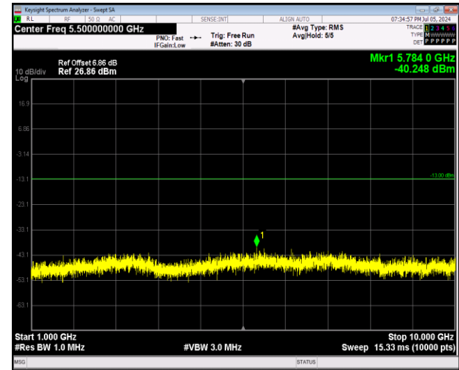
Band5-10MHz-64QAM-20450-1RB#0-Range2:1000~10 00MHz
