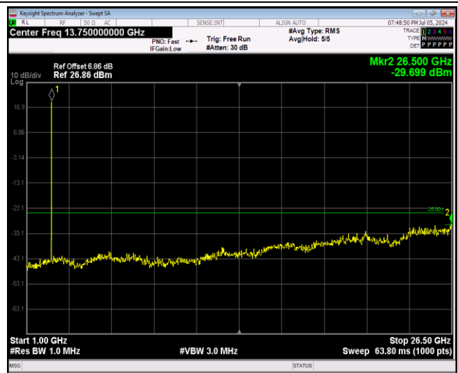
Band7-5MHz-16QAM-21100-1RB#0-Range2:1000~265 00MHz
