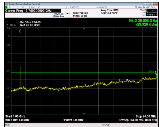
Band41-5MHz-16QAM-41215-1RB#0-Range2:1000~26500MHz
