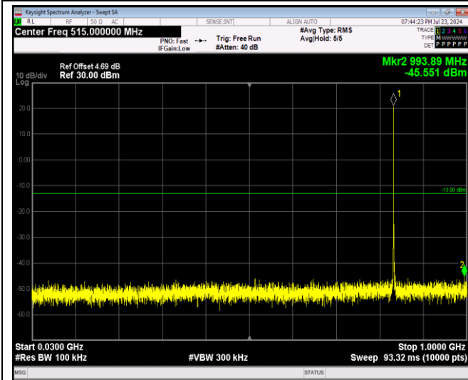
Band5-1.4MHz-64QAM-20643-1RB#0-Range1:30~1000MHz
