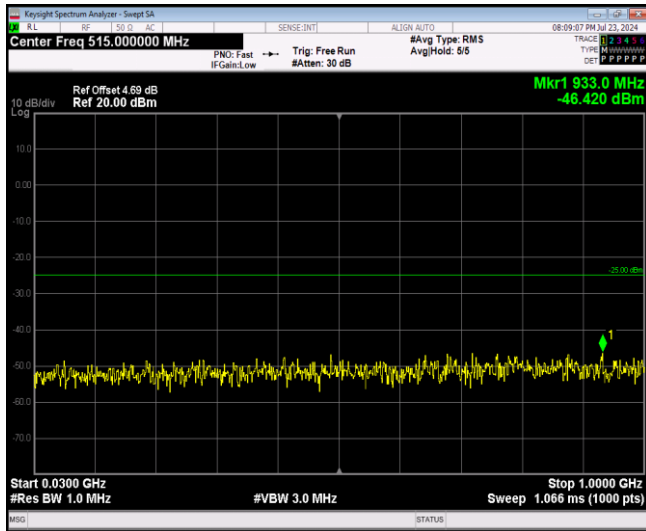
Band7-5MHz-64QAM-21100-1RB#0-Range1:30~100 0MHz
