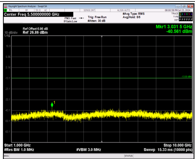
Band5-10MHz-64QAM-20600-1RB#0-Range2:1000~10000MHz
