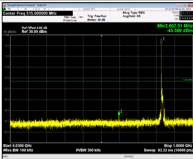
Band5-10MHz-QPSK-20600-1RB#0-Range1:30~100 00MHz
