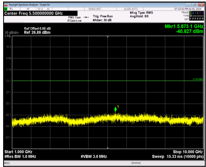
Band5-10MHz-16QAM-20525-1RB#0-Range2:1000~10000MHz
