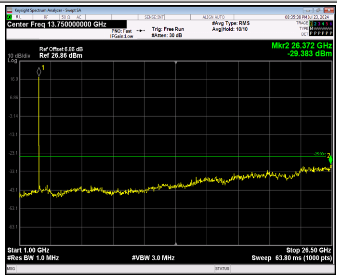
Band41-5MHz-64QAM-40640-1RB#0-Range2:1000~26500MHz
