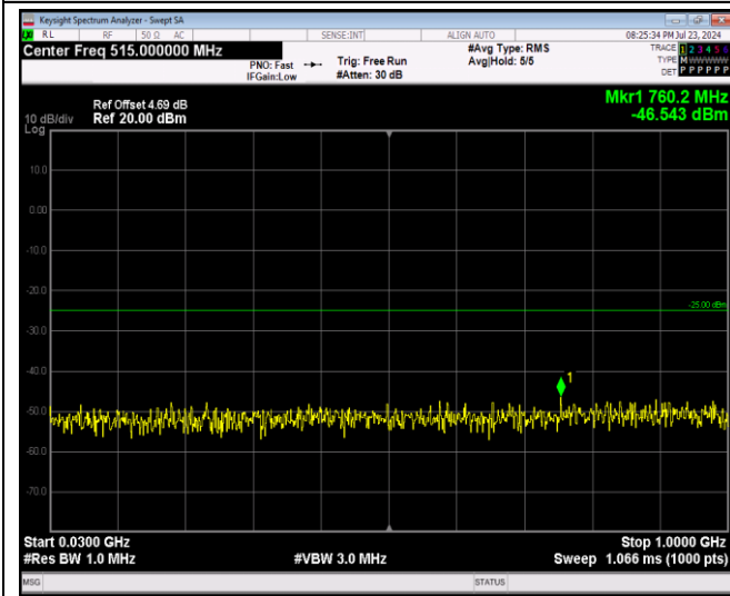
Band7-20MHz-64QAM-20850-1RB#0-Range1:30~1000MHz
