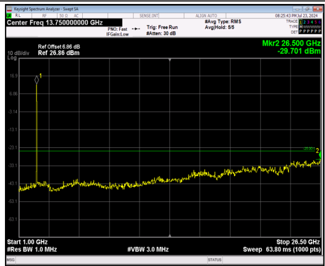
Band7-20MHz-64QAM-20850-1RB#0-Range2:1000~26500MHz
