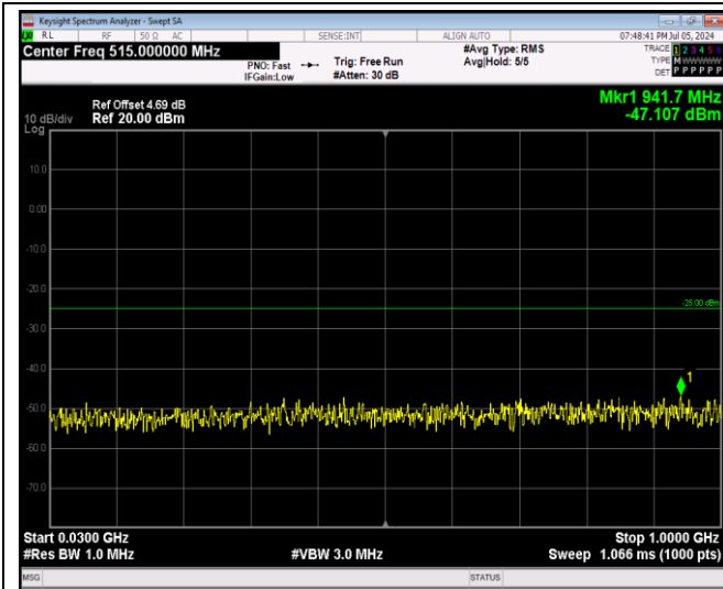
Band7-5MHz-16QAM-21100-1RB#0-Range1:30~100 OMHz
