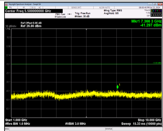
Band5-10MHz-64QAM-20525-1RB#0-Range2:1000~10 00MHz
