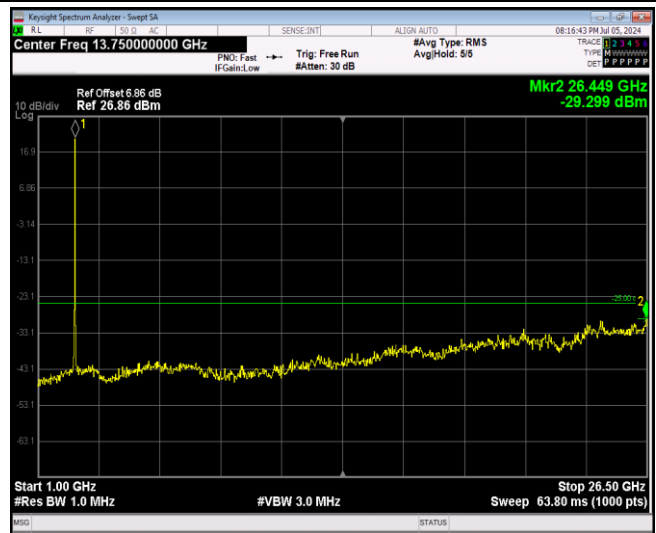
Band7-20MHz-64QAM-20850-1RB#0-Range2:1000~26500MHz
