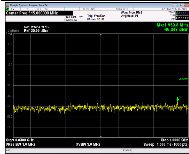
Band7-5MHz-16QAM-21425-1RB#0-Range1:30~100 OMHz
