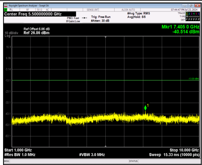
Band5-1.4MHz-64QAM-20643-1RB#0-Range2:1000~10000MHz
