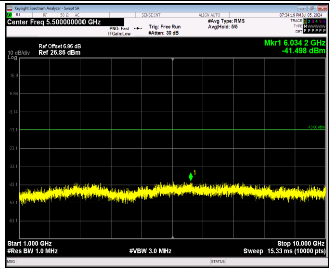
Band5-10MHz-16QAM-20525-1RB#0-Range2:1000~10000MHz
