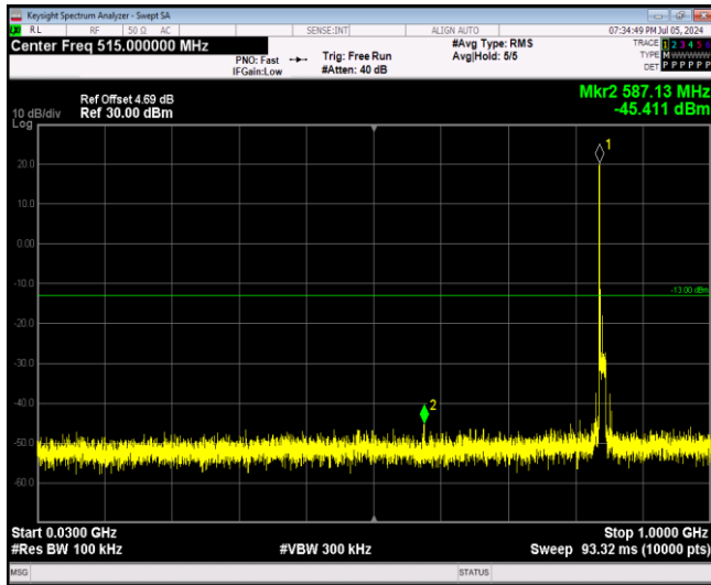
Band5-10MHz-64QAM-20450-1RB#0-Range1:30~10 00MHz
