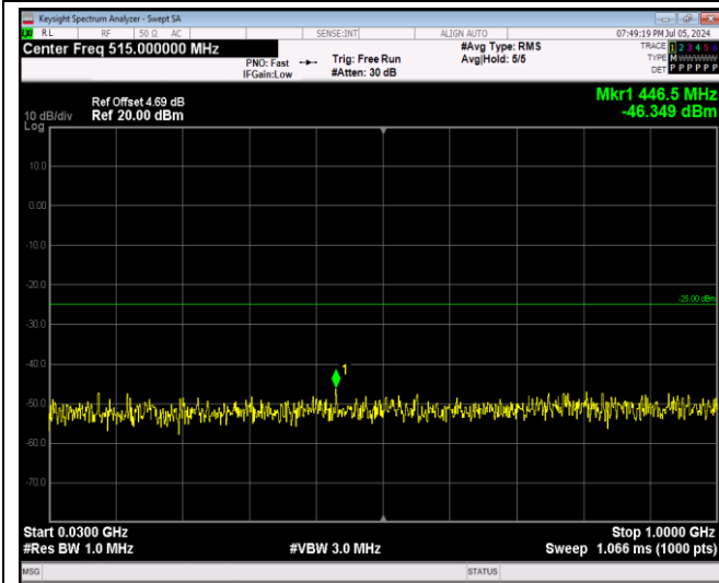
Band7-5MHz-16QAM-21425-1RB#0-Range1:30~100 OMHz
