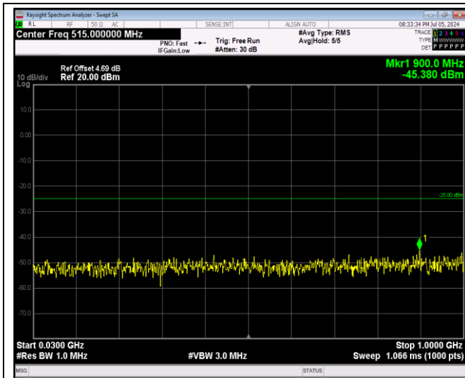
Band41-5MHz-64QAM-40065-1RB#0-Range1:30~1000MHz
