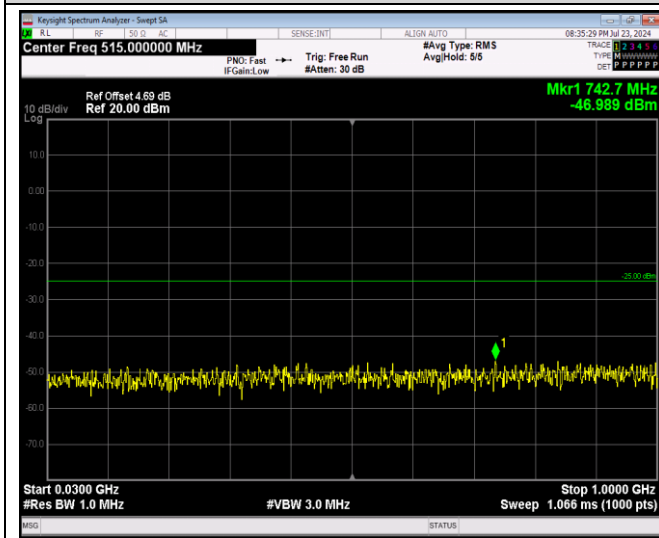
Band41-5MHz-64QAM-40640-1RB#0-Range1:30~1000MHz
