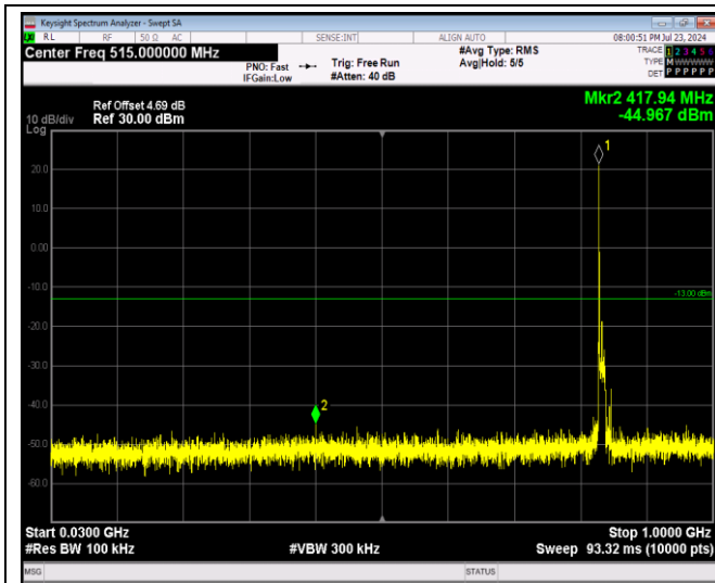
Band5-10MHz-64QAM-20600-1RB#0-Range1:30~1000MHz
