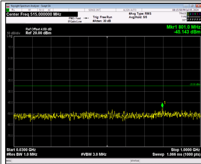
Band7-20MHz-16QAM-21350-1RB#0-Range1:30~1000MHz
