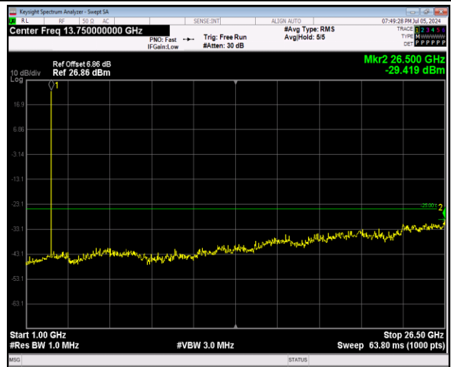
Band7-5MHz-16QAM-21425-1RB#0-Range2:1000~265 00MHz
