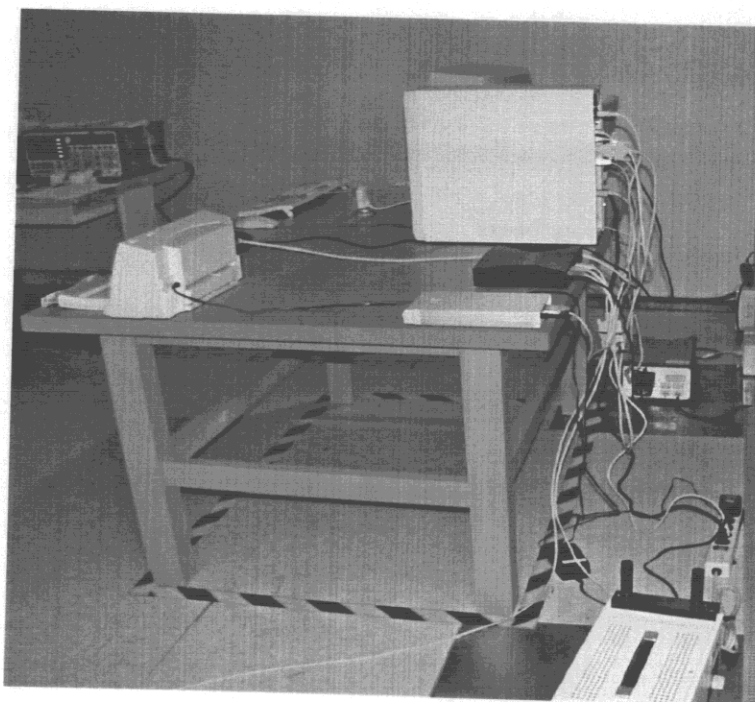
Mode 1 :Back View of Conducted Test ( Maximum Testing Configuration)
