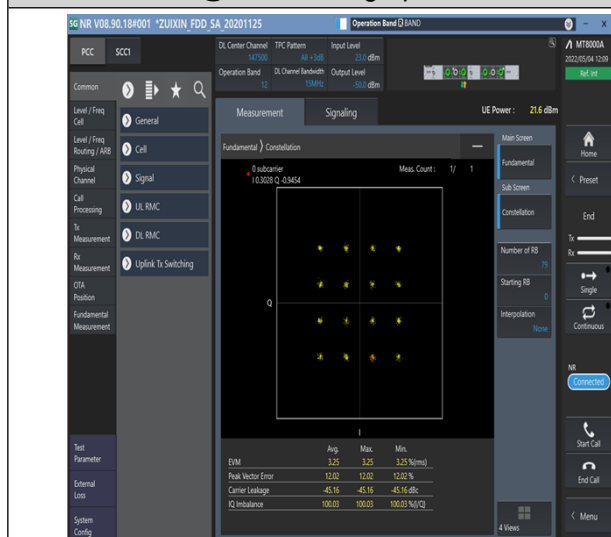
1-N12-PC3-15-15-M-7-CP-16QAM-Outer_Full-79@0-Ant1-see graph-PASS
