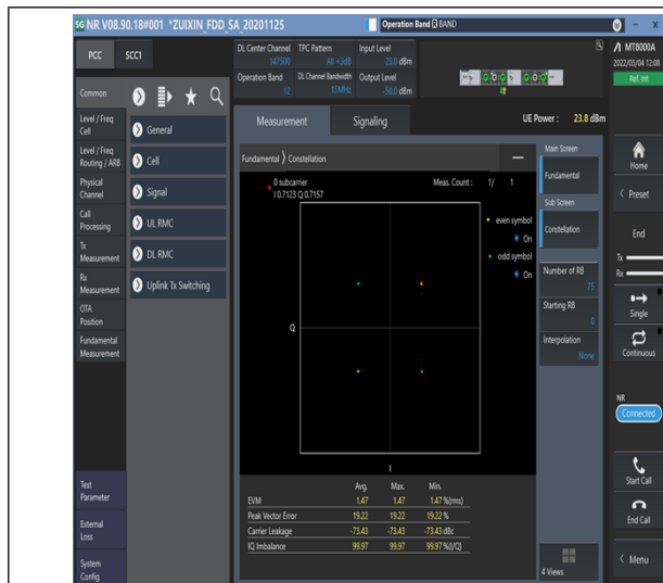
1-N12-PC3-15-15-M-1-DFT-PI2BPSK-Outter_Full-75@0-Ant1-see graph-PASS
