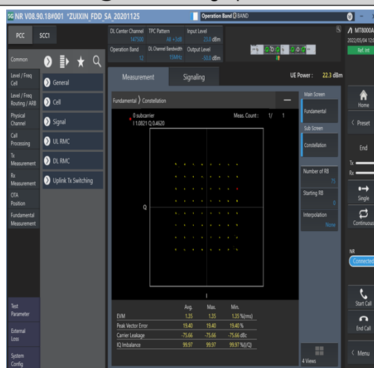
1-N12-PC3-15-15-M-4-DFT-64QAM-Outter_Full-75@0-Ant1-see graph-PASS
