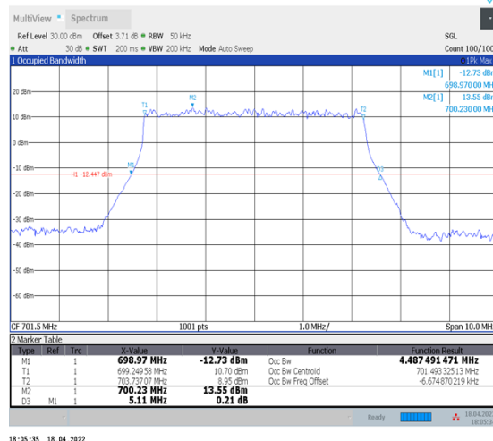
1-N12--15-5-L-2-DFT-PI2BPSK-Outer_Full-25@0-Ant1-4.487-5.110-≤5-PASS
