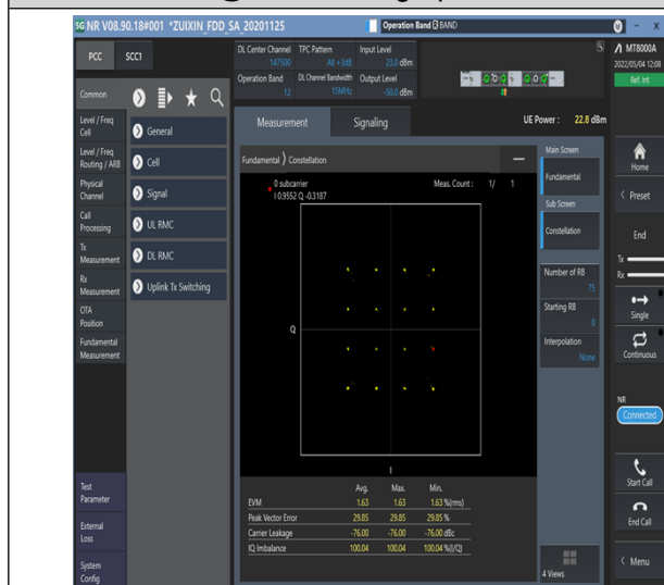
1-N12-PC3-15-15-M-3-DFT-16QAM-Outter_Full-75@0-Ant1-see graph-PASS
