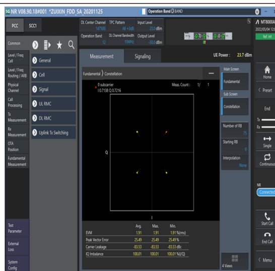
1-N12-PC3-15-15-M-2-DFT-QPSK-Outter_Full-75@0-Ant1-see graph-PASS
