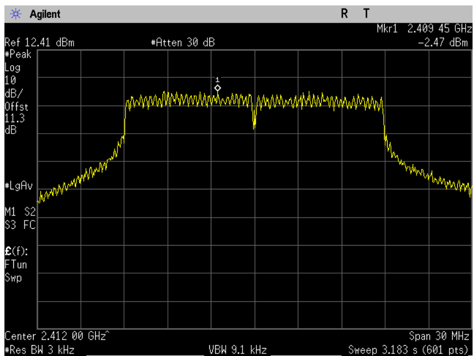
WIFI_Low Ch_2412MHz_20MHz BW_n-mode_Spectral Density_Port 1_
