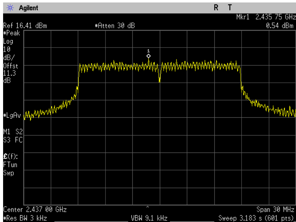
WIFI_Mid Ch_2437MHz_20MHz BW_n-mode_Spectral Density_Port 1_
