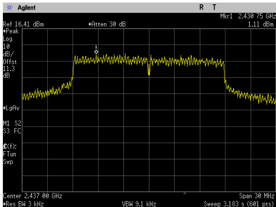
WIFI_Mid Ch_2437MHz_20MHz BW_n-mode_Spectral Density_Port 2_
