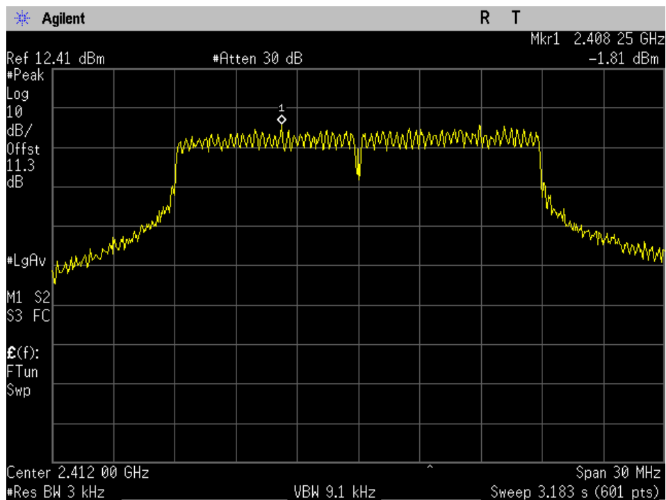
WIFI_Low Ch_2412MHz_20MHz BW_n-mode_Spectral Density_Port 2_
