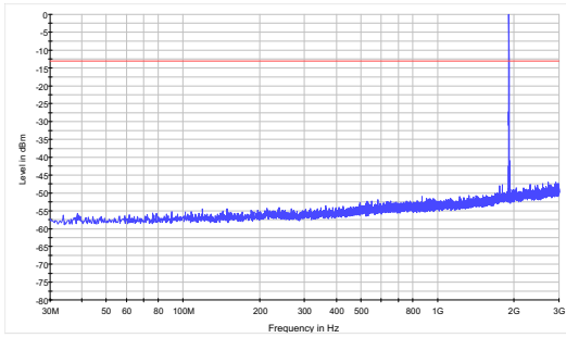
GSM 1900 CH-High 30MHz~3GHz
