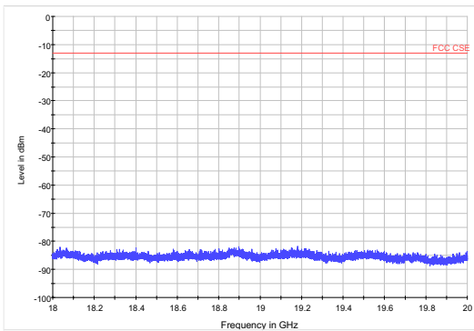
GSM 1900 CH-High 18GHz~20GHz
