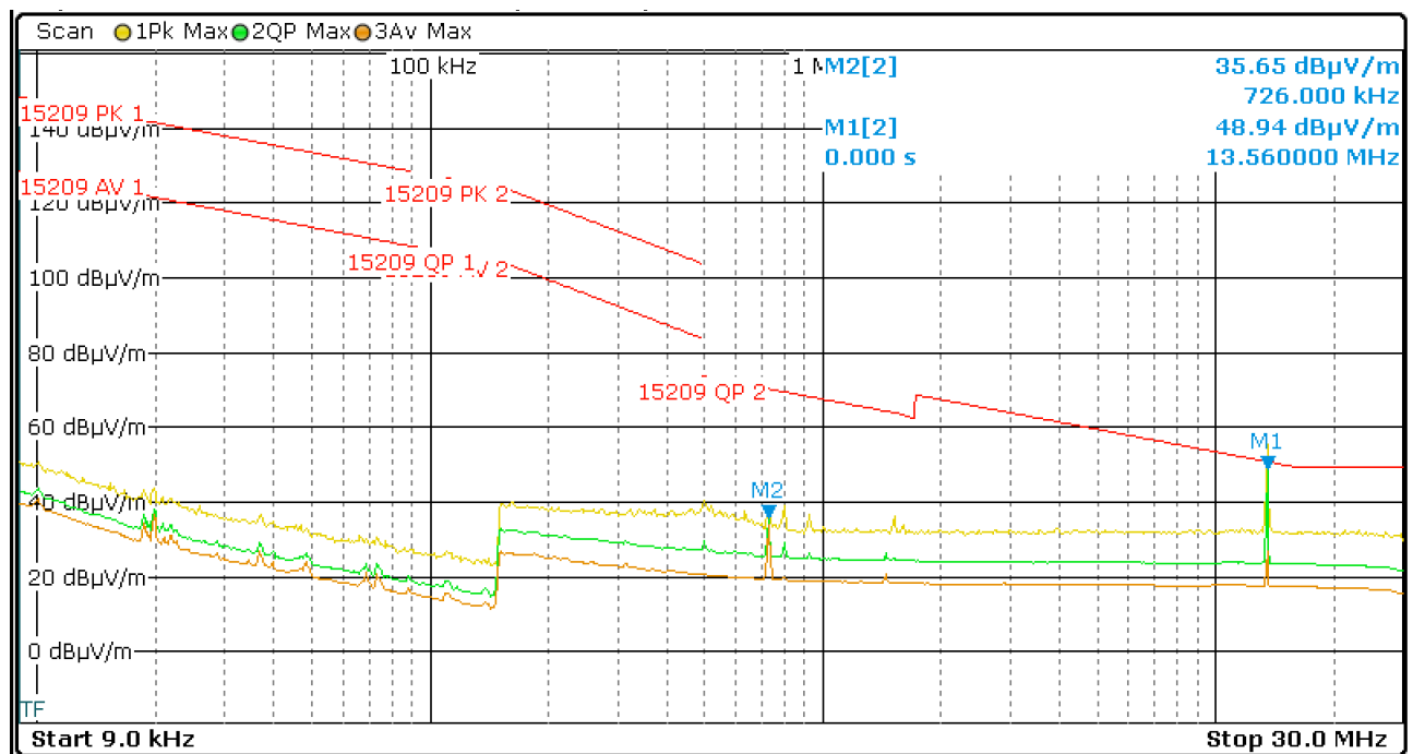
Figure 11: Chart of radiated emissions test below 30 MHz, EUT position Y, antenna polarization in line, without tag
