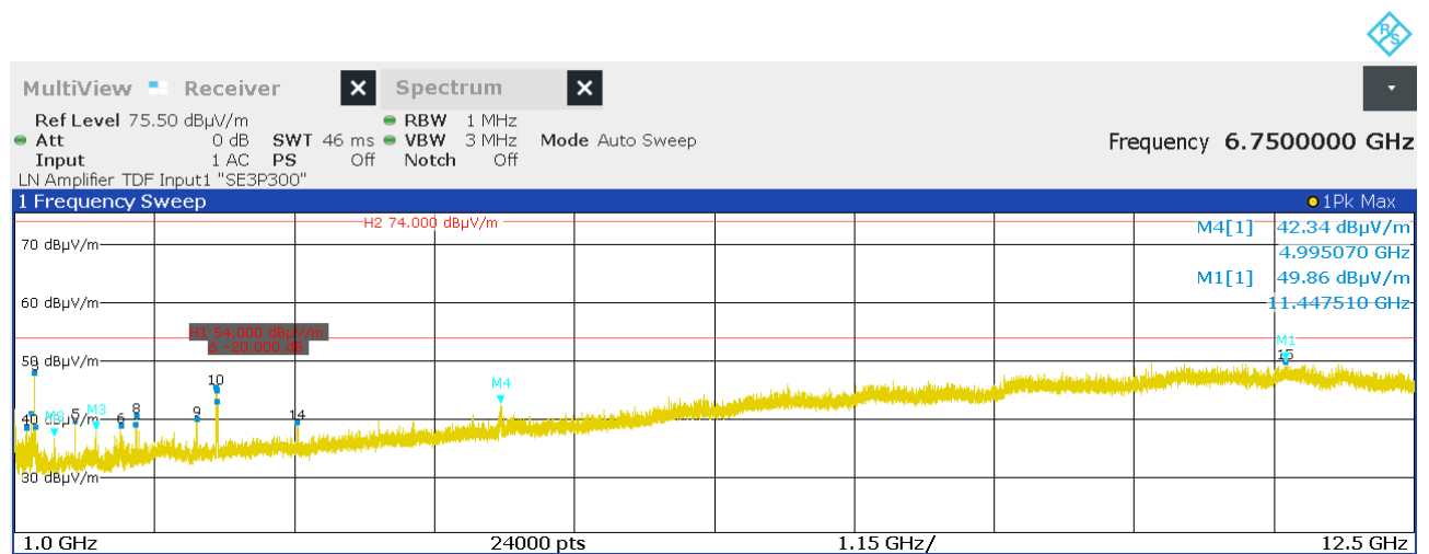
Figure 13: Chart of emissions test from 1 GHz to 12.5 GHz, EUT position Y, antenna polarization vertical, with tag
