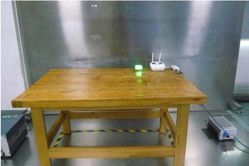
Conducted Emission – Front View
