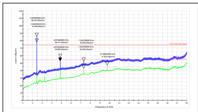
Channel Frequency: 2437MHz Polarization: Horizontal
