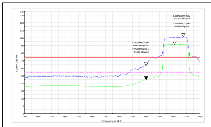
Channel Frequency: 2412MHz Polarization: Horizontal
