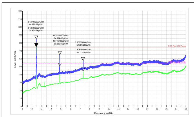
Channel Frequency: 2437MHz Polarization: Horizontal
