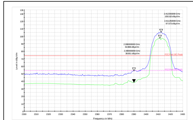
Channel Frequency: 2412MHz Polarization: Horizontal
