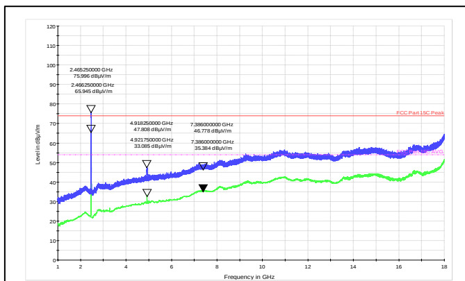
Channel Frequency: 2462MHz Polarization: Horizontal
