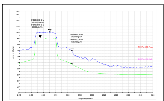
Channel Frequency: 2462MHz Polarization: Horizontal
