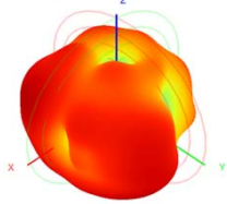
2500.0MHz H+V, Eff: 8.9%
