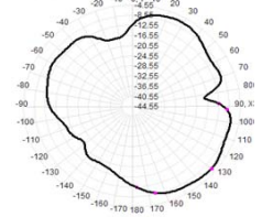
Total(H+V), Max=-6.96dBi, CrD=16.20
